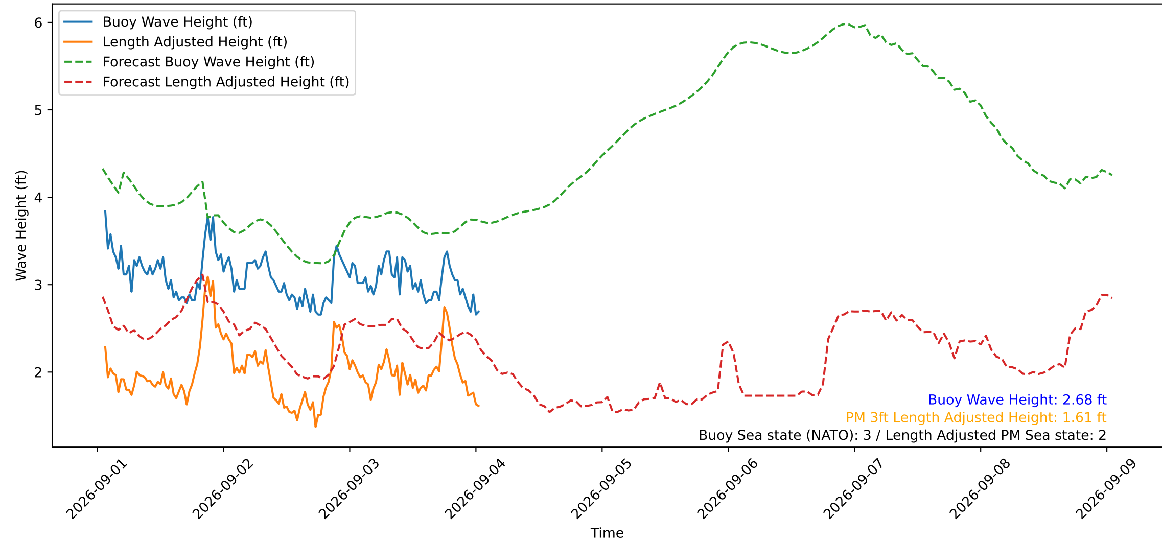
Wave Heights over Time for Green Beach at 2026-09-04 01:21:15
