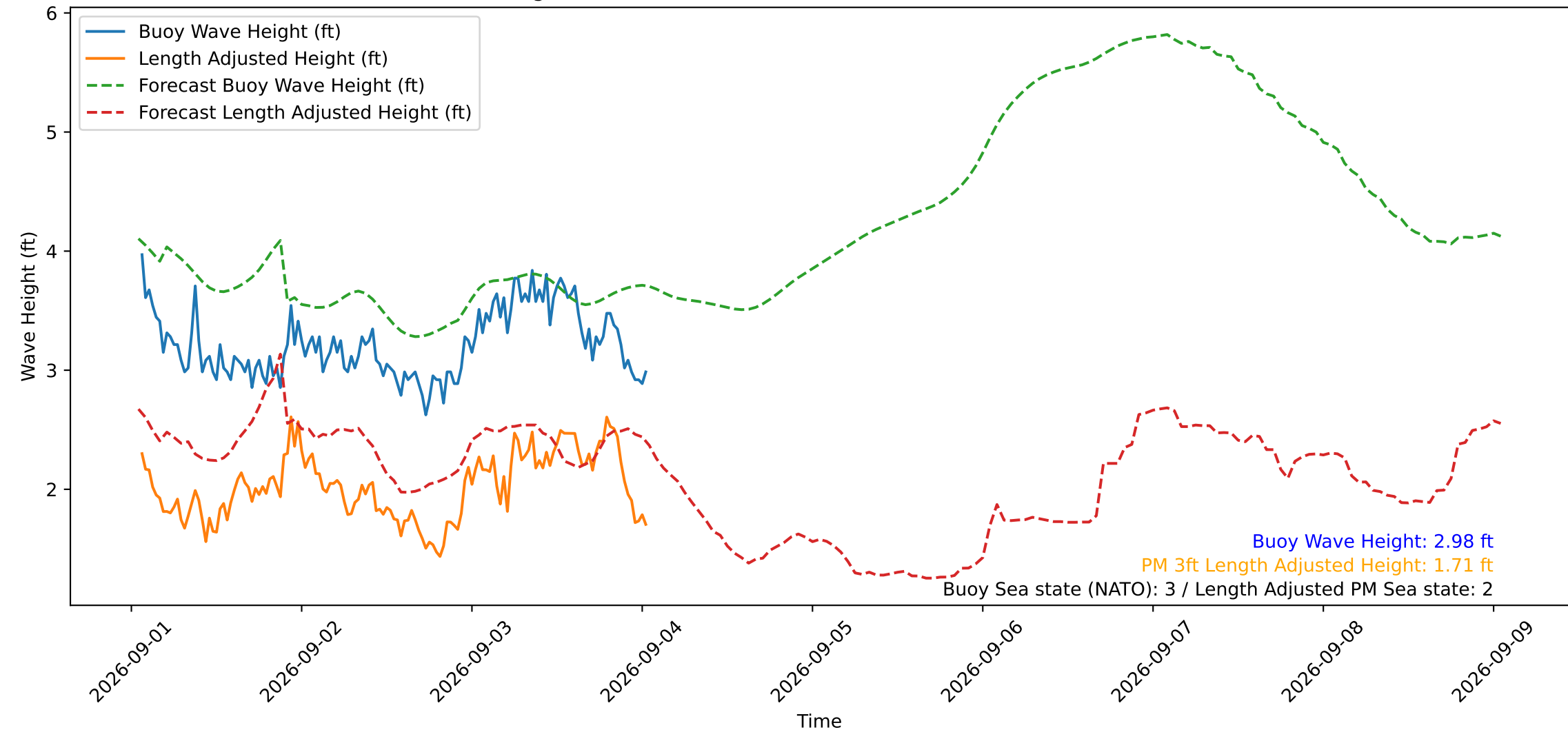
Wave Heights over Time for Oceanside Harbor at 2026-09-04 01:20:29
