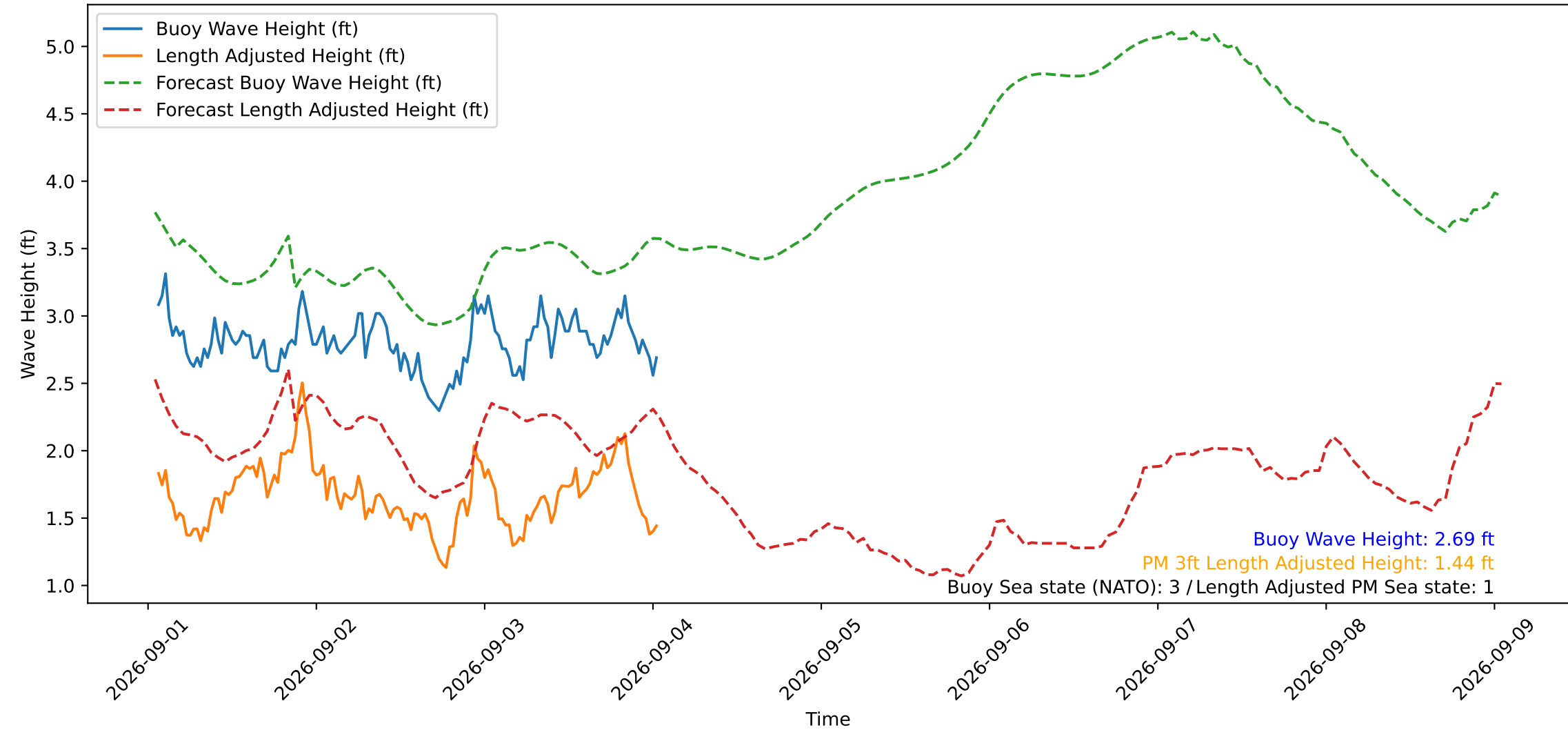
Wave Heights over Time for Red Beach at 2026-09-04 01:20:51
