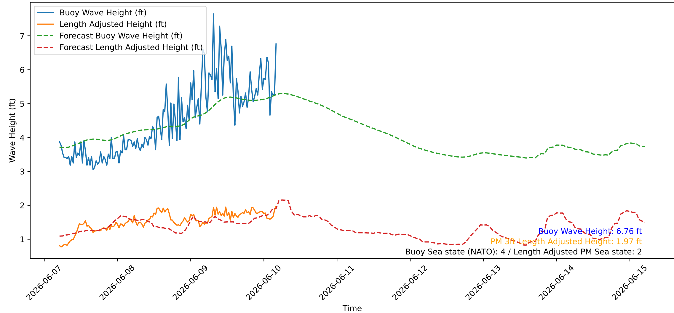
Wave Heights over Time for Red Beach at 2026-06-10 04:40:46
