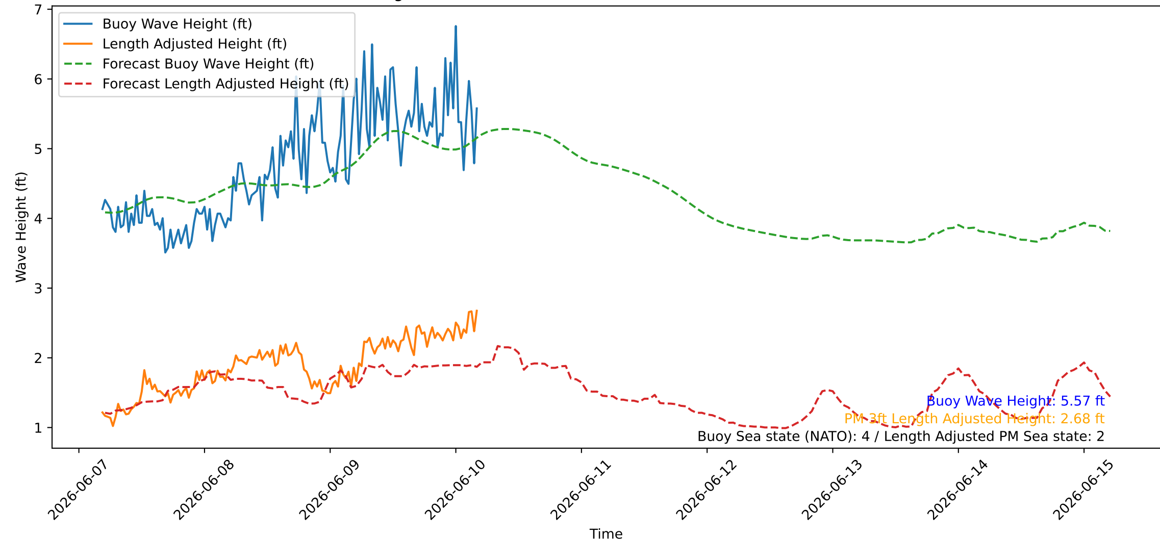
Wave Heights over Time for Oceanside Harbor at 2026-06-10 04:40:26
