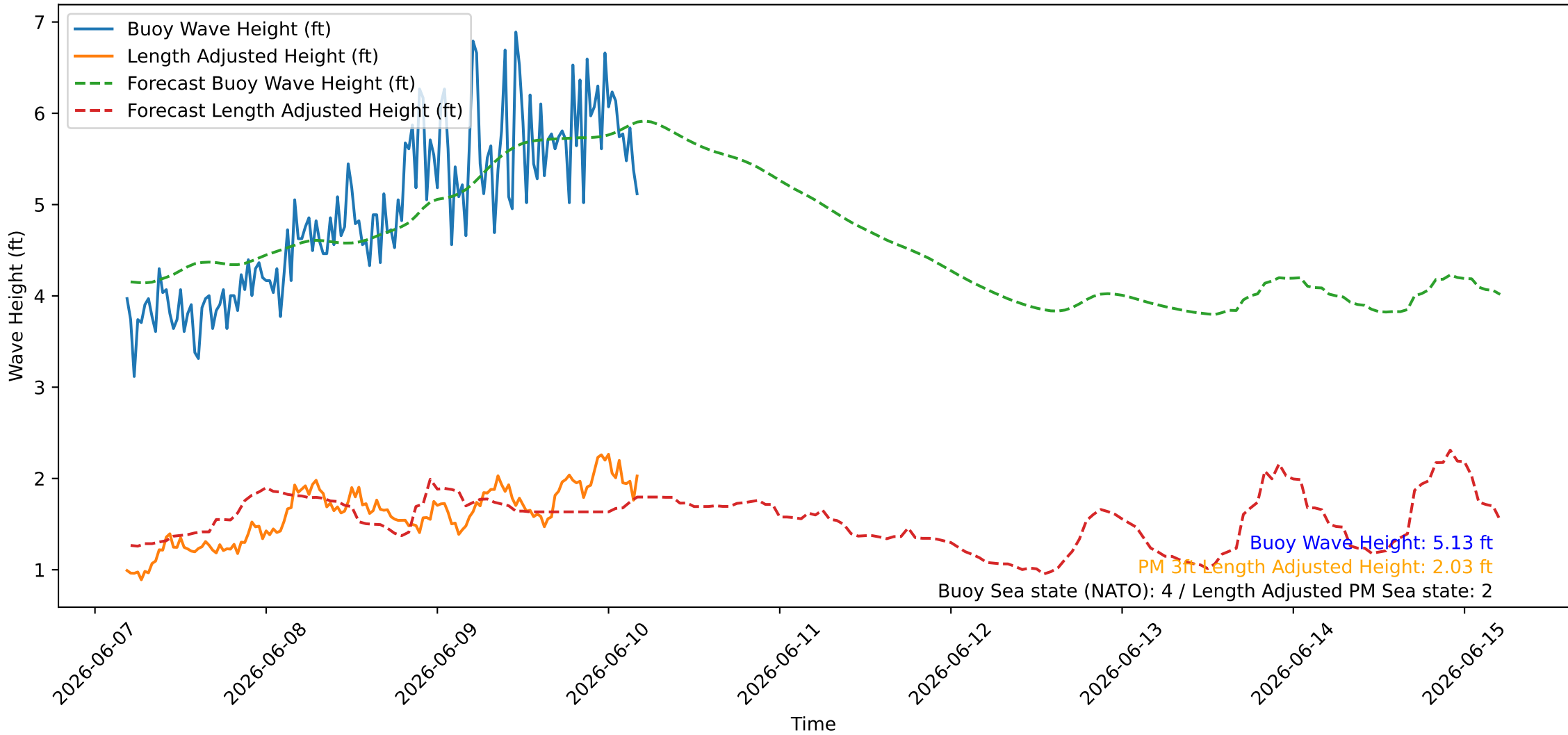
Wave Heights over Time for Green Beach at 2026-06-10 04:41:10
