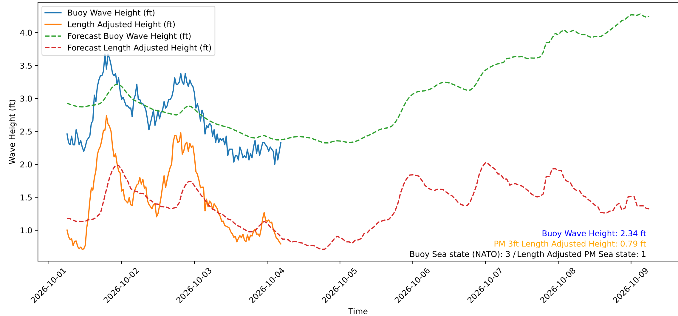
Wave Heights over Time for Green Beach at 2026-10-04 05:31:12
