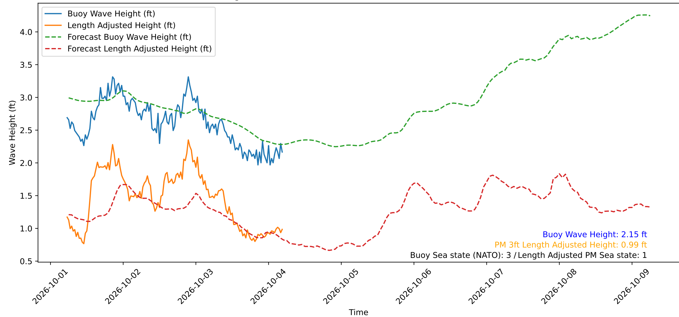
Wave Heights over Time for Oceanside Harbor at 2026-10-04 05:30:30
