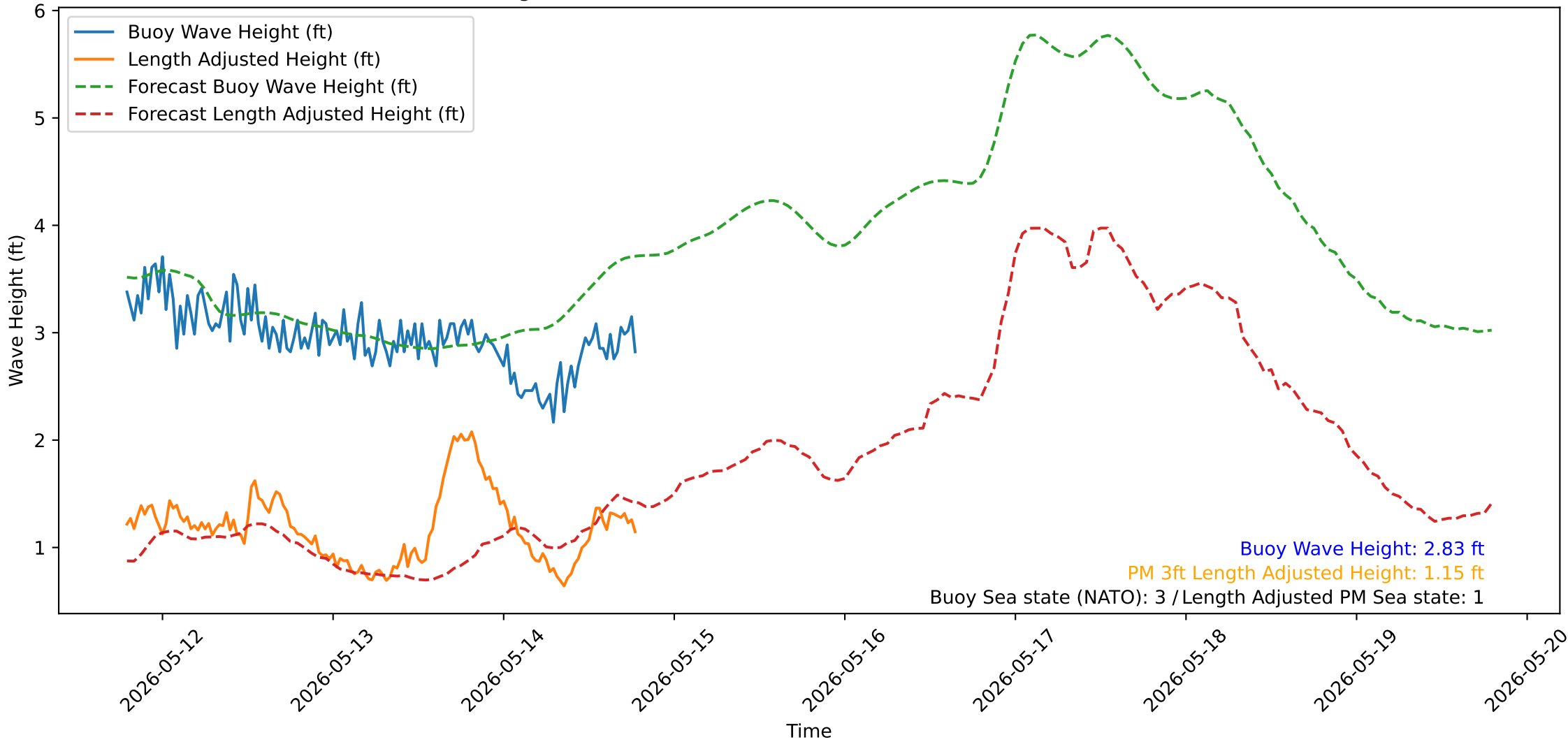
Wave Heights over Time for Oceanside Harbor at 2026-05-14 19:10:32
