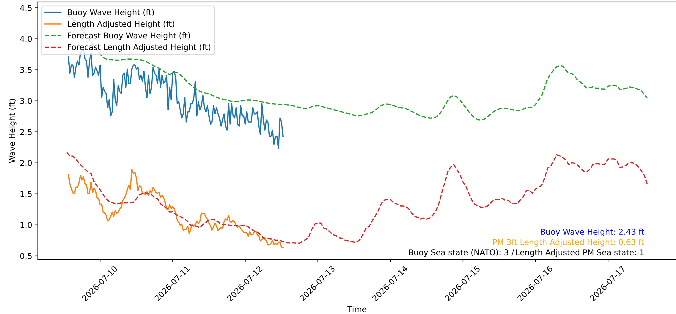
Wave Heights over Time for Green Beach at 2026-07-12 13:21:11
