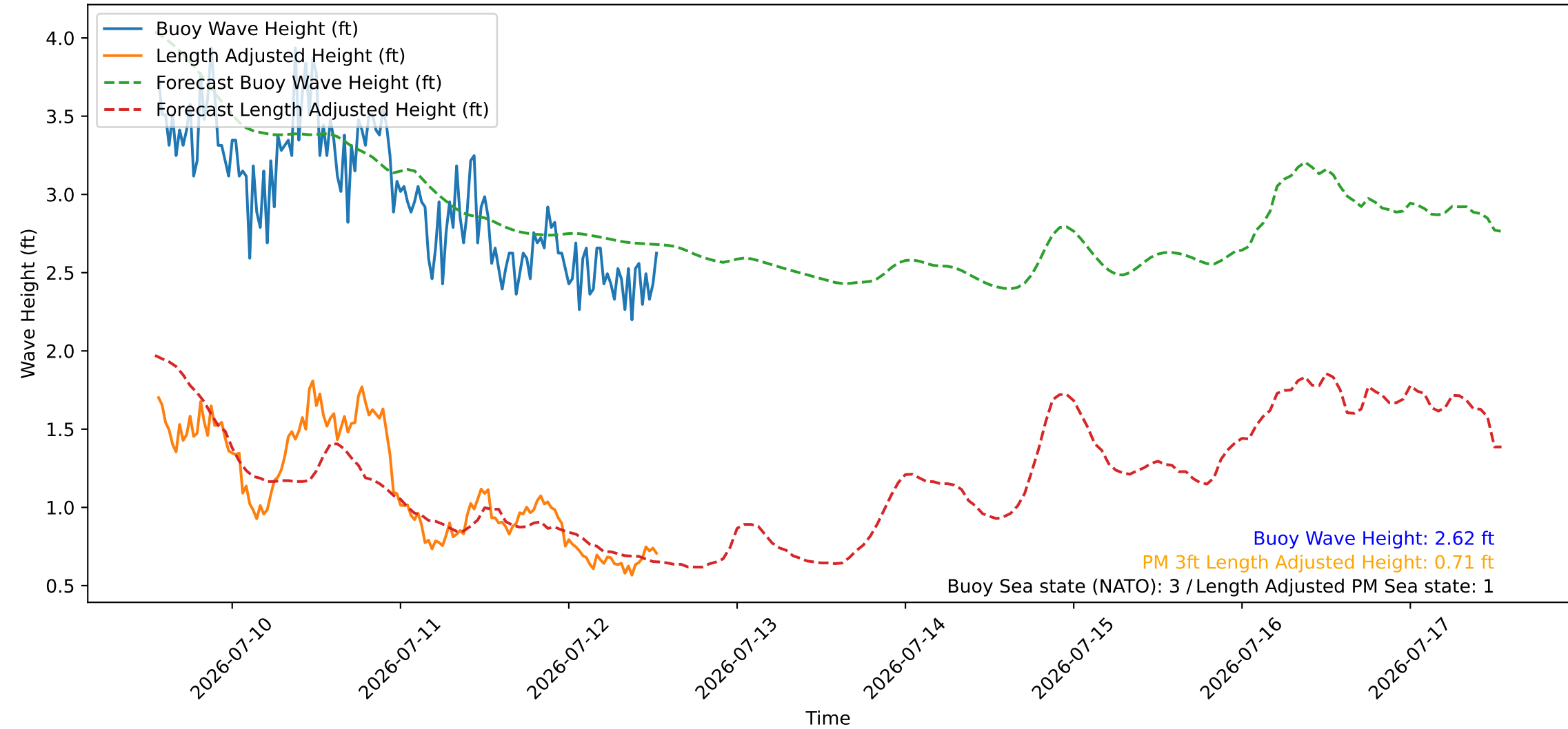
Wave Heights over Time for Red Beach at 2026-07-12 13:20:48
