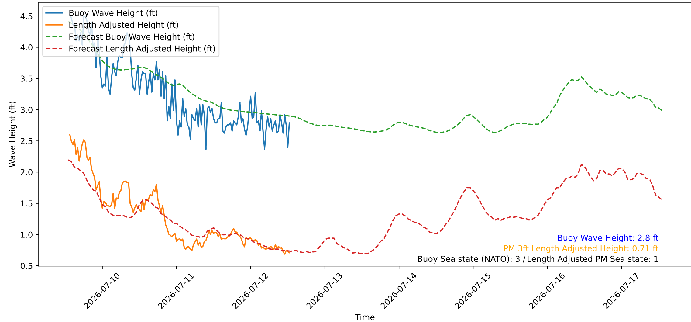
Wave Heights over Time for Oceanside Harbor at 2026-07-12 13:20:27
