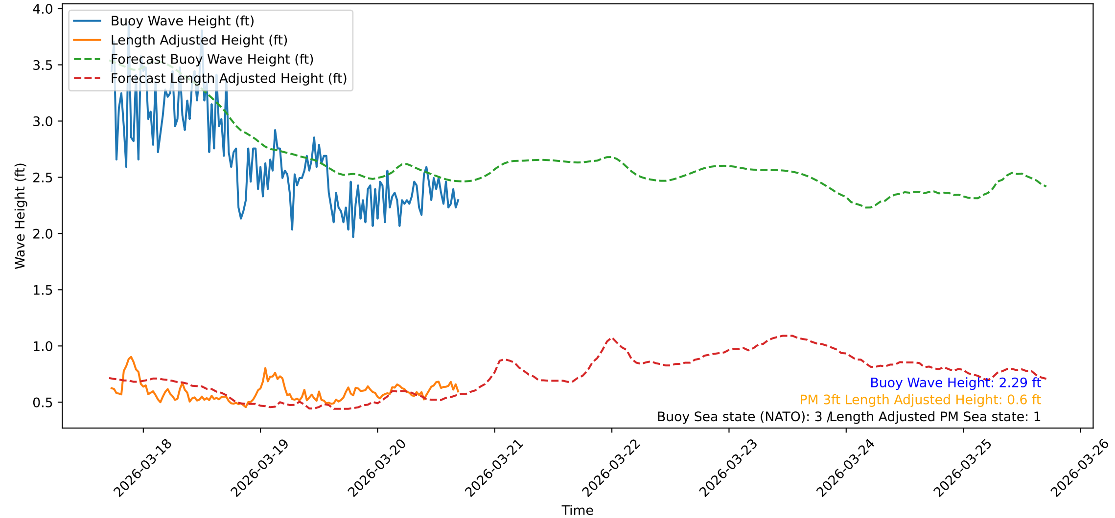
Wave Heights over Time for Oceanside Harbor at 2026-03-20 17:20:32
