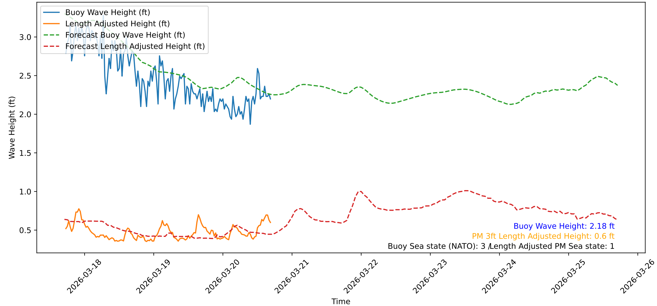
Wave Heights over Time for Red Beach at 2026-03-20 17:20:48
