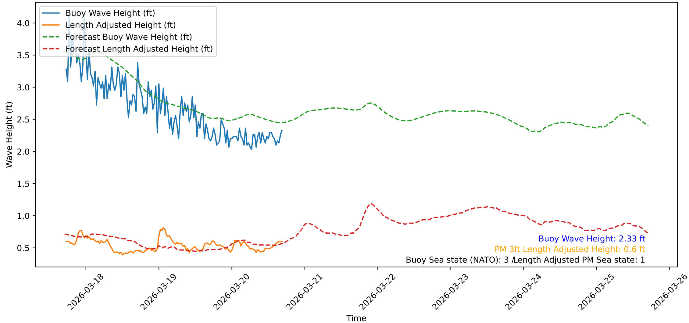
Wave Heights over Time for Green Beach at 2026-03-20 17:21:11
