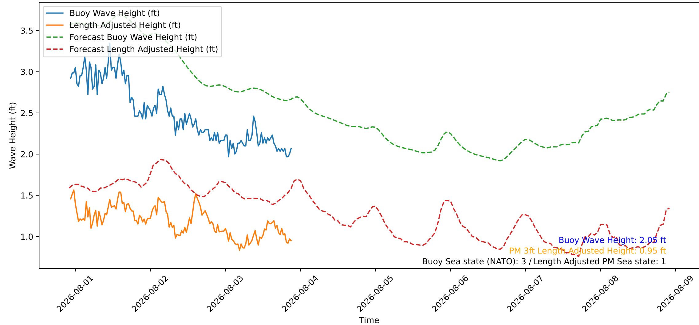
Wave Heights over Time for Red Beach at 2026-08-03 22:00:45
