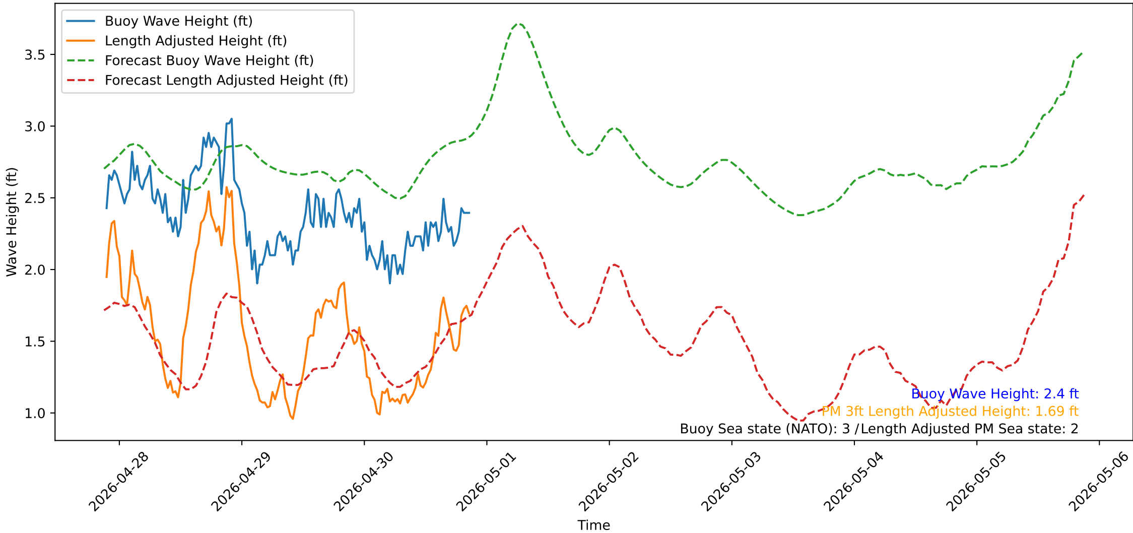
Wave Heights over Time for Oceanside Harbor at 2026-04-30 21:20:32
