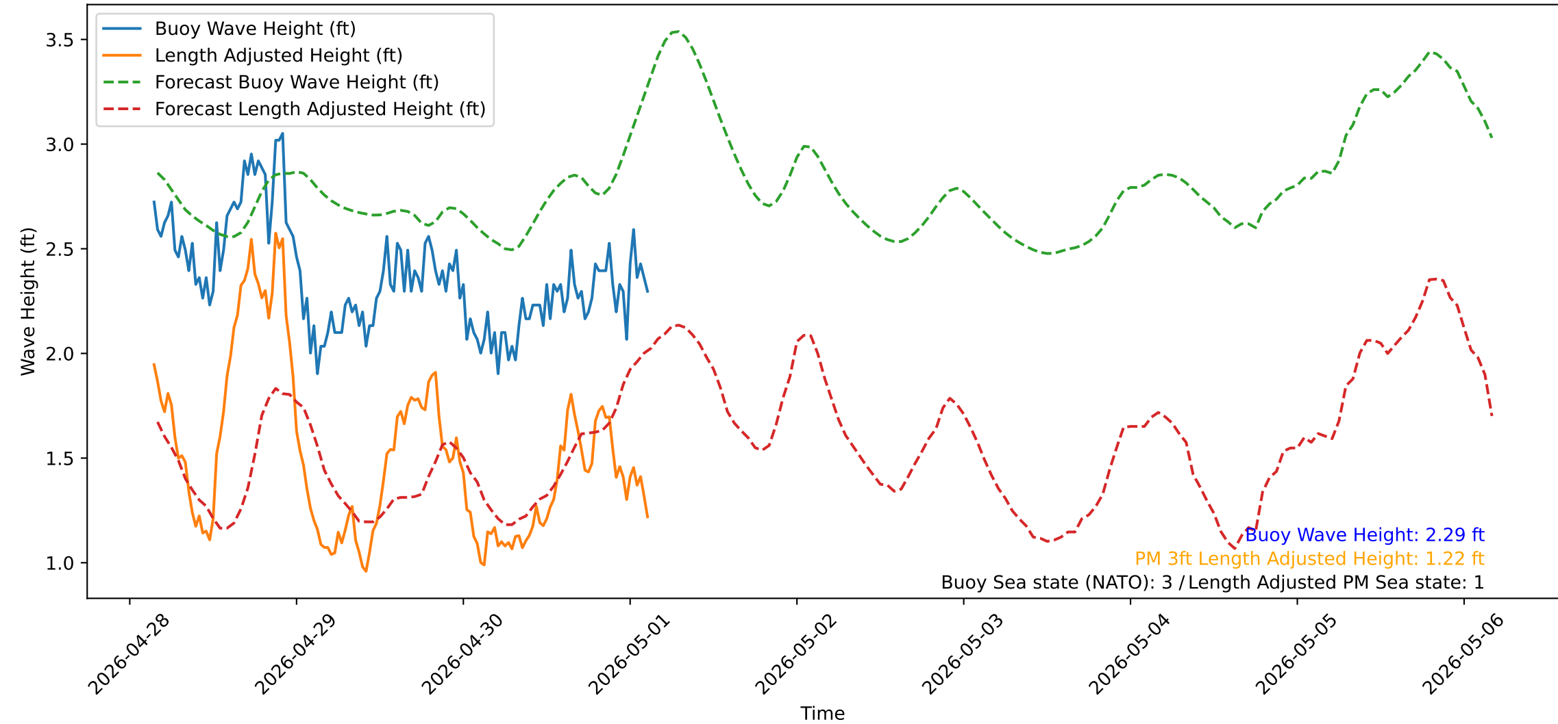
Wave Heights over Time for Oceanside Harbor at 2026-05-01 03:40:31
