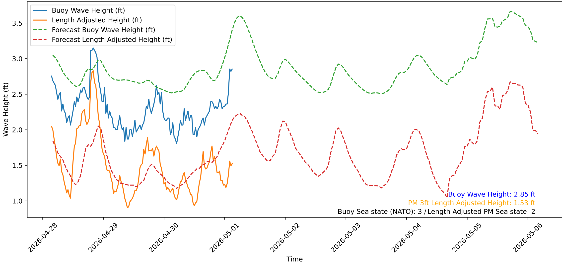
Wave Heights over Time for Green Beach at 2026-05-01 03:41:12
