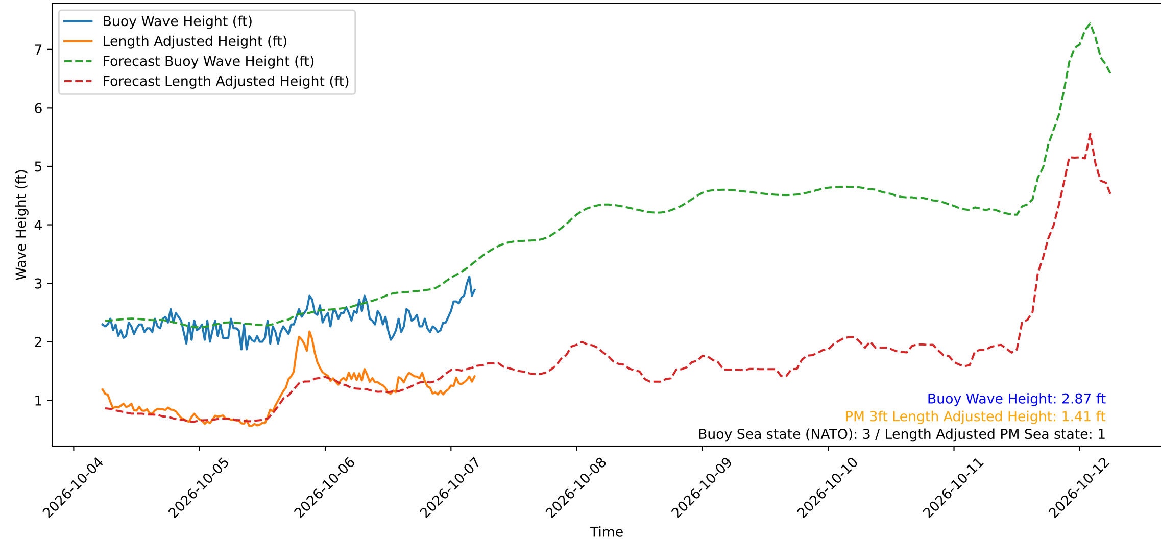
Wave Heights over Time for Oceanside Harbor at 2026-10-07 05:30:29
