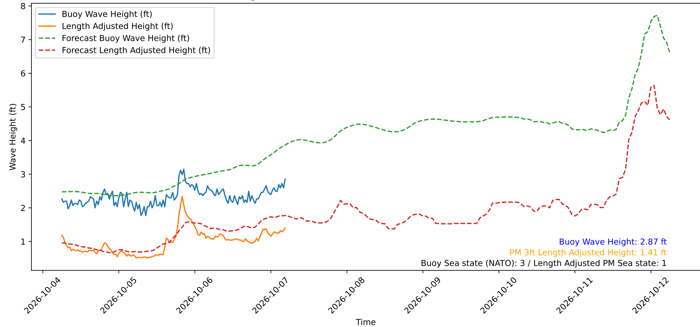
Wave Heights over Time for Green Beach at 2026-10-07 05:31:11
