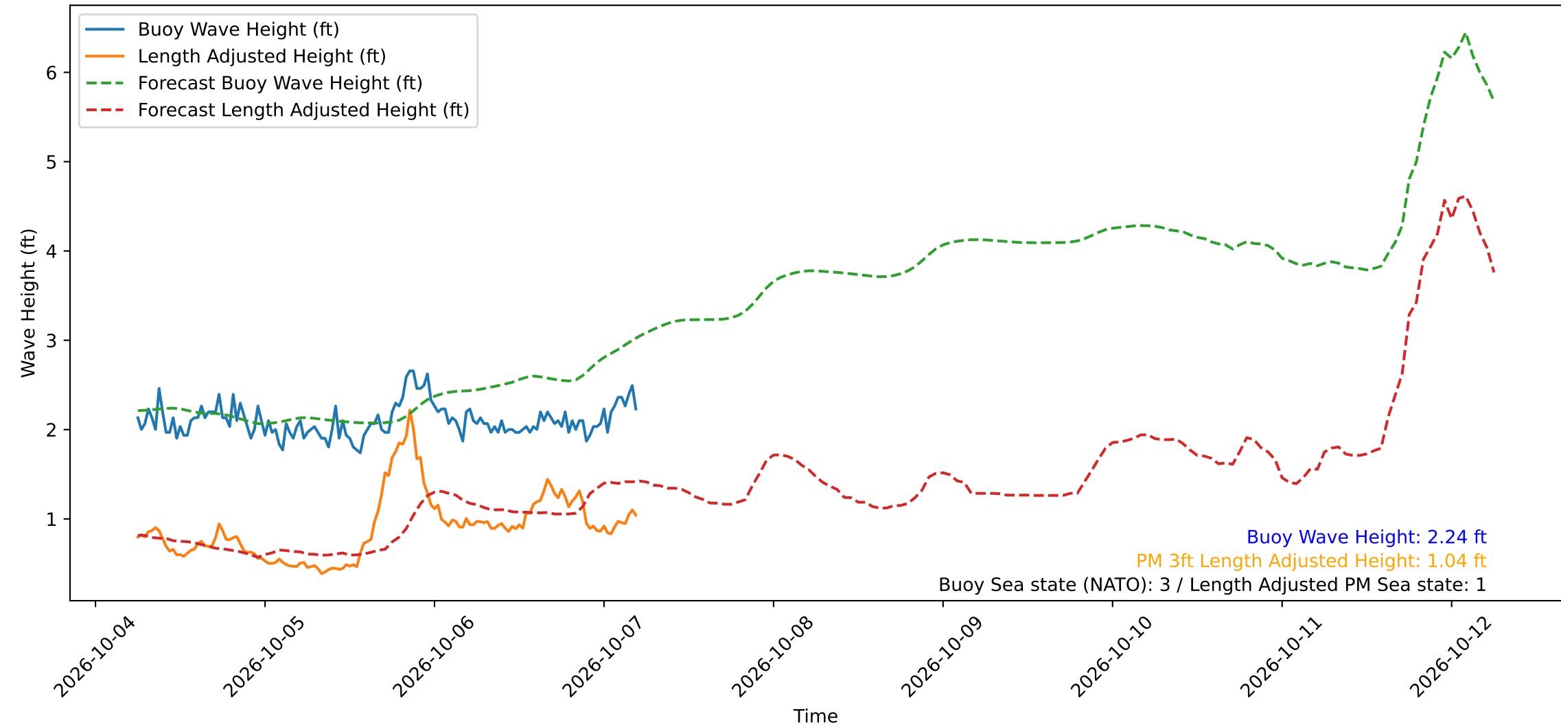
Wave Heights over Time for Red Beach at 2026-10-07 05:30:49
