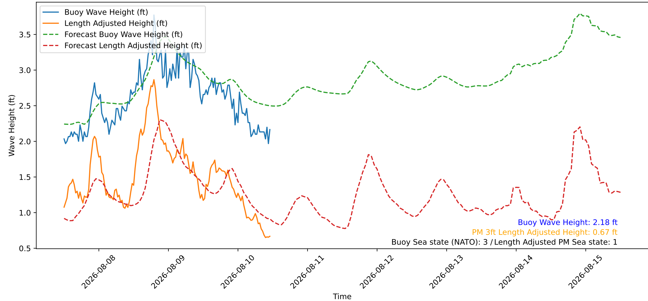
Wave Heights over Time for Green Beach at 2026-08-10 12:01:09
