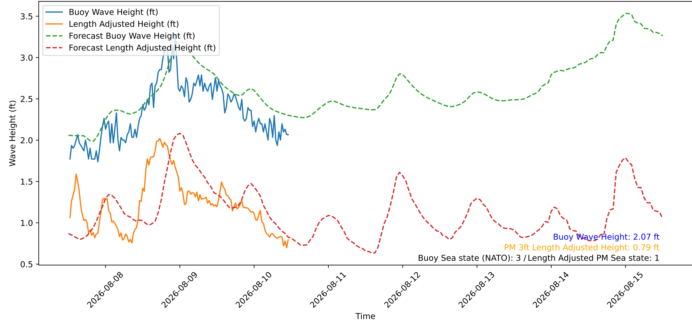
Wave Heights over Time for Red Beach at 2026-08-10 12:00:46
