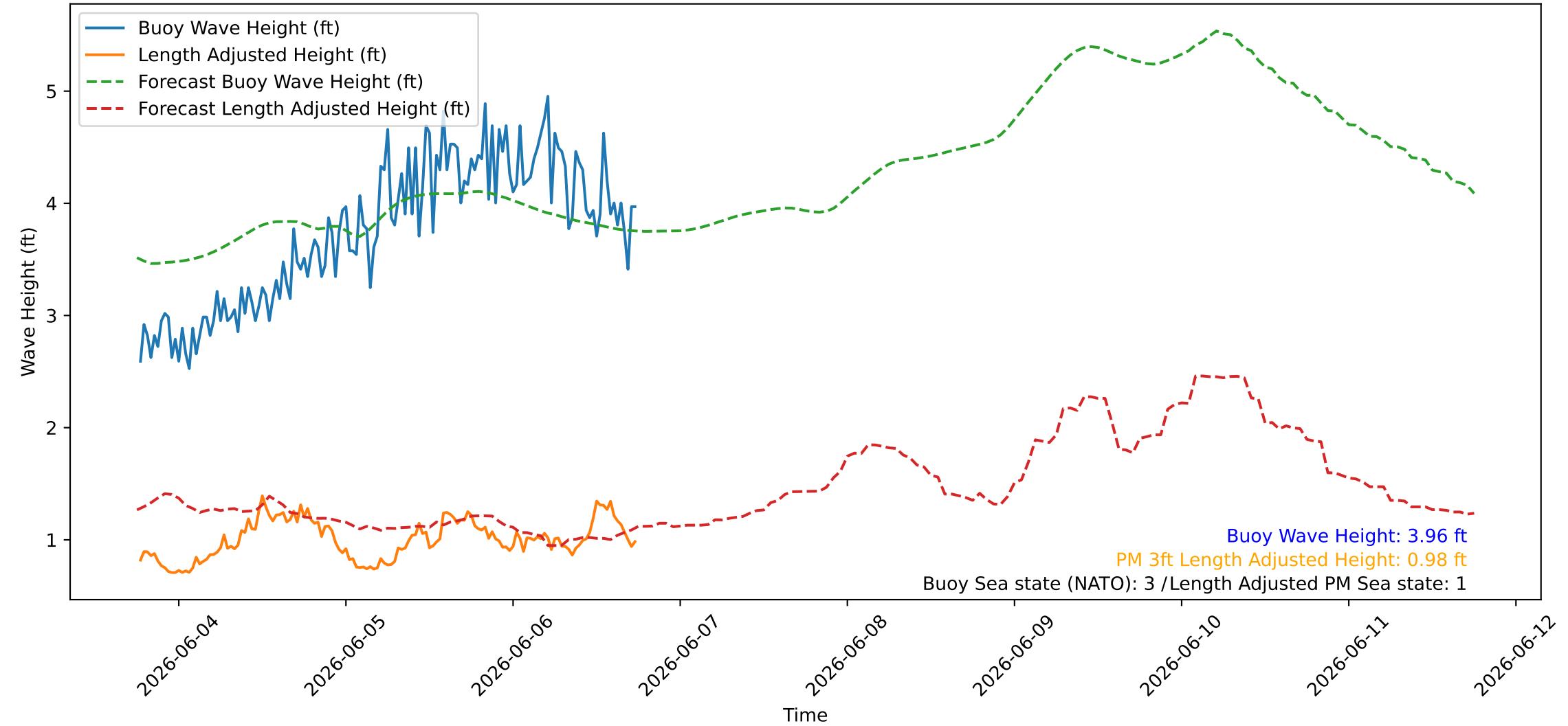
Wave Heights over Time for Red Beach at 2026-06-06 18:20:46
