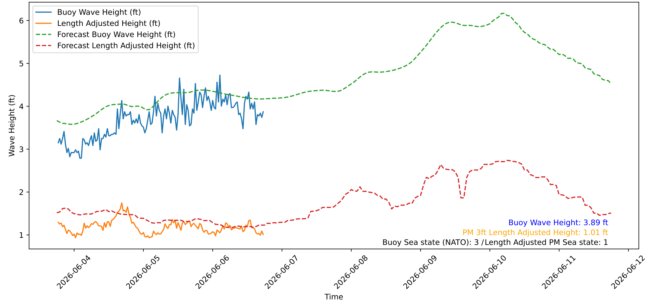
Wave Heights over Time for Green Beach at 2026-06-06 18:21:09
