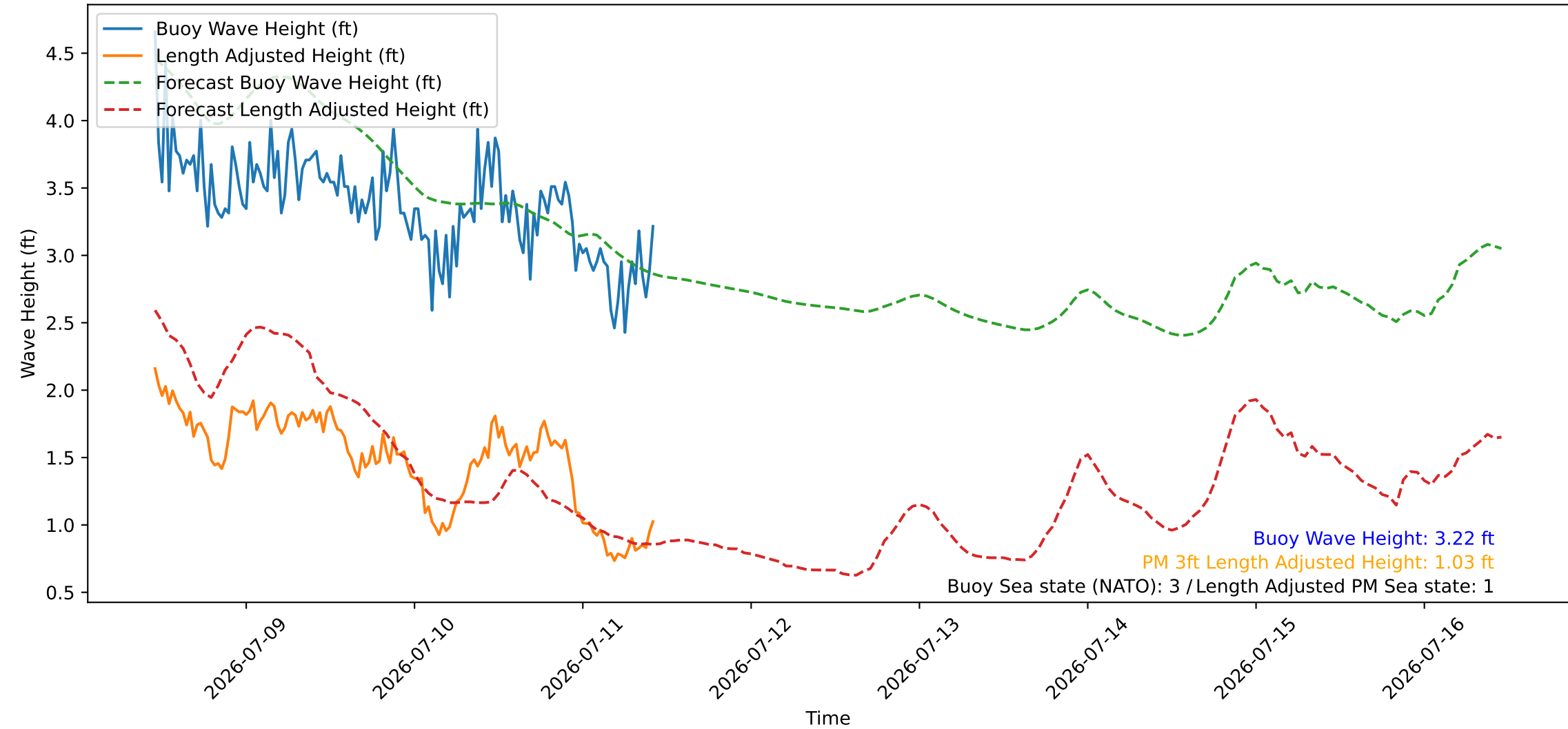
Wave Heights over Time for Red Beach at 2026-07-11 10:40:47
