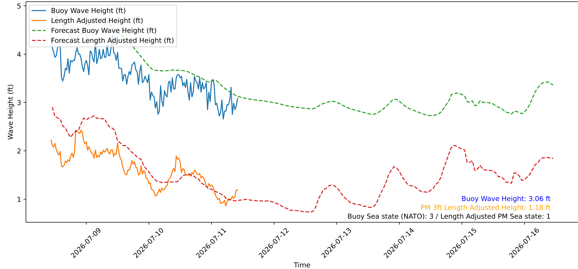
Wave Heights over Time for Green Beach at 2026-07-11 10:41:09
