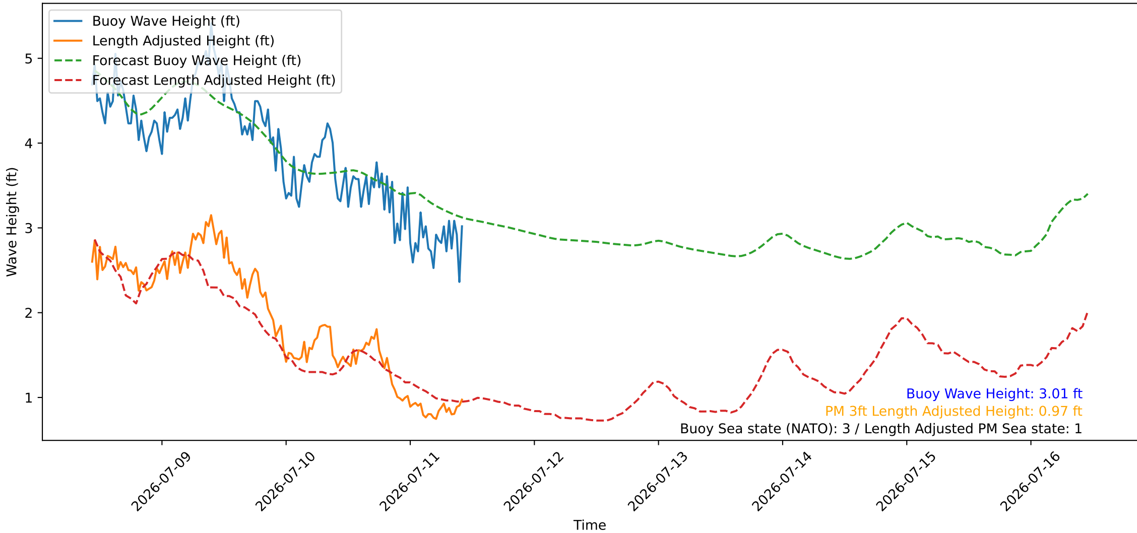
Wave Heights over Time for Oceanside Harbor at 2026-07-11 10:40:27
