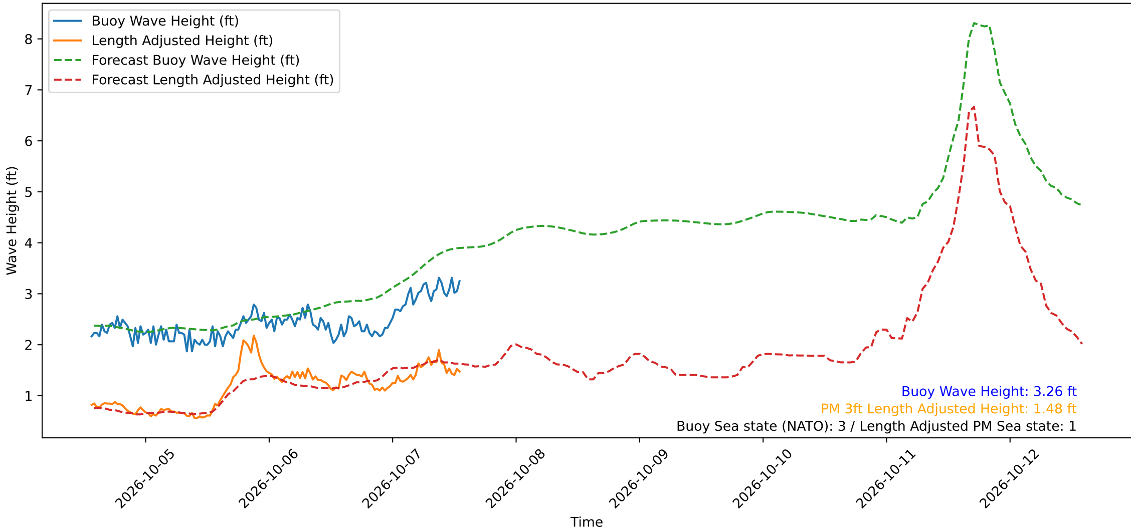
Wave Heights over Time for Oceanside Harbor at 2026-10-07 13:30:30
