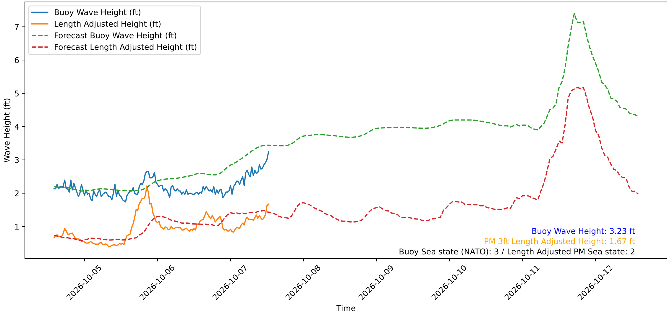
Wave Heights over Time for Red Beach at 2026-10-07 13:30:50
