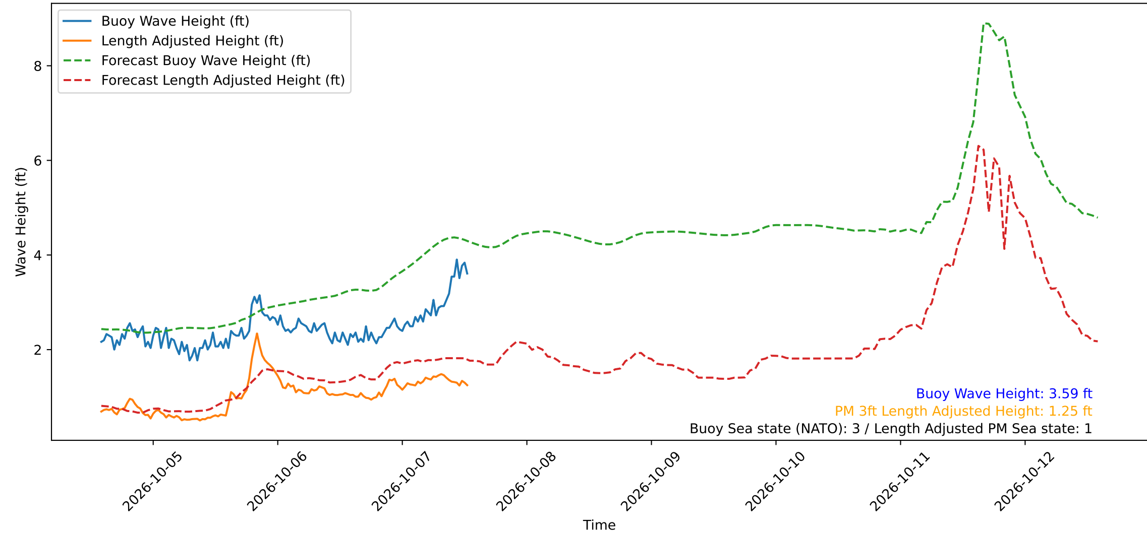
Wave Heights over Time for Green Beach at 2026-10-07 13:31:13
