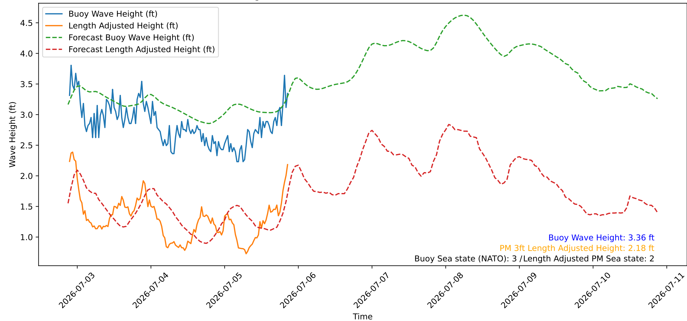
Wave Heights over Time for Red Beach at 2026-07-05 21:10:46
