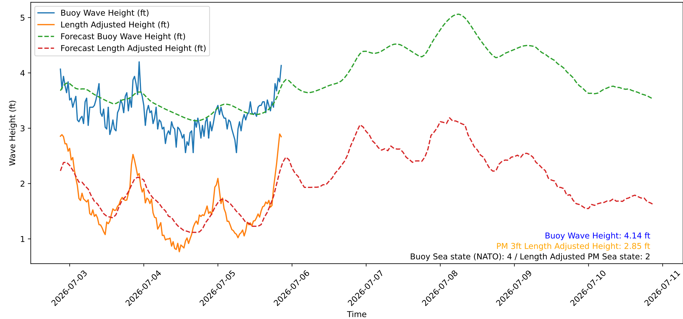
Wave Heights over Time for Green Beach at 2026-07-05 21:11:08
