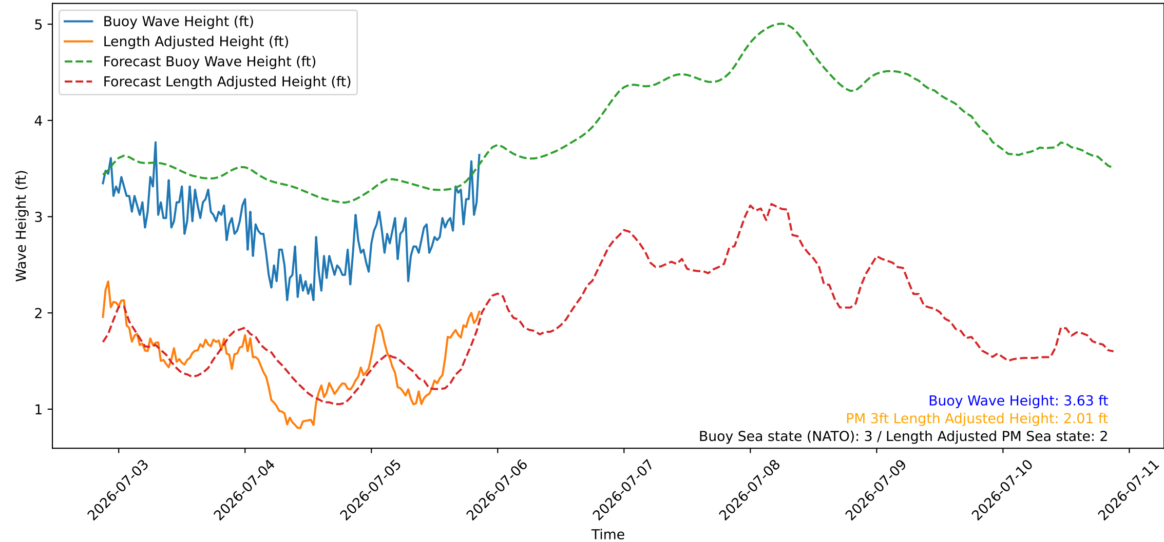
Wave Heights over Time for Oceanside Harbor at 2026-07-05 21:10:26
