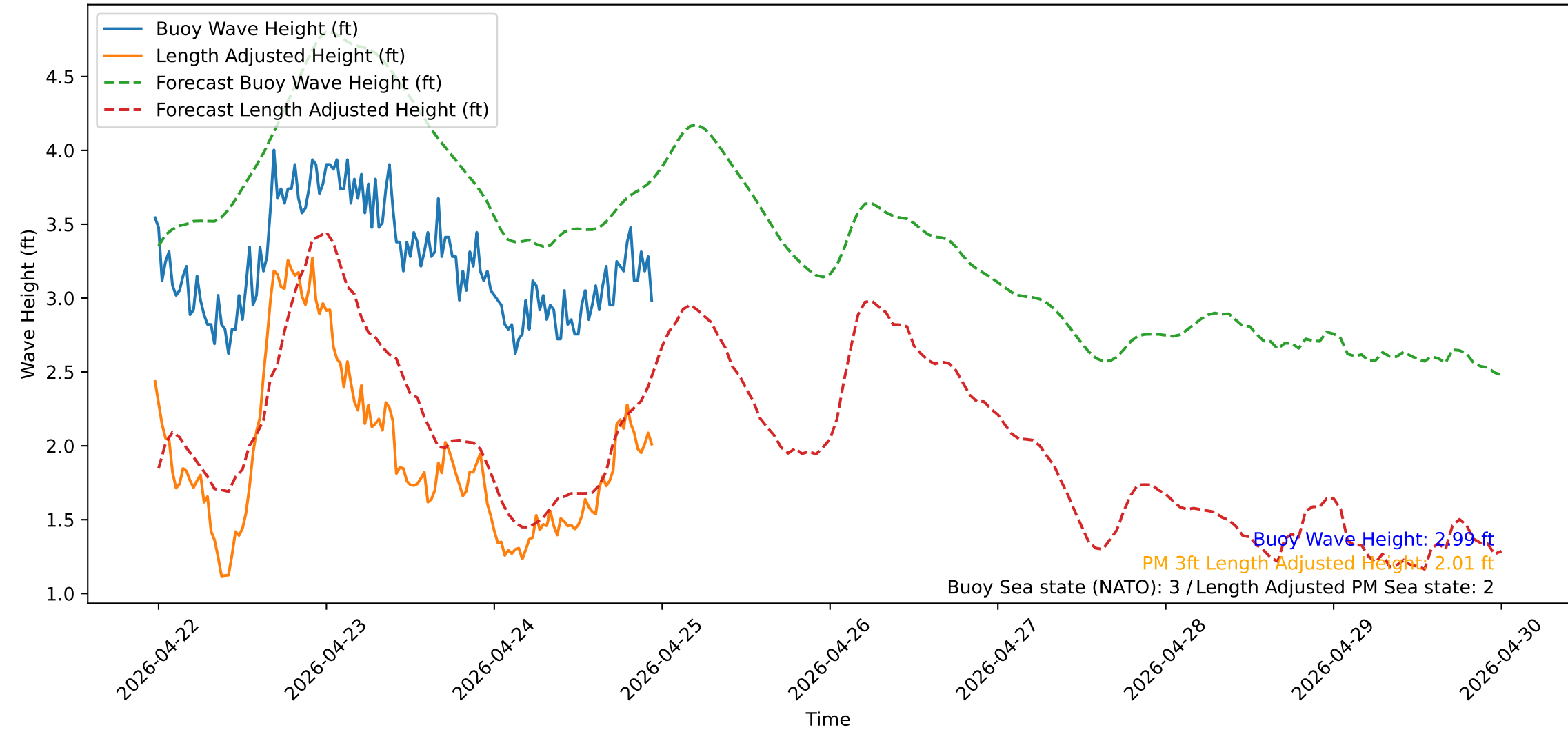
Wave Heights over Time for Green Beach at 2026-04-24 23:31:13
