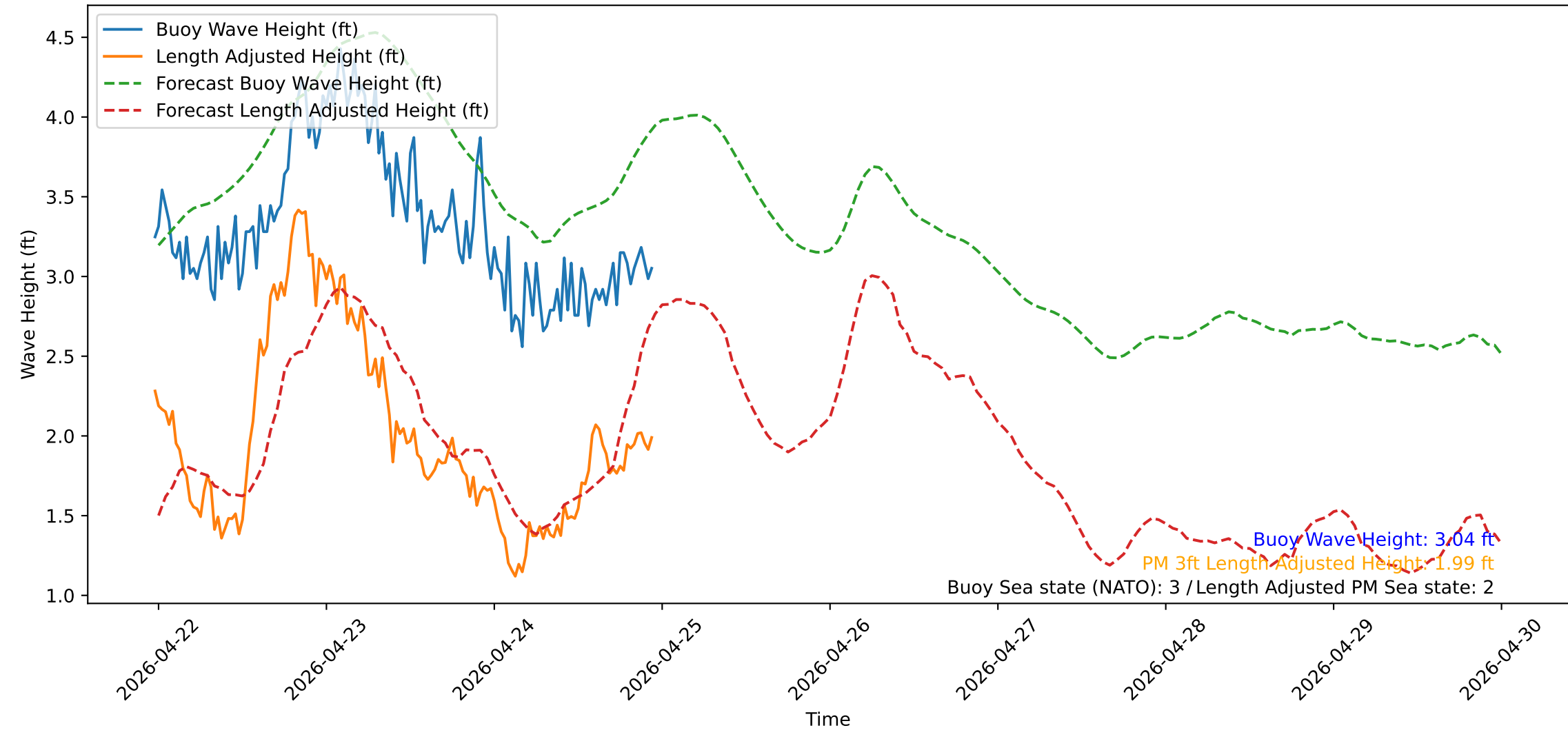
Wave Heights over Time for Oceanside Harbor at 2026-04-24 23:30:31
