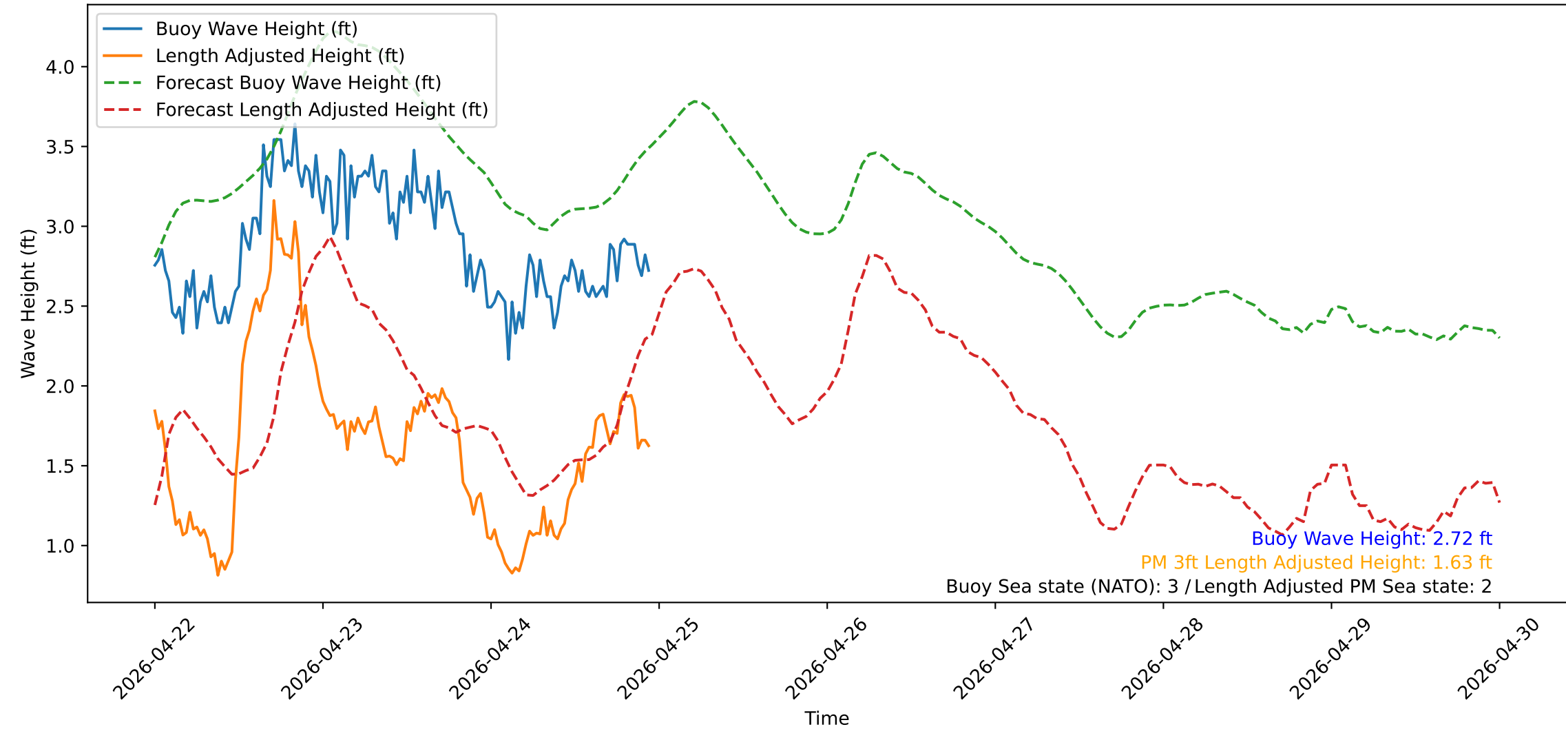
Wave Heights over Time for Red Beach at 2026-04-24 23:30:51
