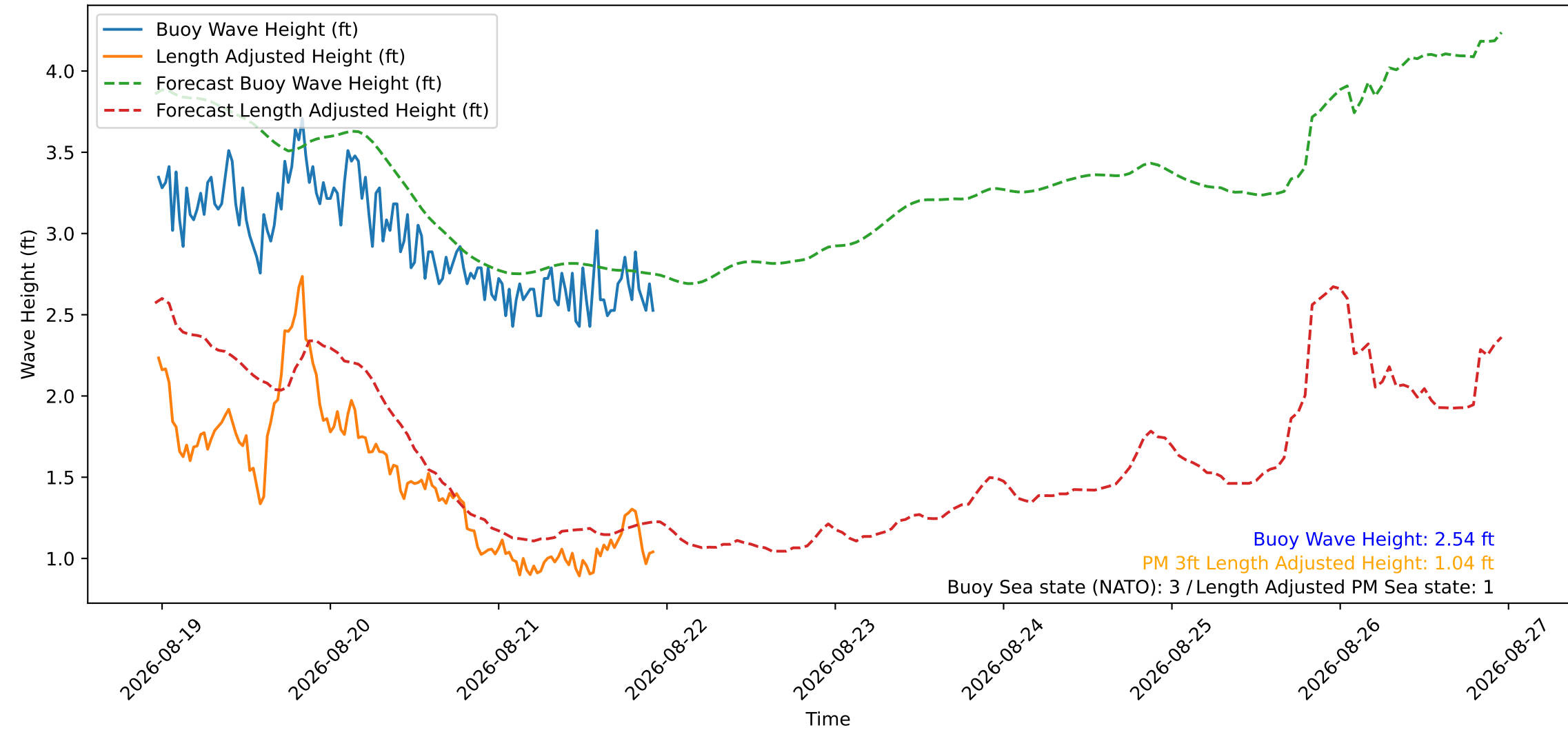
Wave Heights over Time for Green Beach at 2026-08-21 23:01:11
