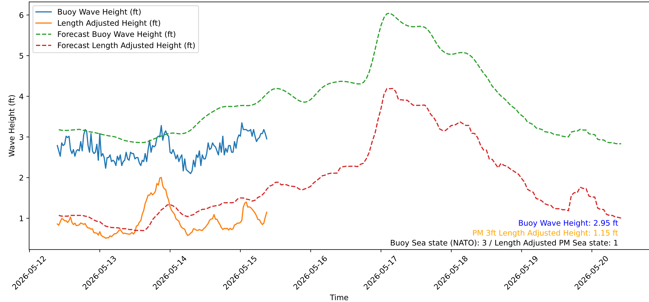
Wave Heights over Time for Green Beach at 2026-05-15 09:41:14
