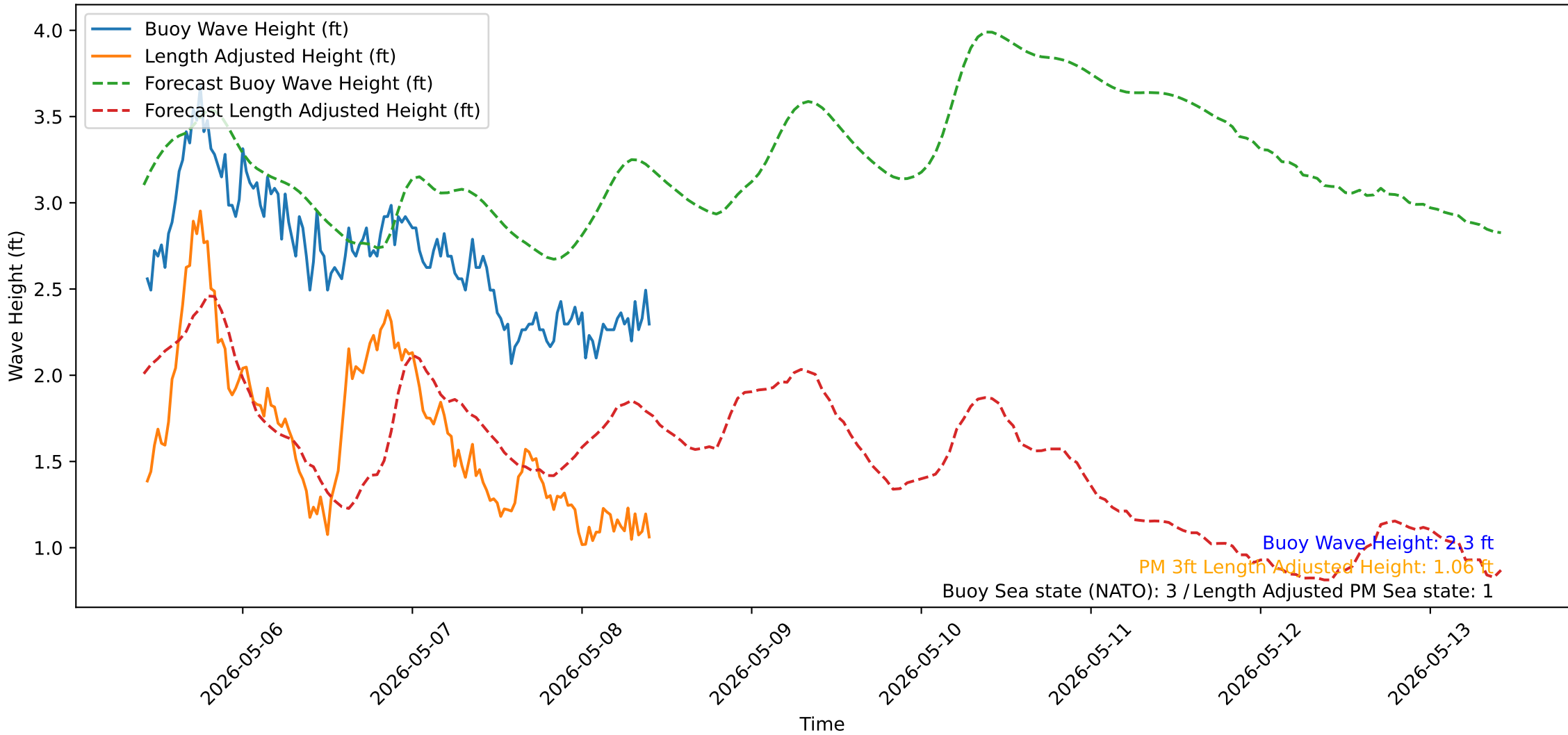
Wave Heights over Time for Green Beach at 2026-05-08 10:21:15
