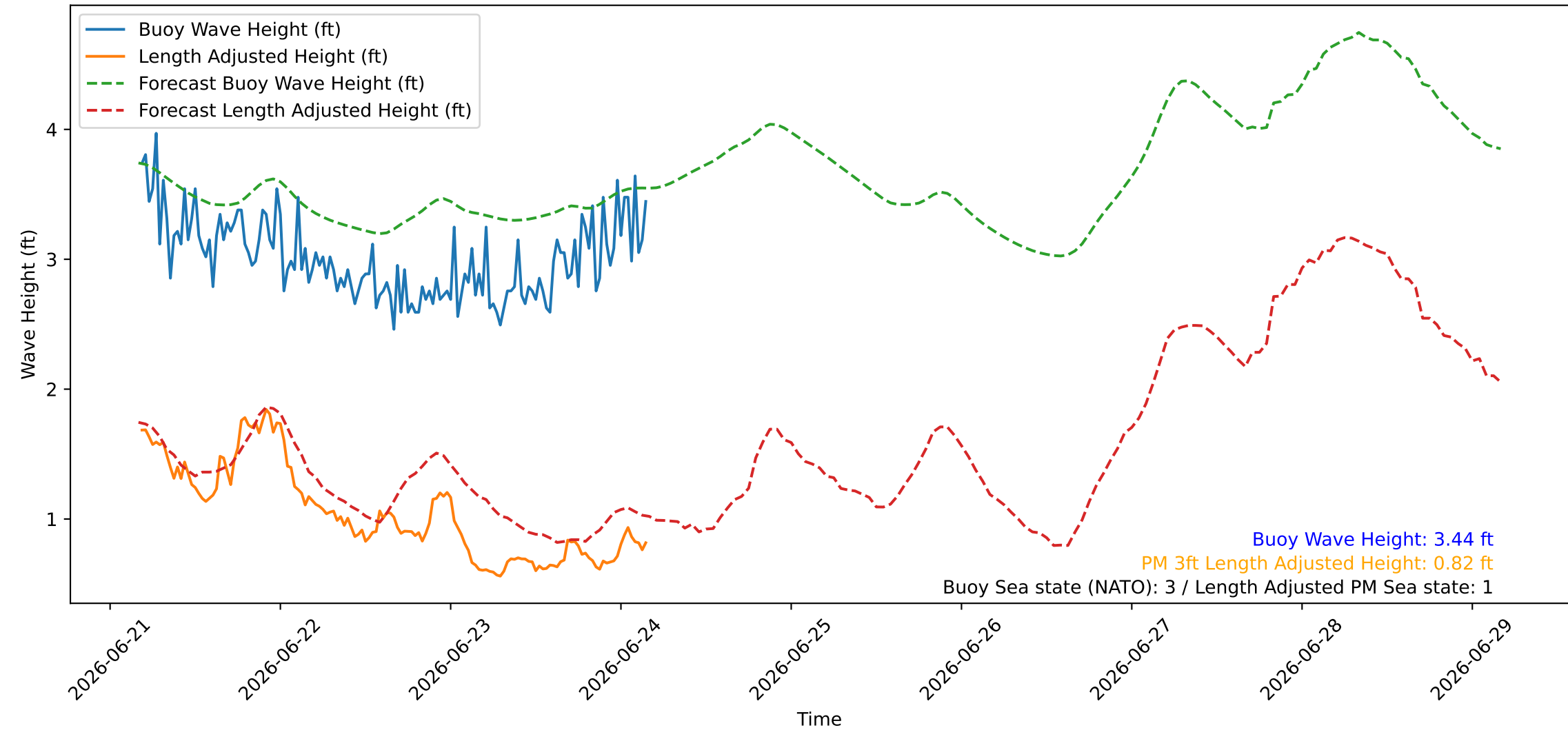
Wave Heights over Time for Green Beach at 2026-06-24 04:21:09
