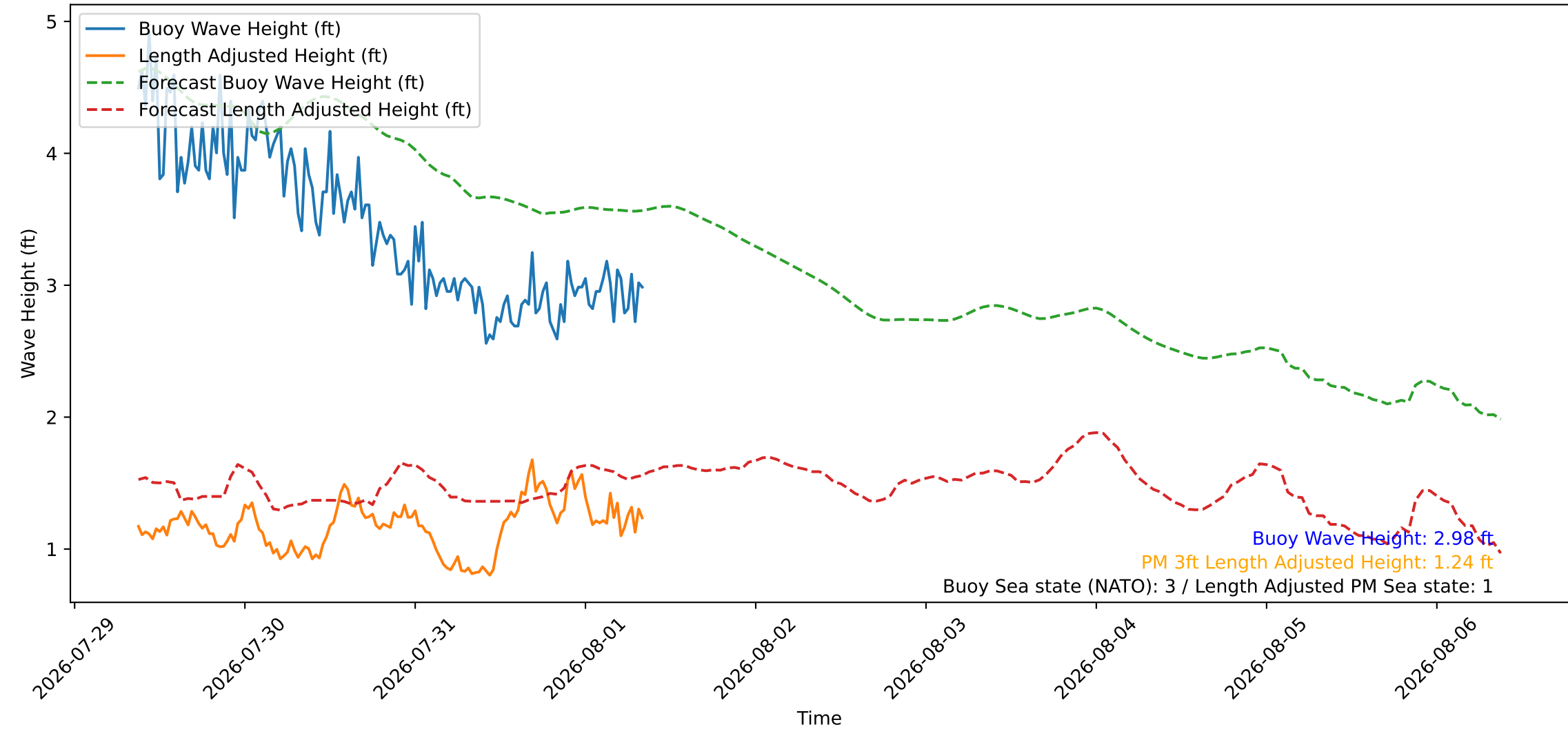
Wave Heights over Time for Red Beach at 2026-08-01 08:40:46
