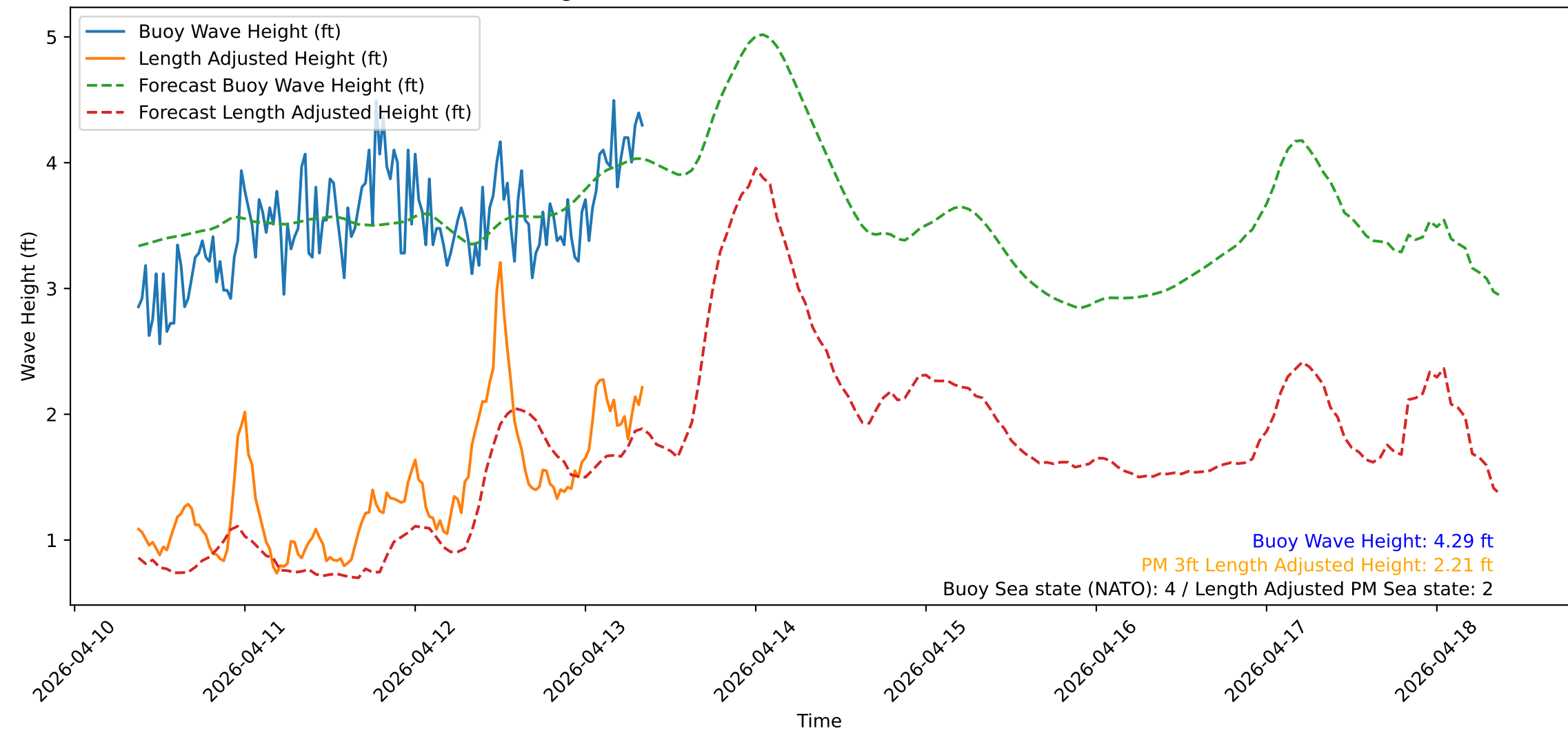
Wave Heights over Time for Green Beach at 2026-04-13 09:01:11
