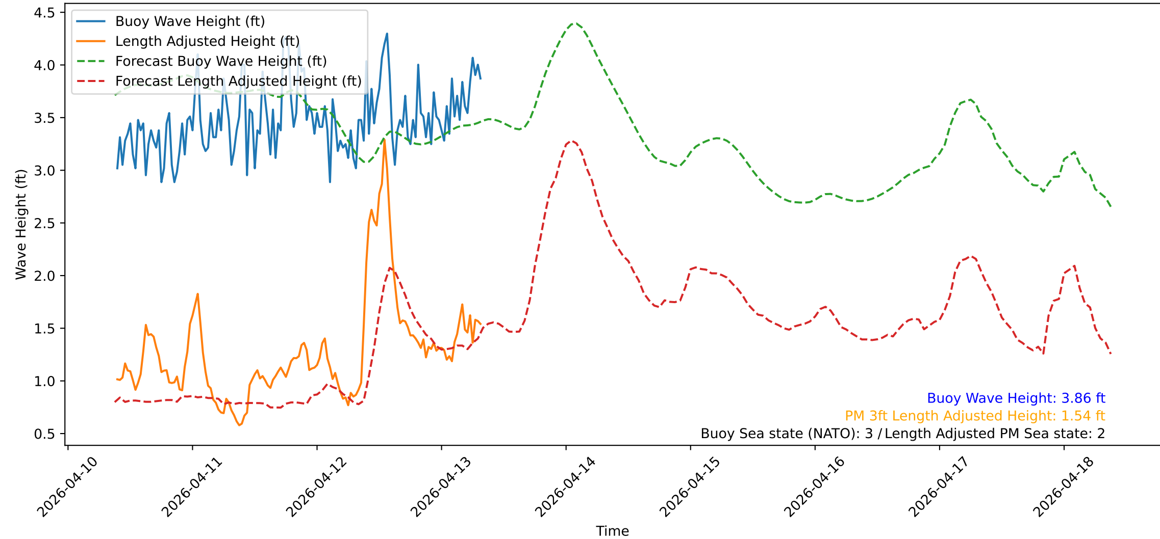
Wave Heights over Time for Red Beach at 2026-04-13 09:00:49
