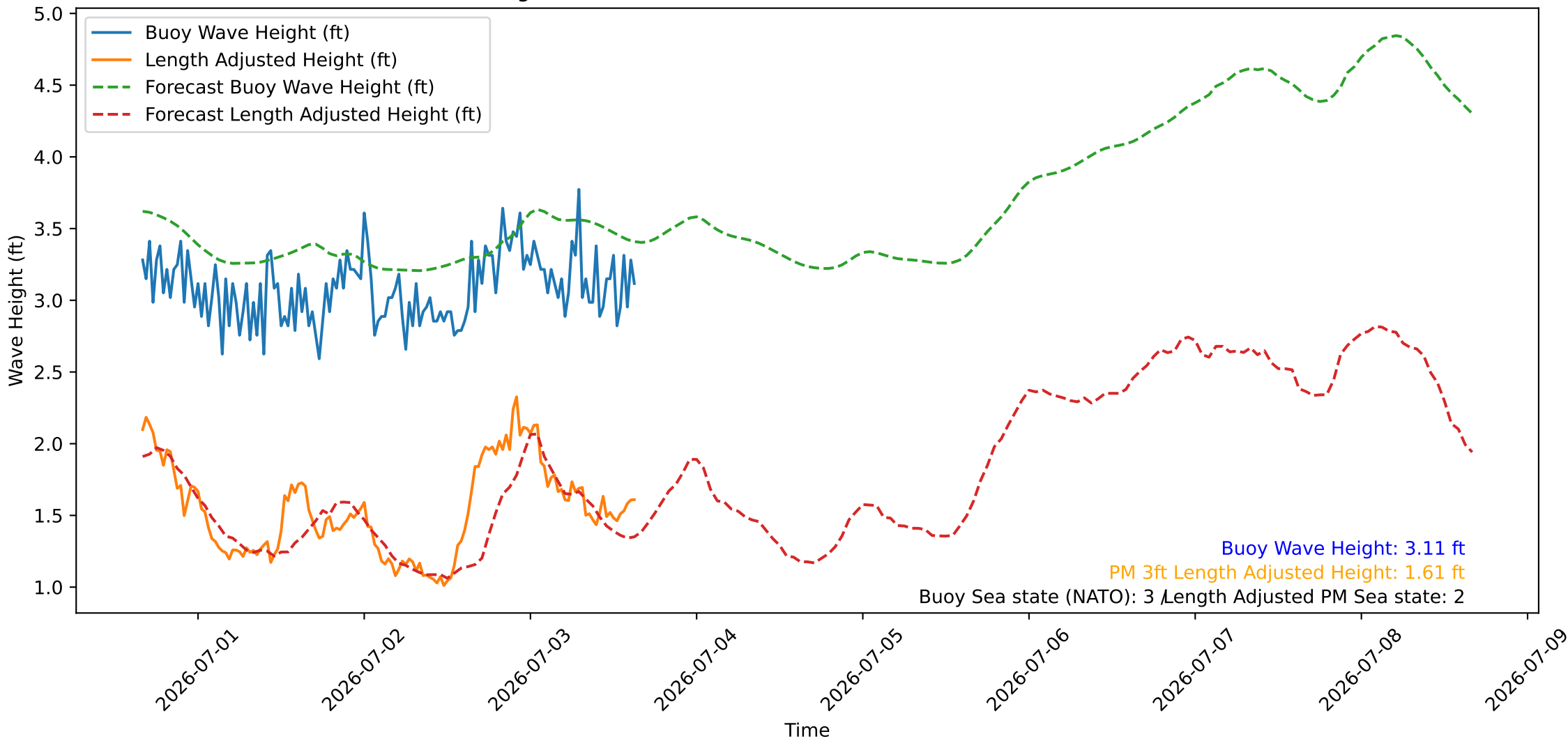
Wave Heights over Time for Oceanside Harbor at 2026-07-03 15:50:26
