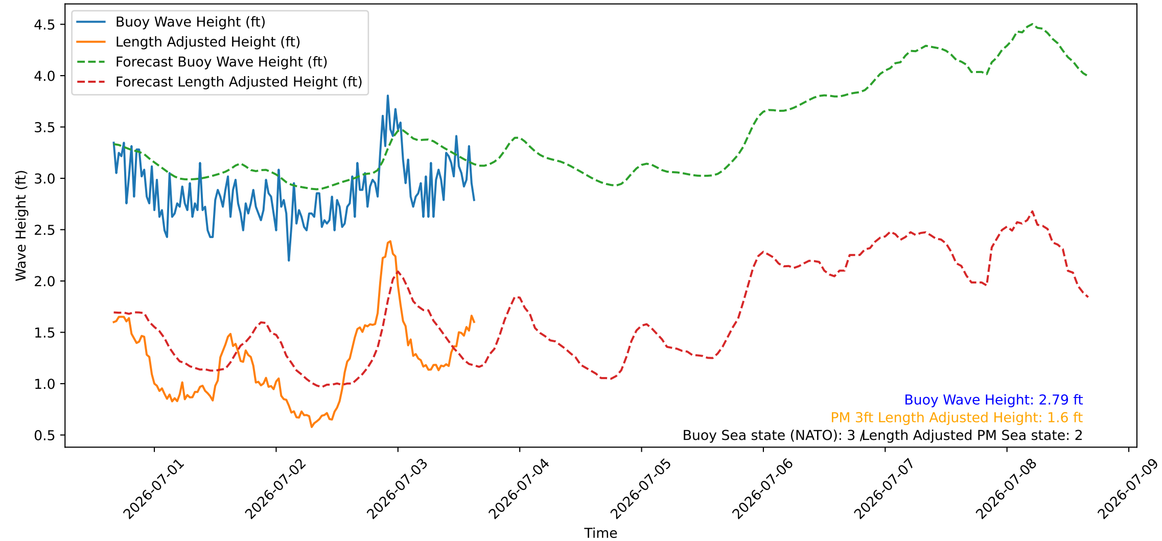
Wave Heights over Time for Red Beach at 2026-07-03 15:50:47
