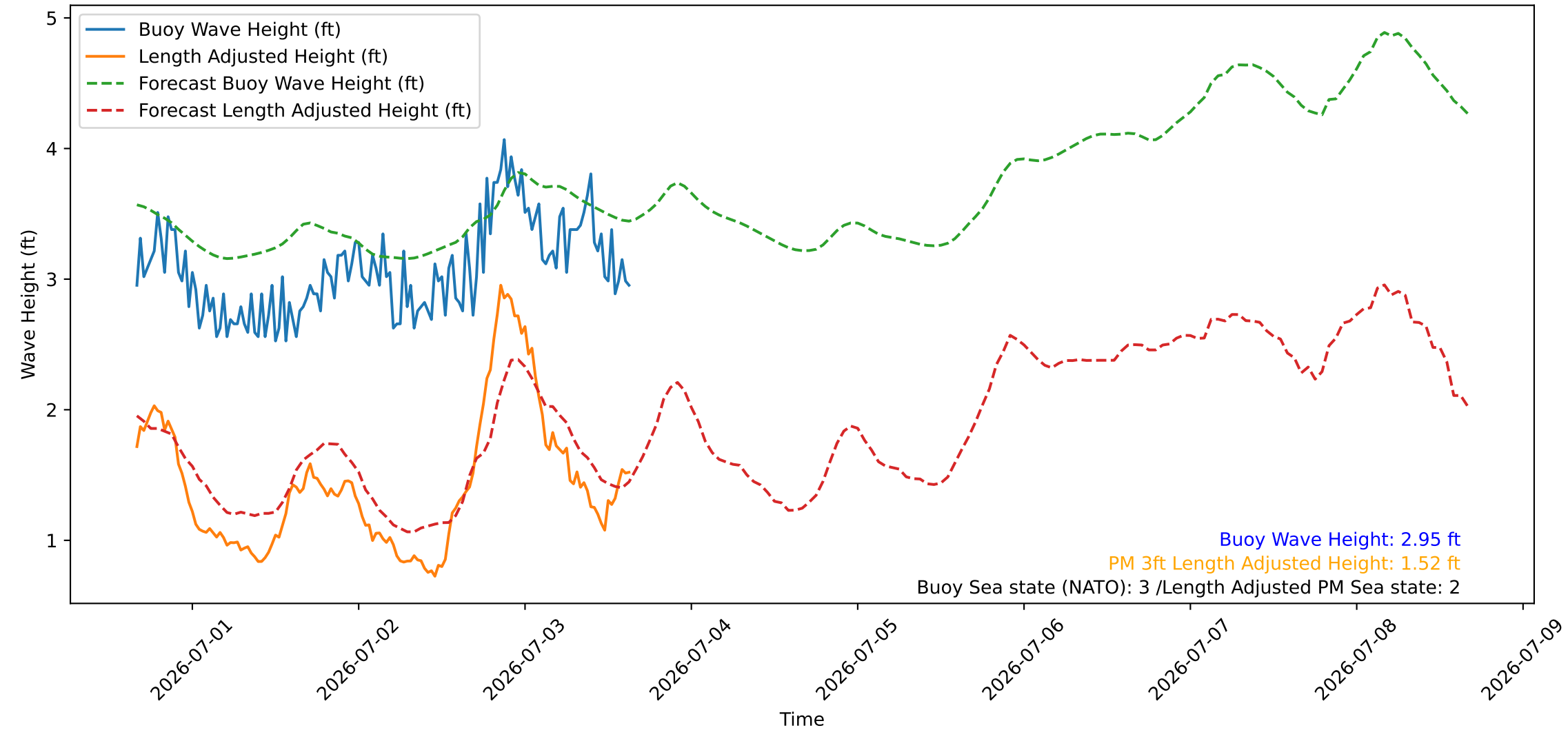
Wave Heights over Time for Green Beach at 2026-07-03 15:51:09
