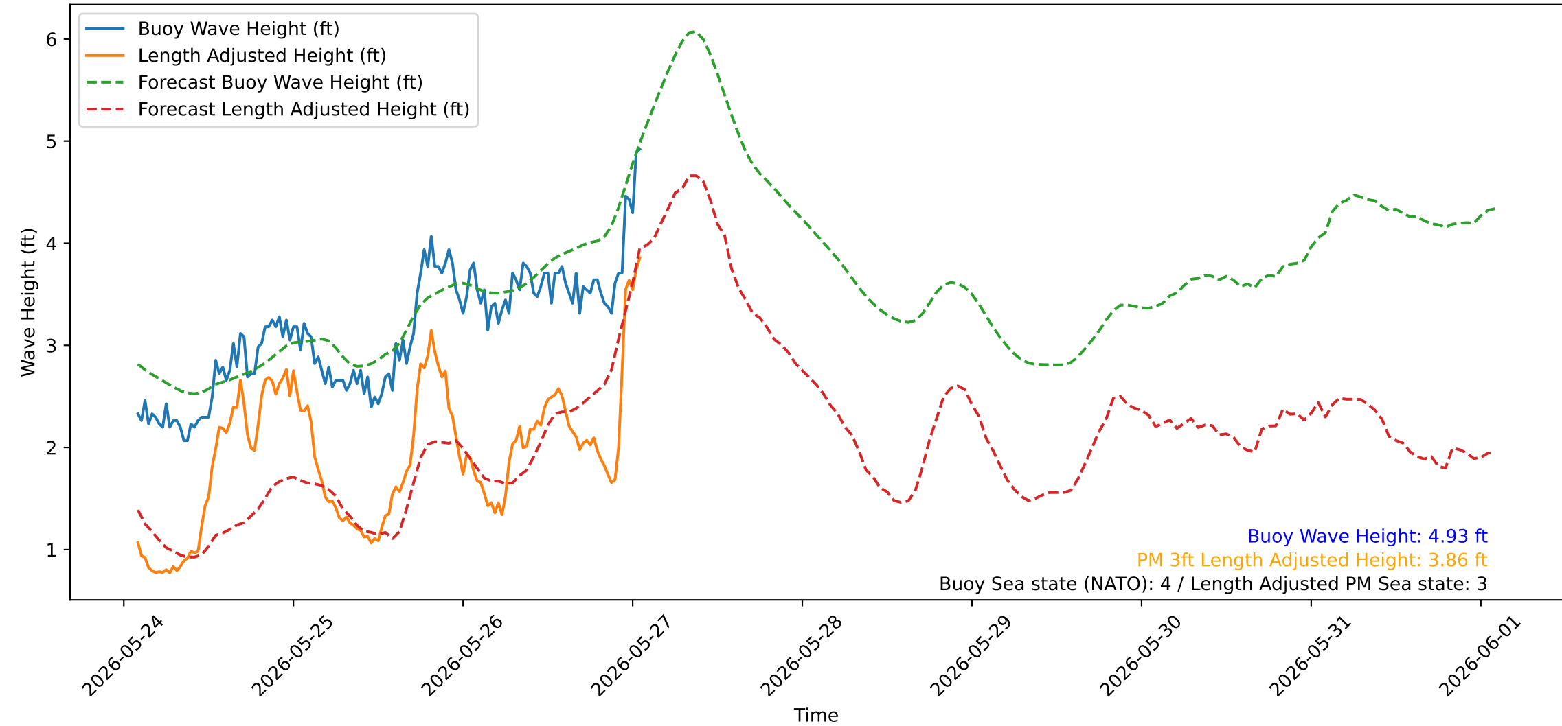
Wave Heights over Time for Green Beach at 2026-05-27 01:51:10
