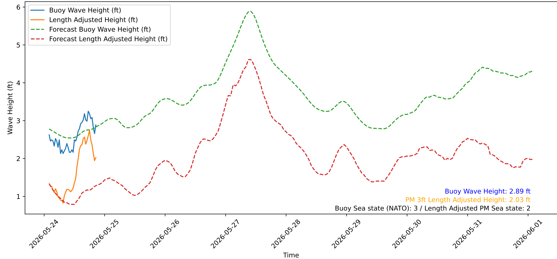
Wave Heights over Time for Oceanside Harbor at 2026-05-27 01:50:26
