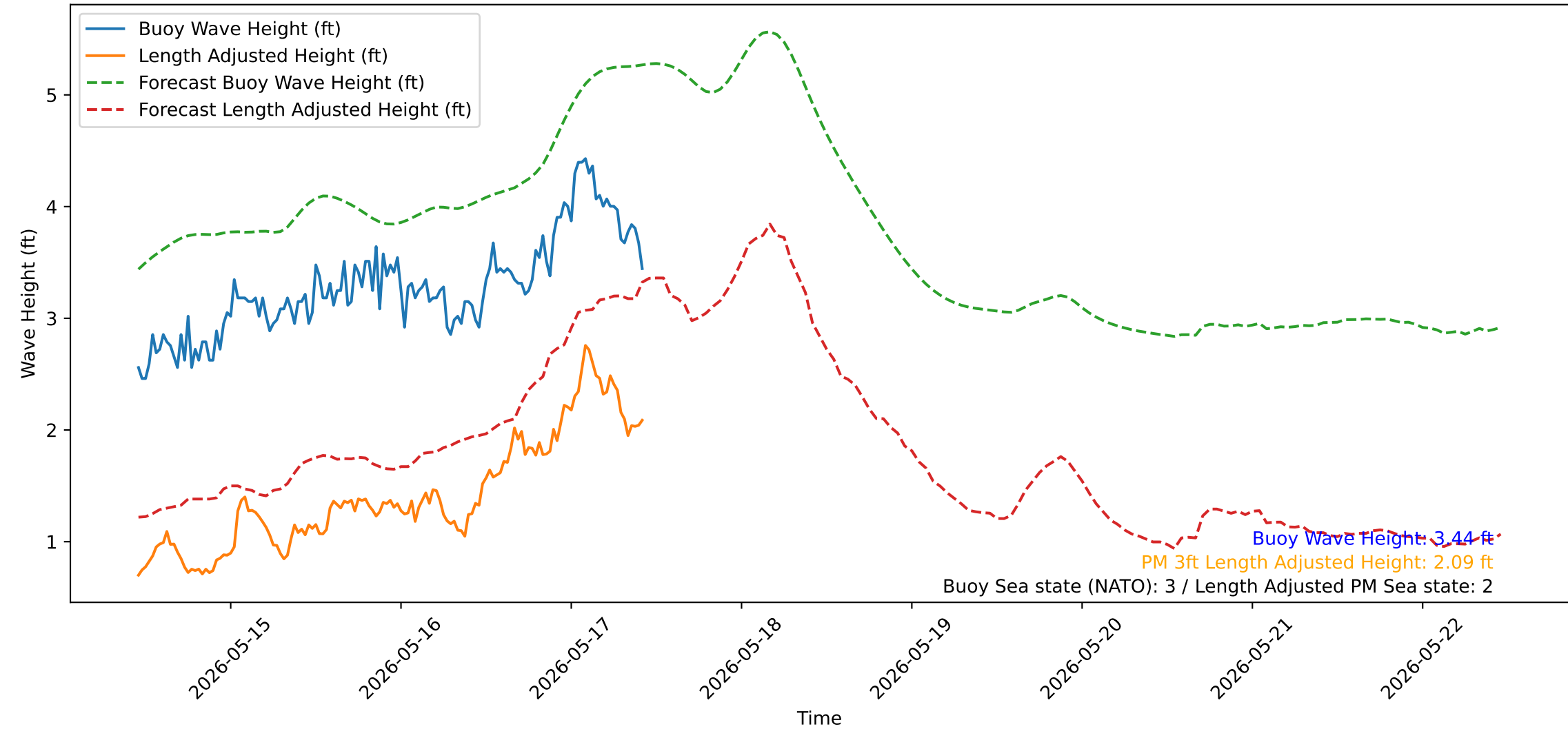
Wave Heights over Time for Green Beach at 2026-05-17 10:51:14
