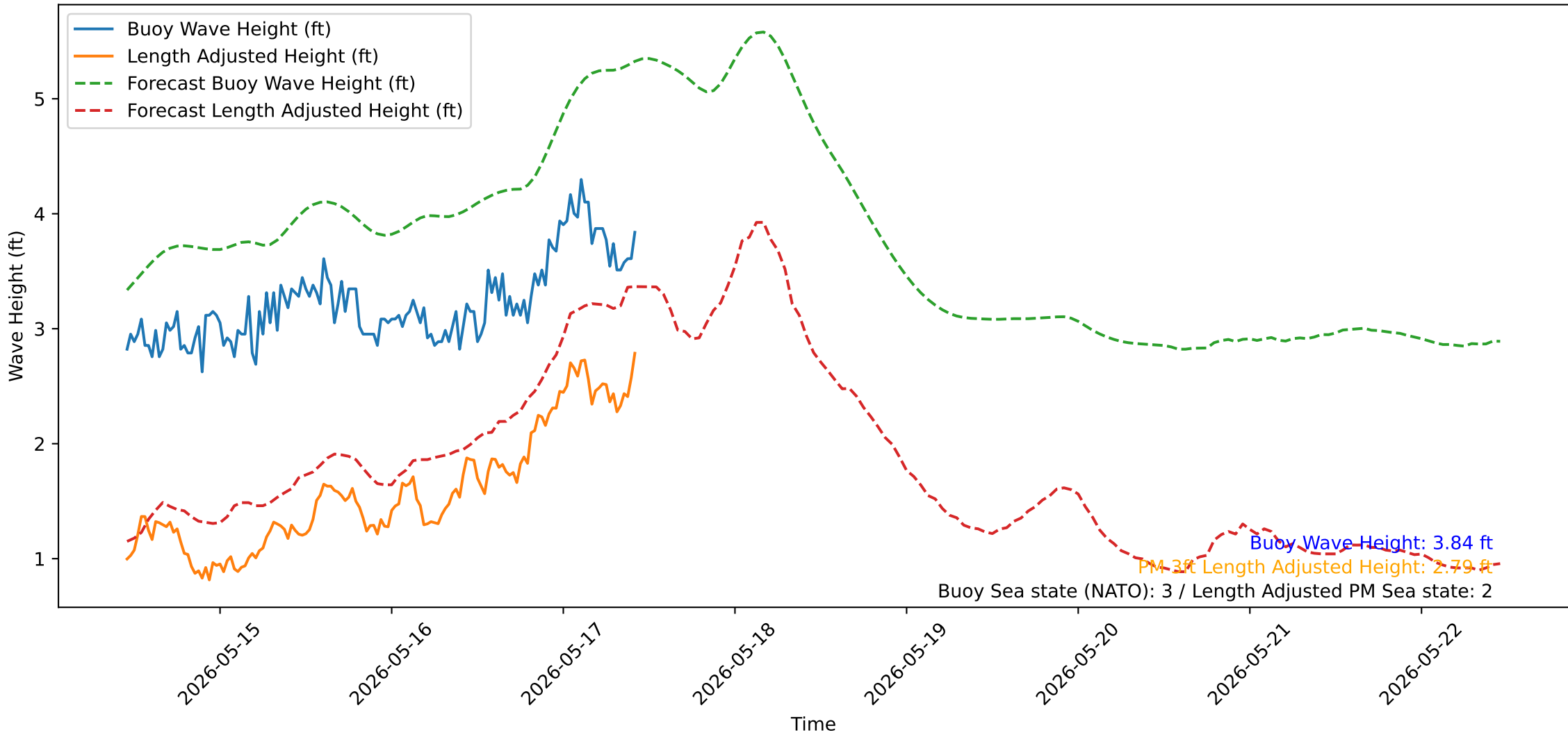
Wave Heights over Time for Oceanside Harbor at 2026-05-17 10:50:32
