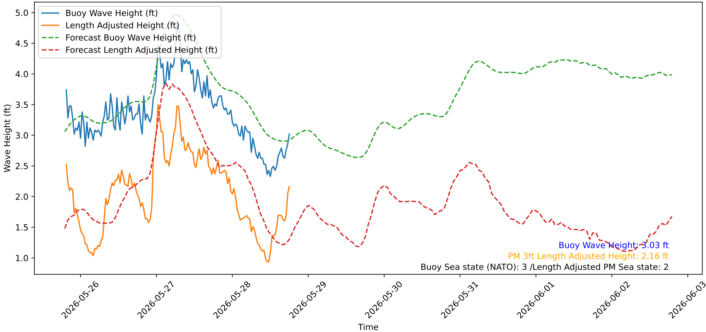
Wave Heights over Time for Red Beach at 2026-05-28 19:00:38
