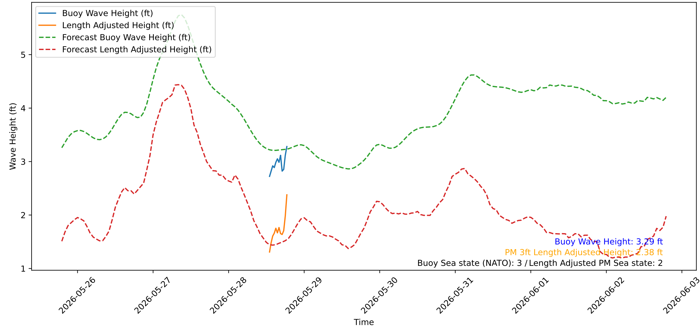
Wave Heights over Time for Oceanside Harbor at 2026-05-28 19:00:19
