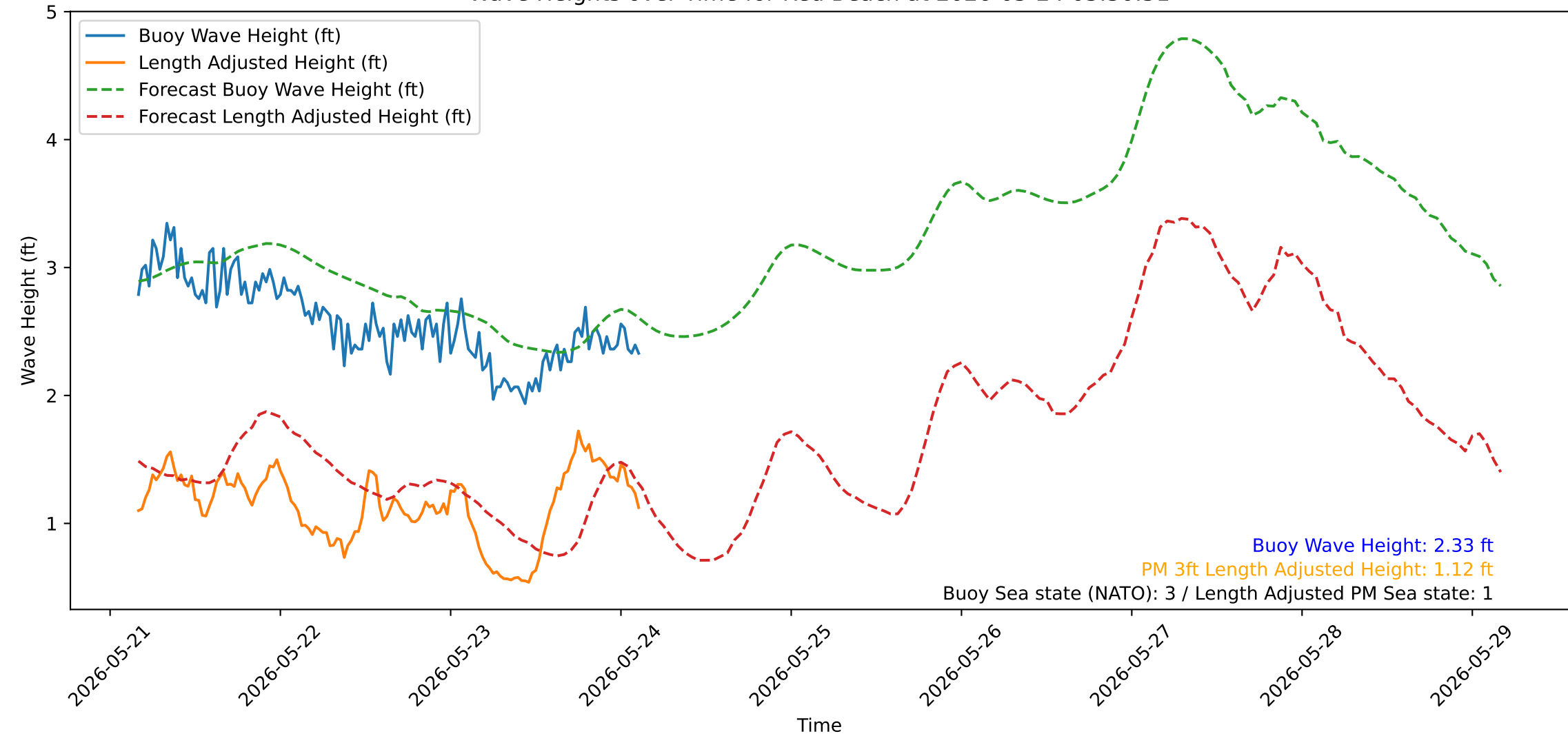
Wave Heights over Time for Red Beach at 2026-05-24 03:30:51
