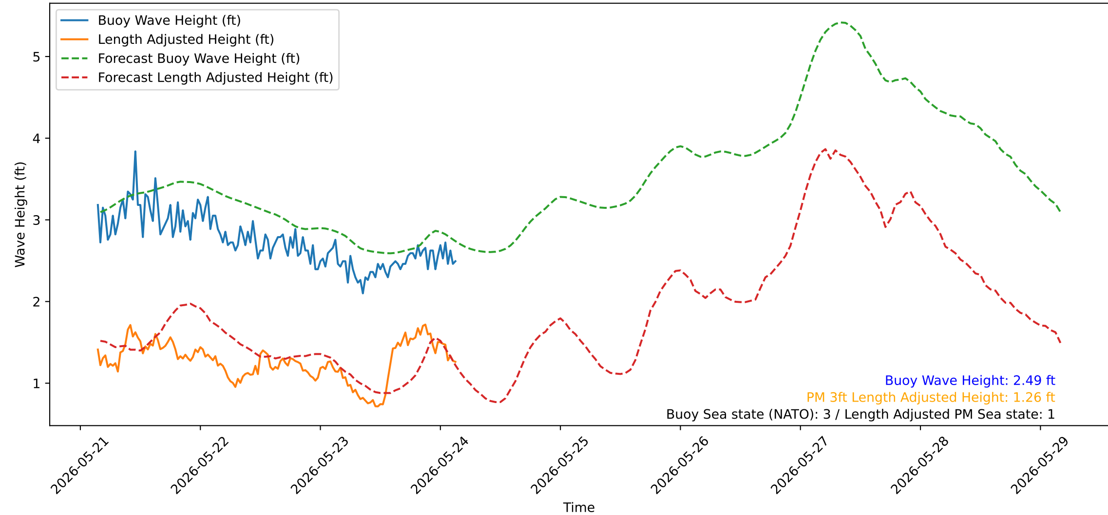
Wave Heights over Time for Oceanside Harbor at 2026-05-24 03:30:31
