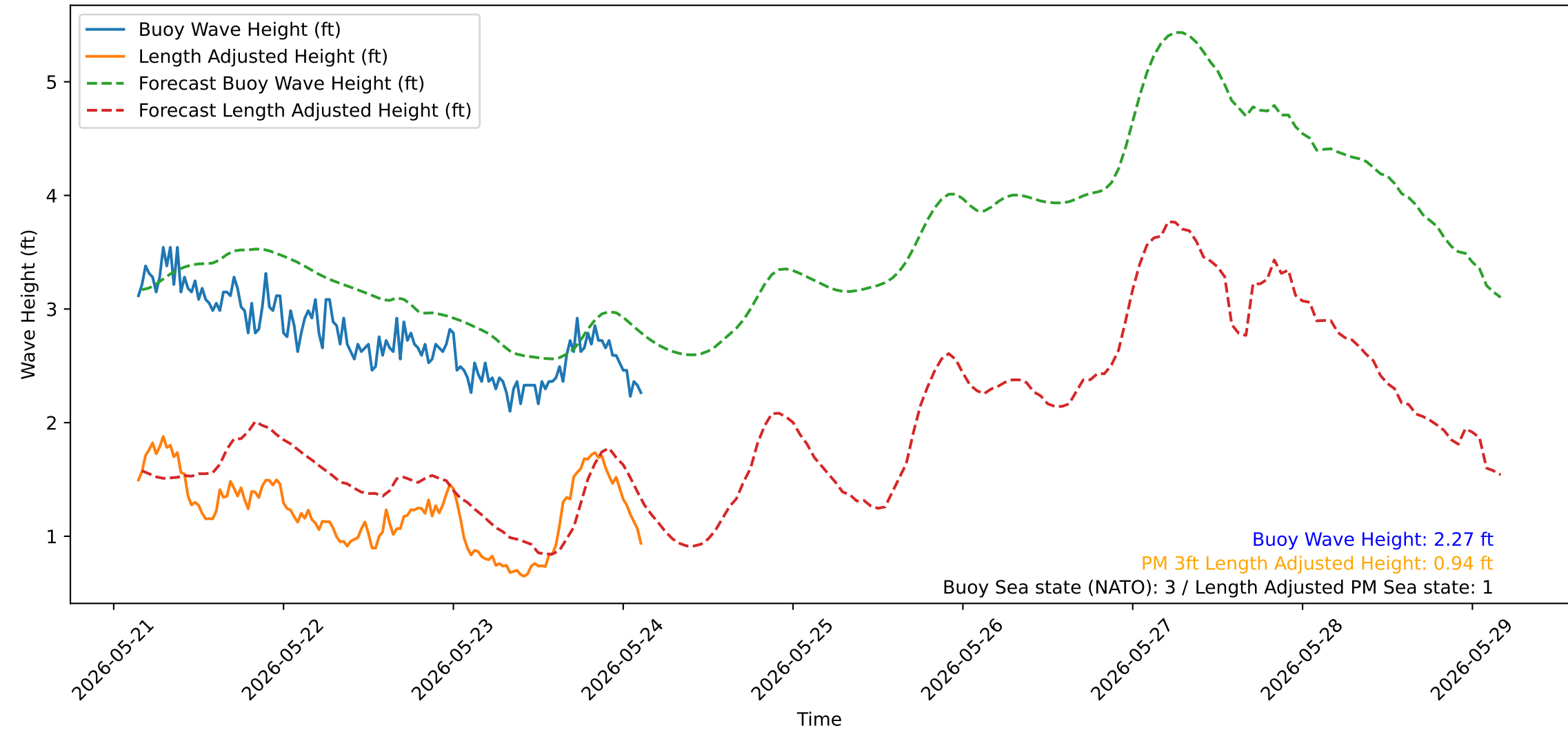
Wave Heights over Time for Green Beach at 2026-05-24 03:31:13
