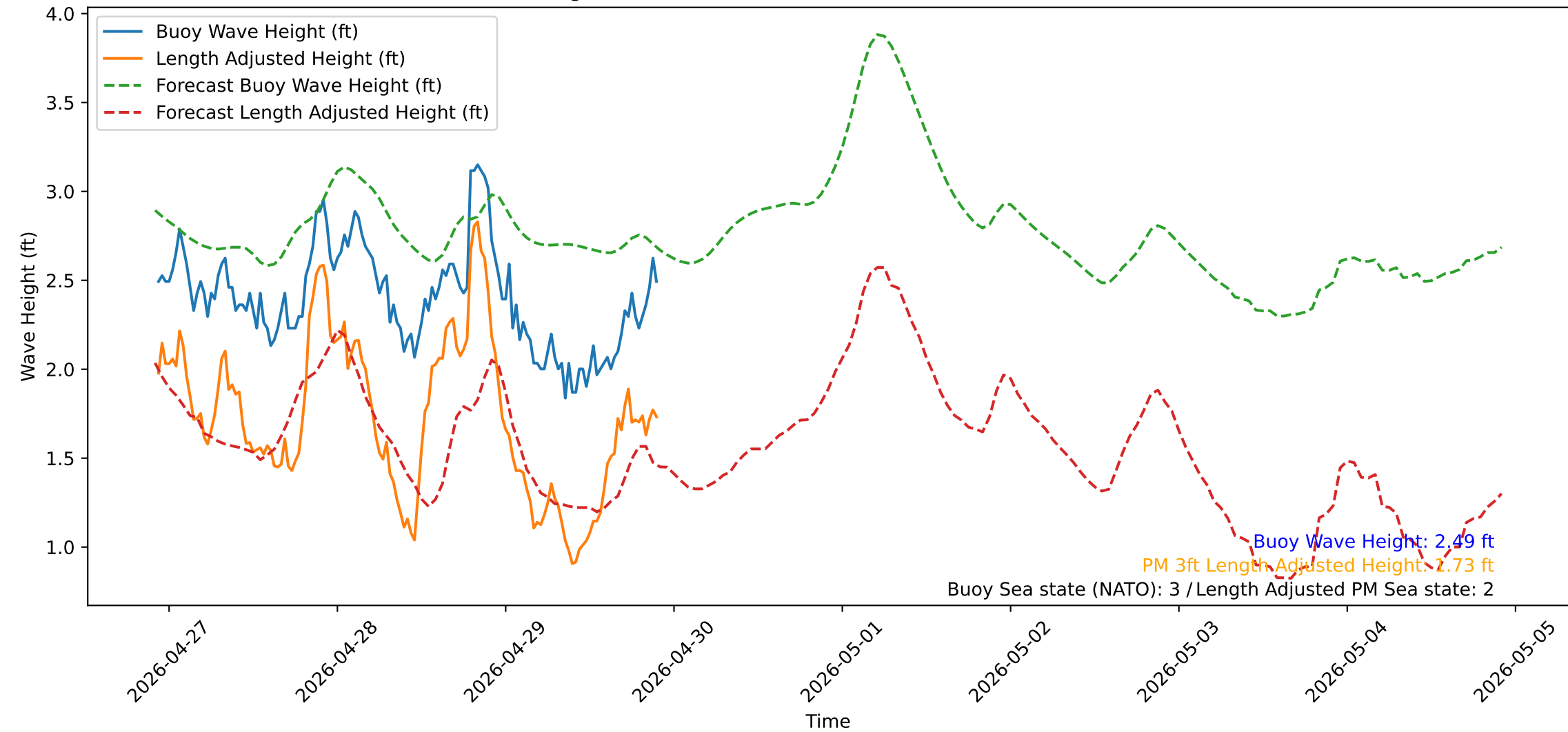
Wave Heights over Time for Green Beach at 2026-04-29 22:21:14
