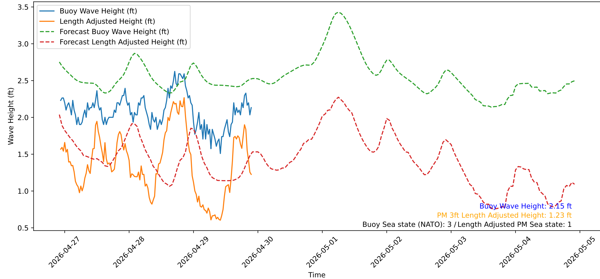
Wave Heights over Time for Red Beach at 2026-04-29 22:20:52
