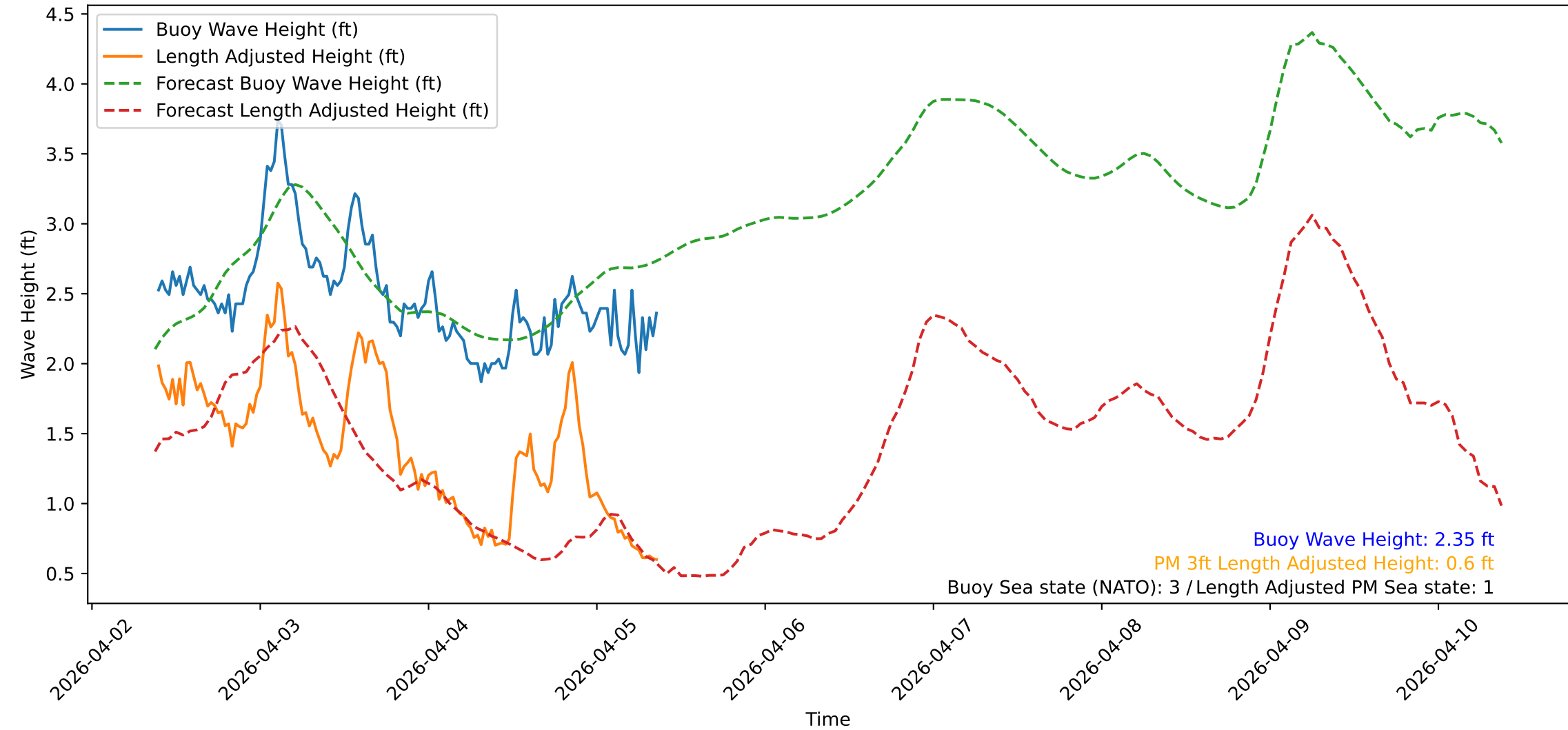
Wave Heights over Time for Red Beach at 2026-04-05 09:20:48
