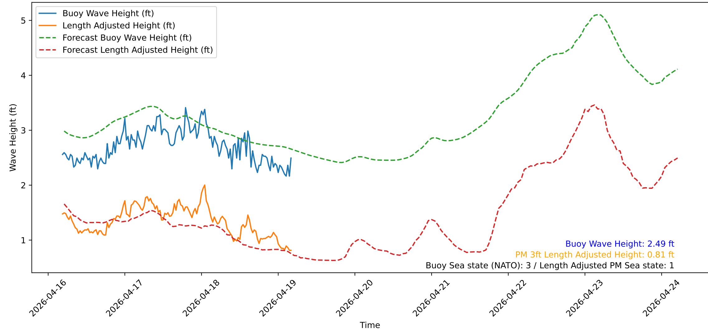
Wave Heights over Time for Oceanside Harbor at 2026-04-19 04:30:31
