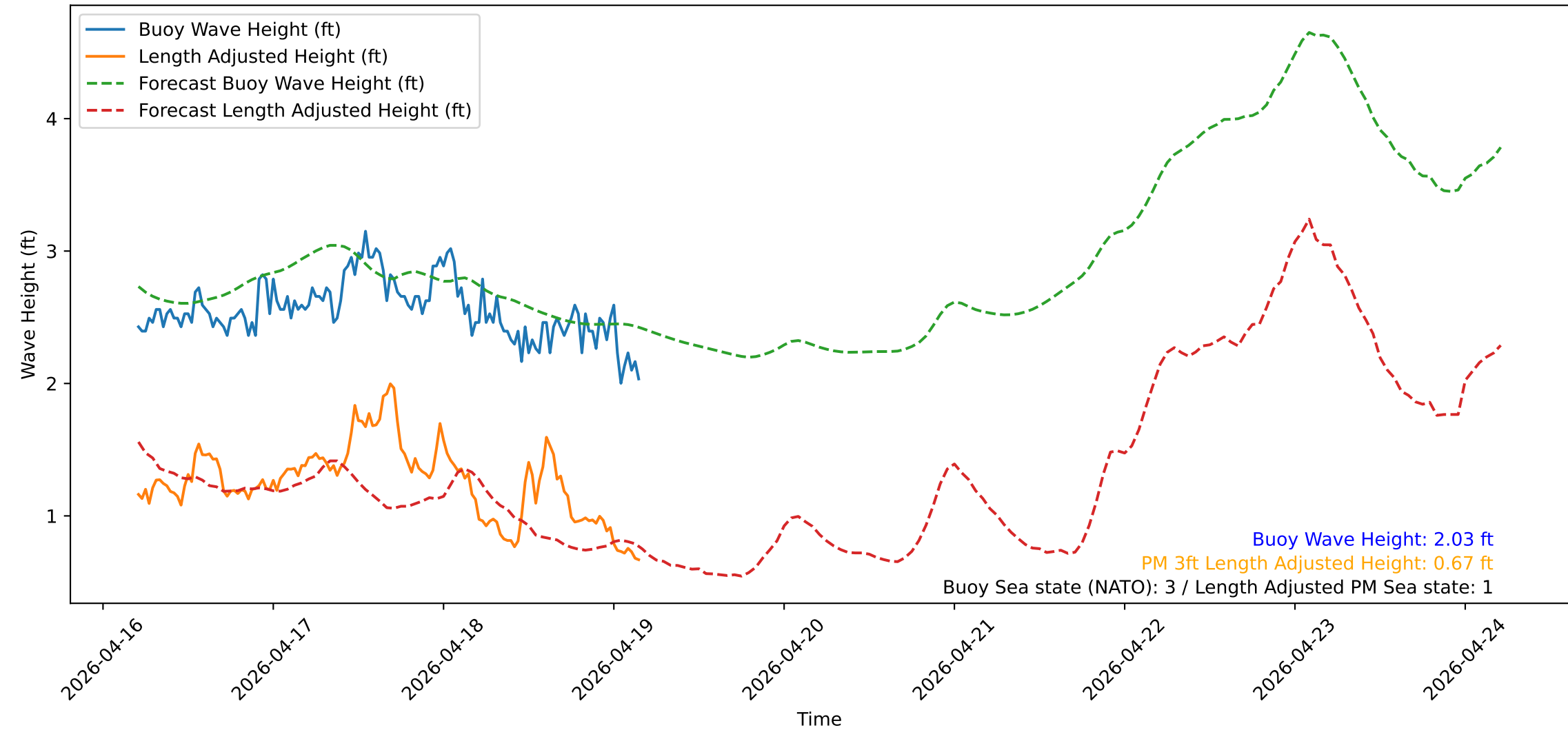
Wave Heights over Time for Red Beach at 2026-04-19 04:30:50
