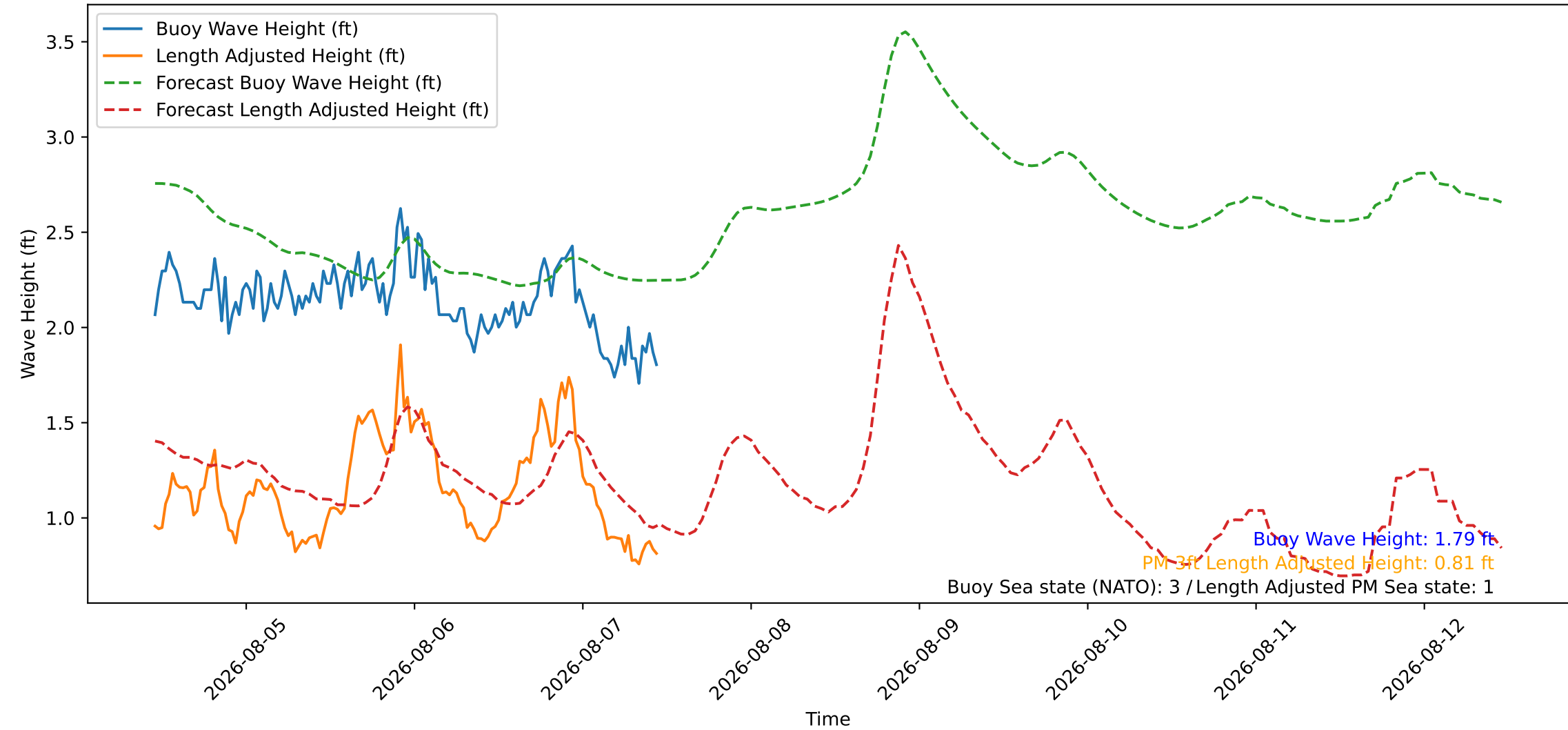
Wave Heights over Time for Green Beach at 2026-08-07 11:11:07
