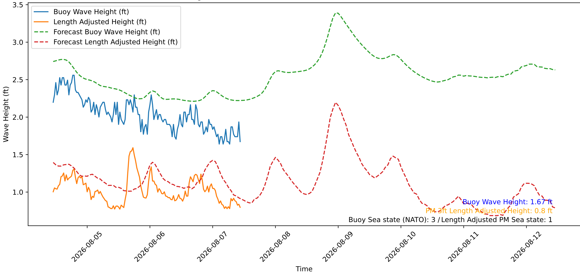
Wave Heights over Time for Oceanside Harbor at 2026-08-07 11:10:26
