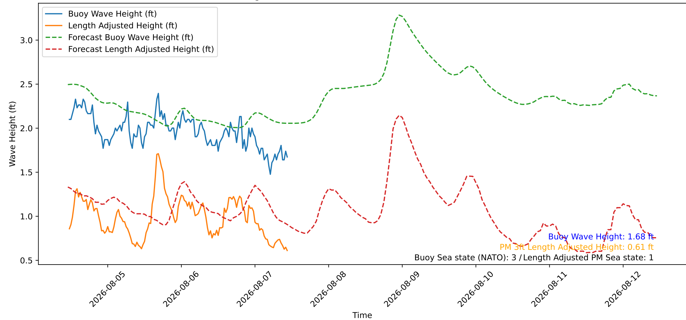
Wave Heights over Time for Red Beach at 2026-08-07 11:10:45
