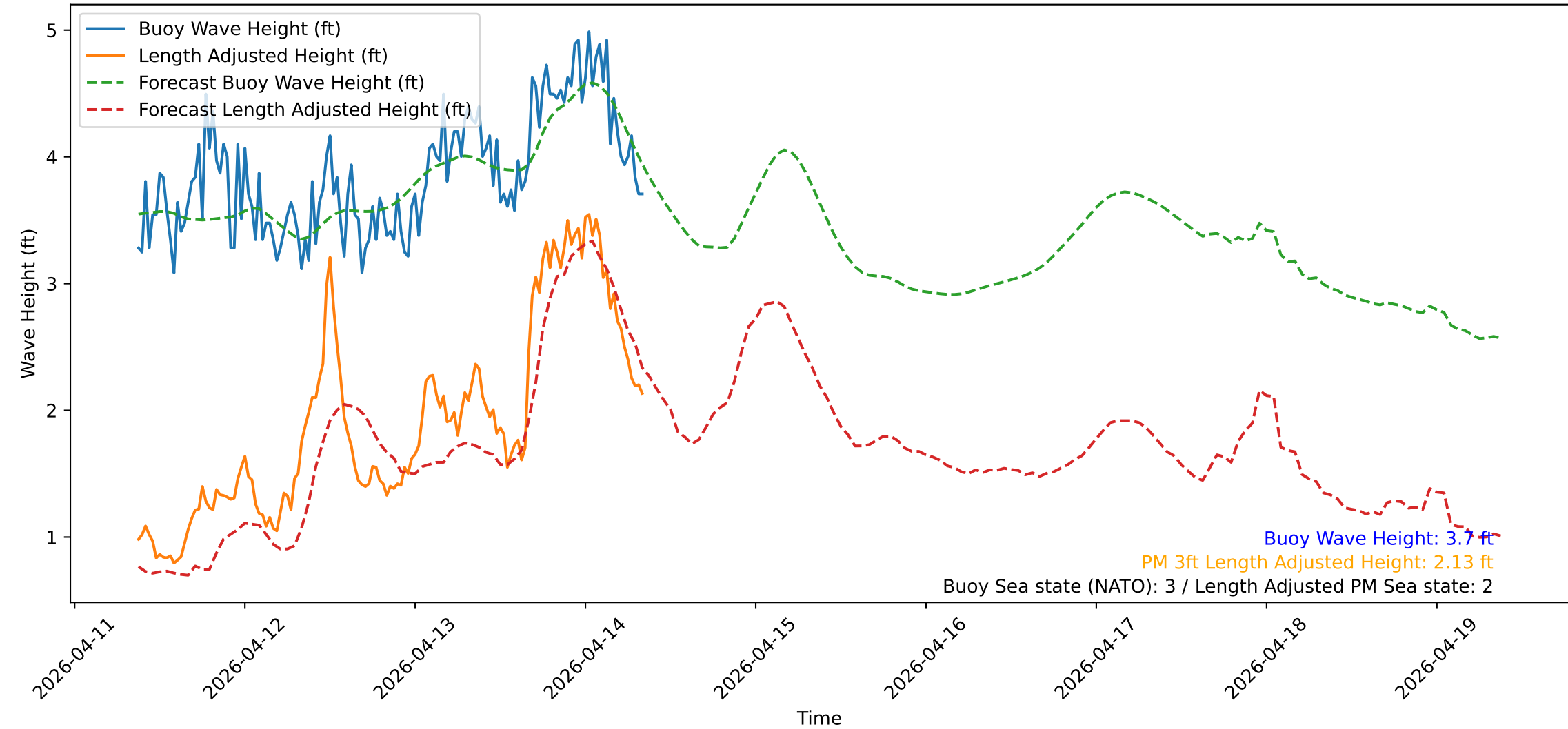
Wave Heights over Time for Green Beach at 2026-04-14 09:01:12
