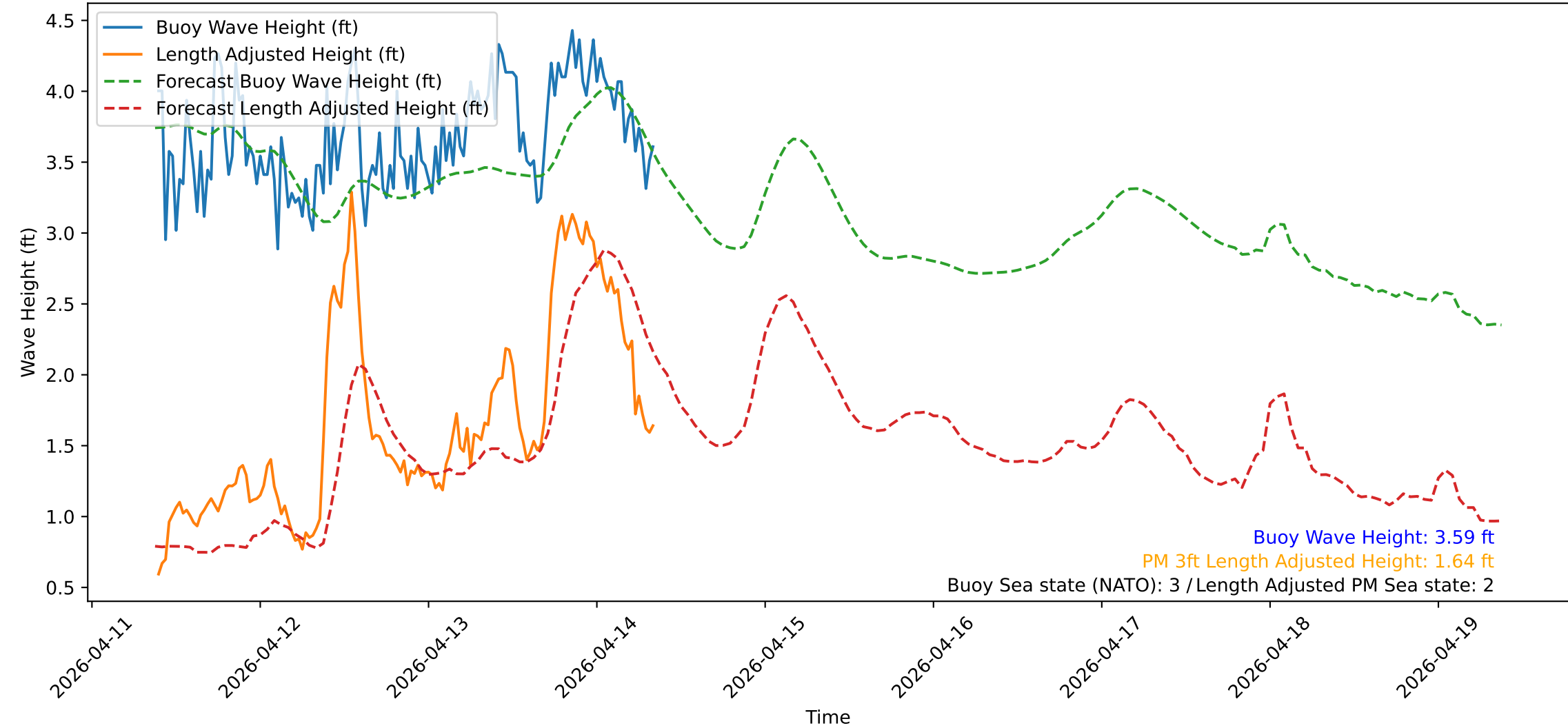
Wave Heights over Time for Red Beach at 2026-04-14 09:00:50
