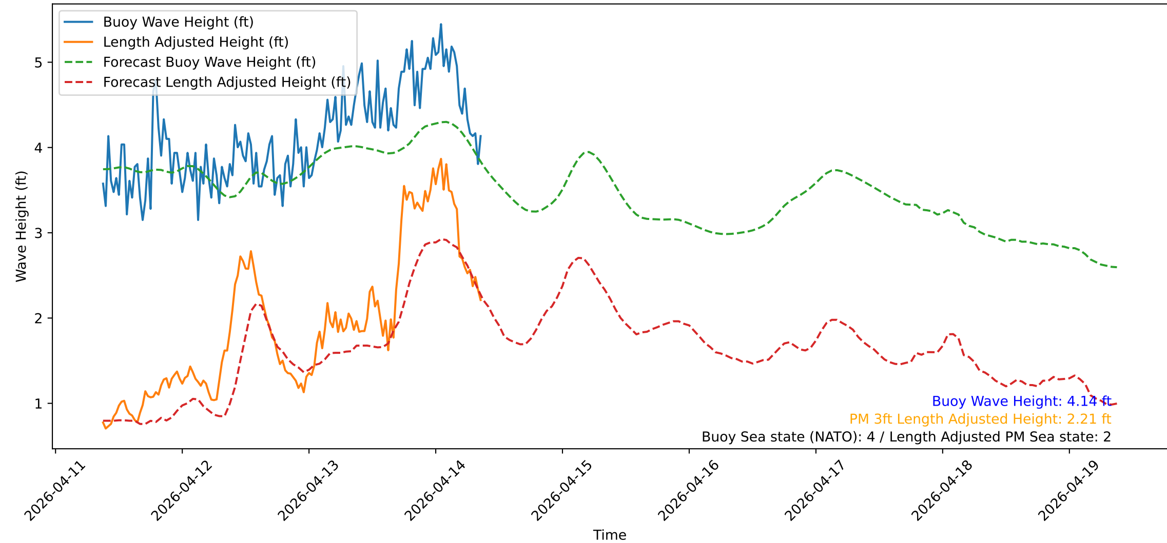
Wave Heights over Time for Oceanside Harbor at 2026-04-14 09:00:31
