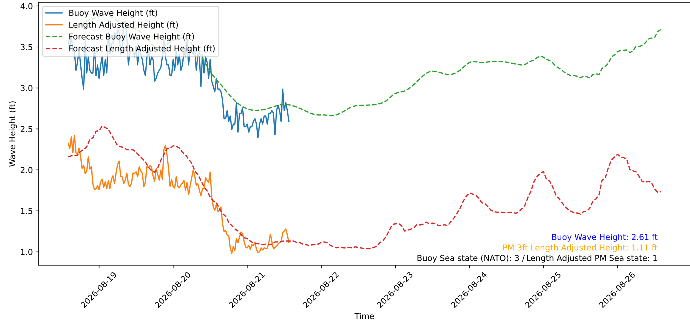
Wave Heights over Time for Oceanside Harbor at 2026-08-21 14:10:27
