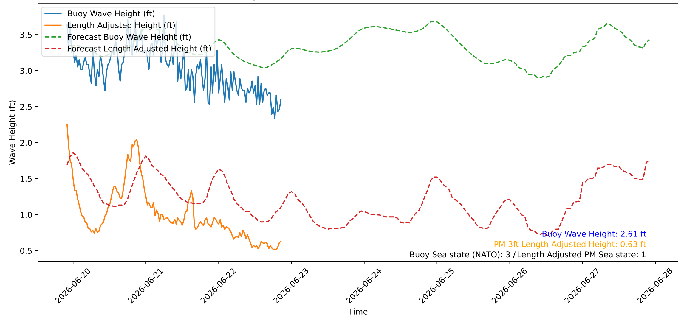
Wave Heights over Time for Red Beach at 2026-06-22 21:30:46
