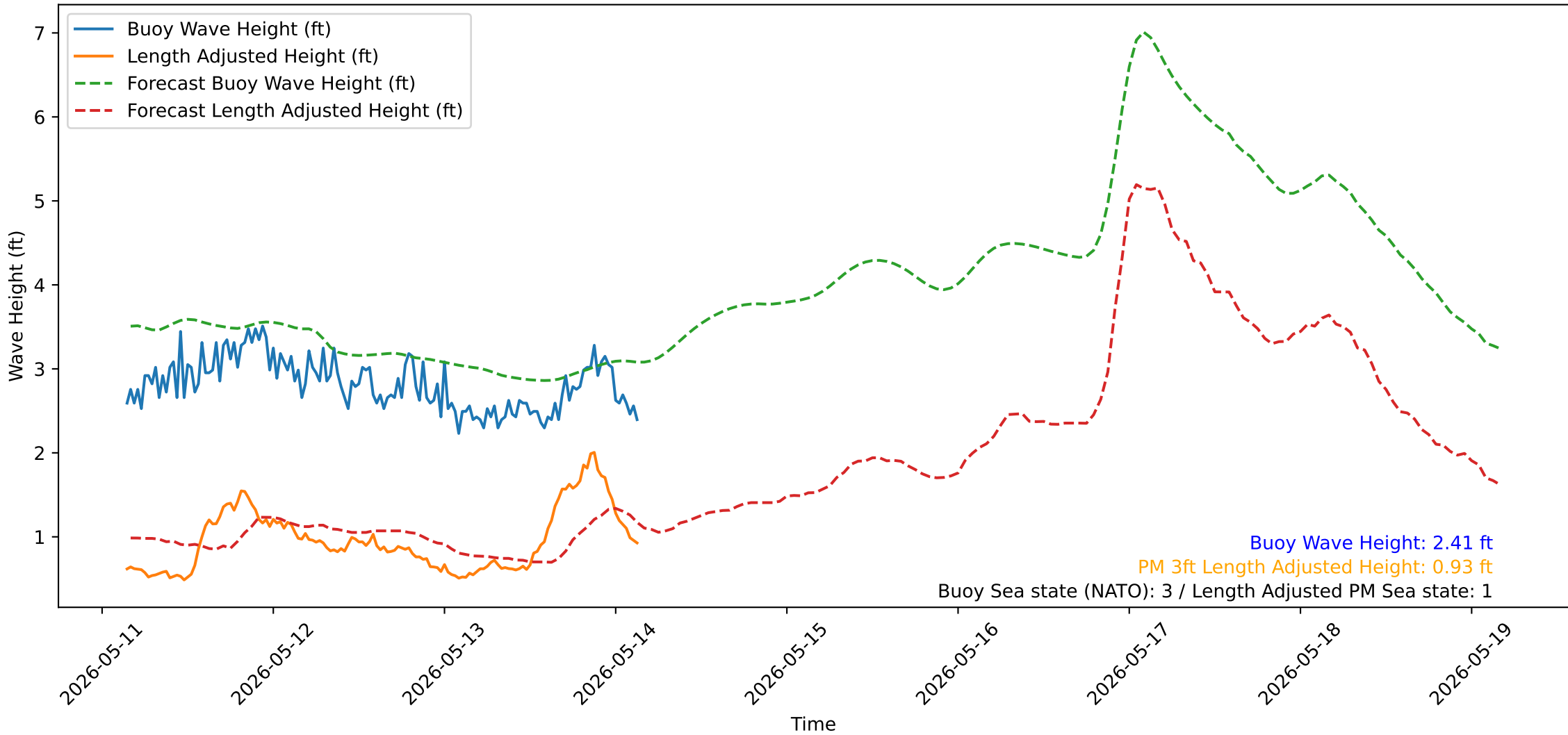
Wave Heights over Time for Green Beach at 2026-05-14 03:41:14
