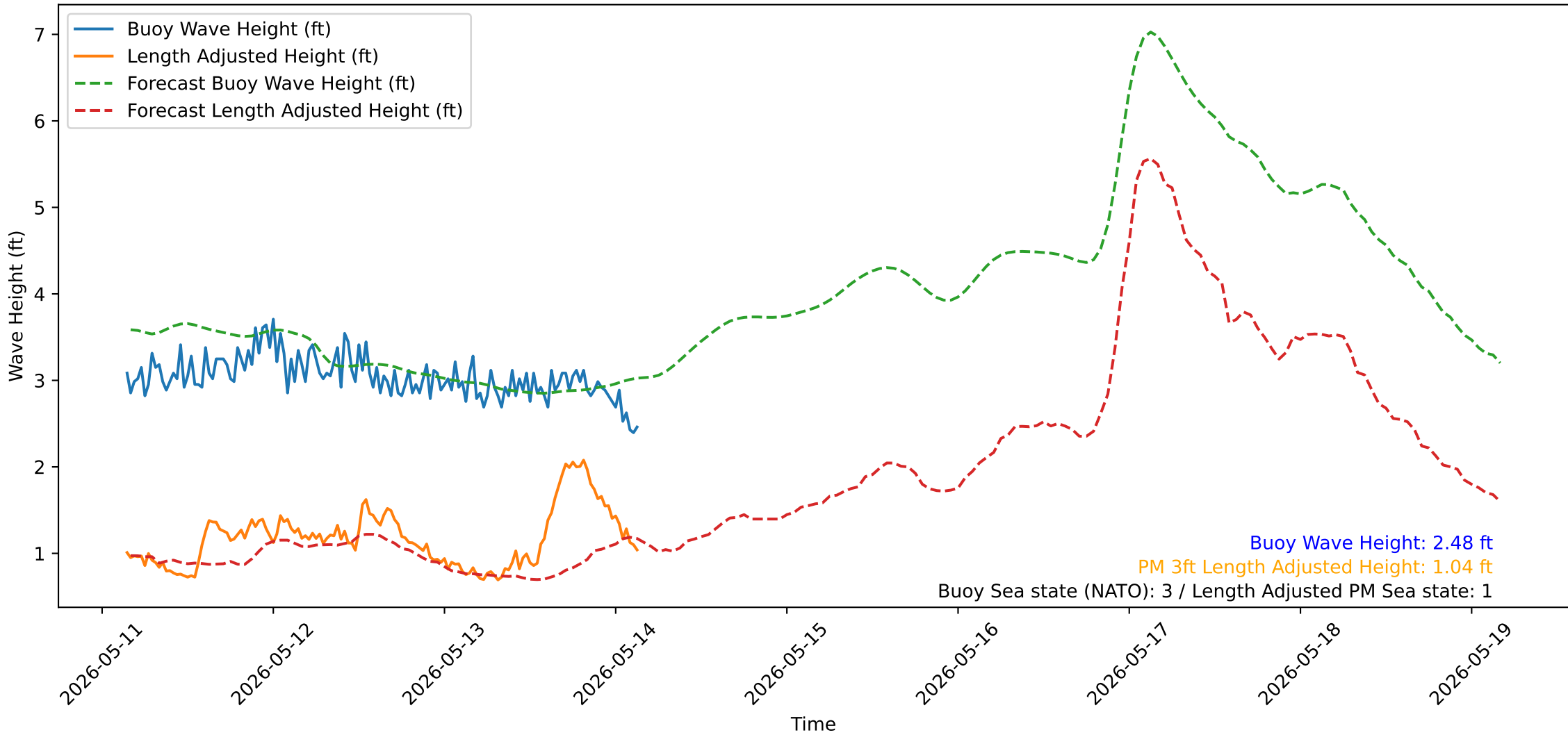
Wave Heights over Time for Oceanside Harbor at 2026-05-14 03:40:31
