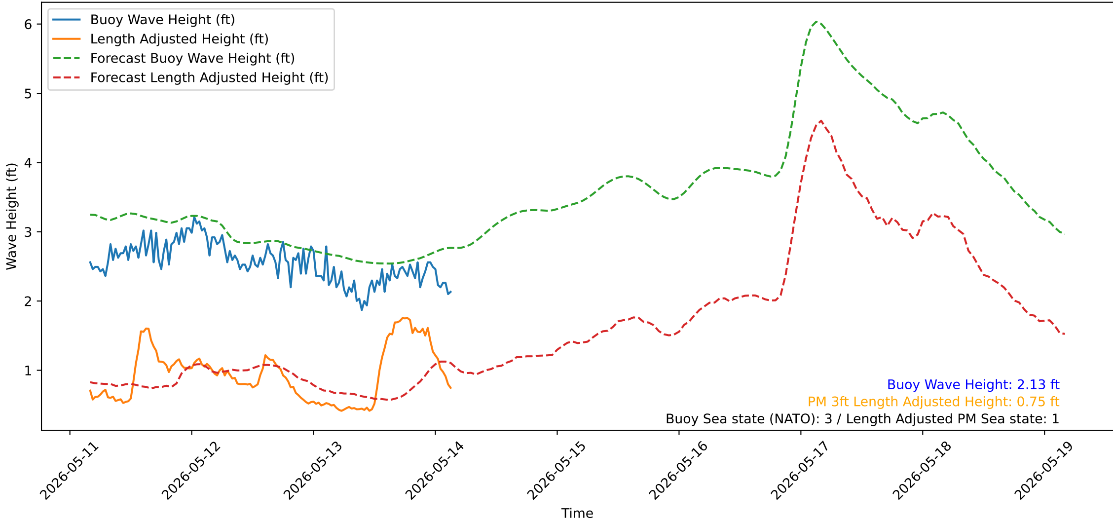
Wave Heights over Time for Red Beach at 2026-05-14 03:40:50
