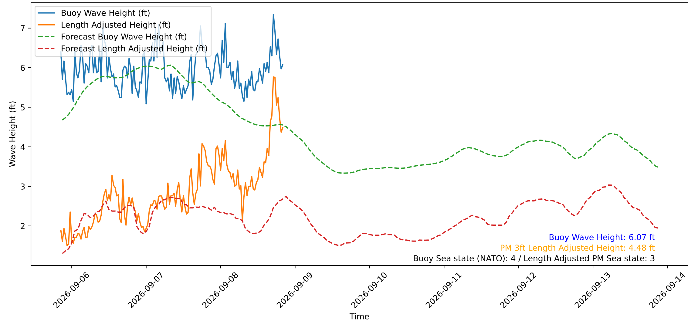
Wave Heights over Time for Oceanside Harbor at 2026-09-08 20:30:30
