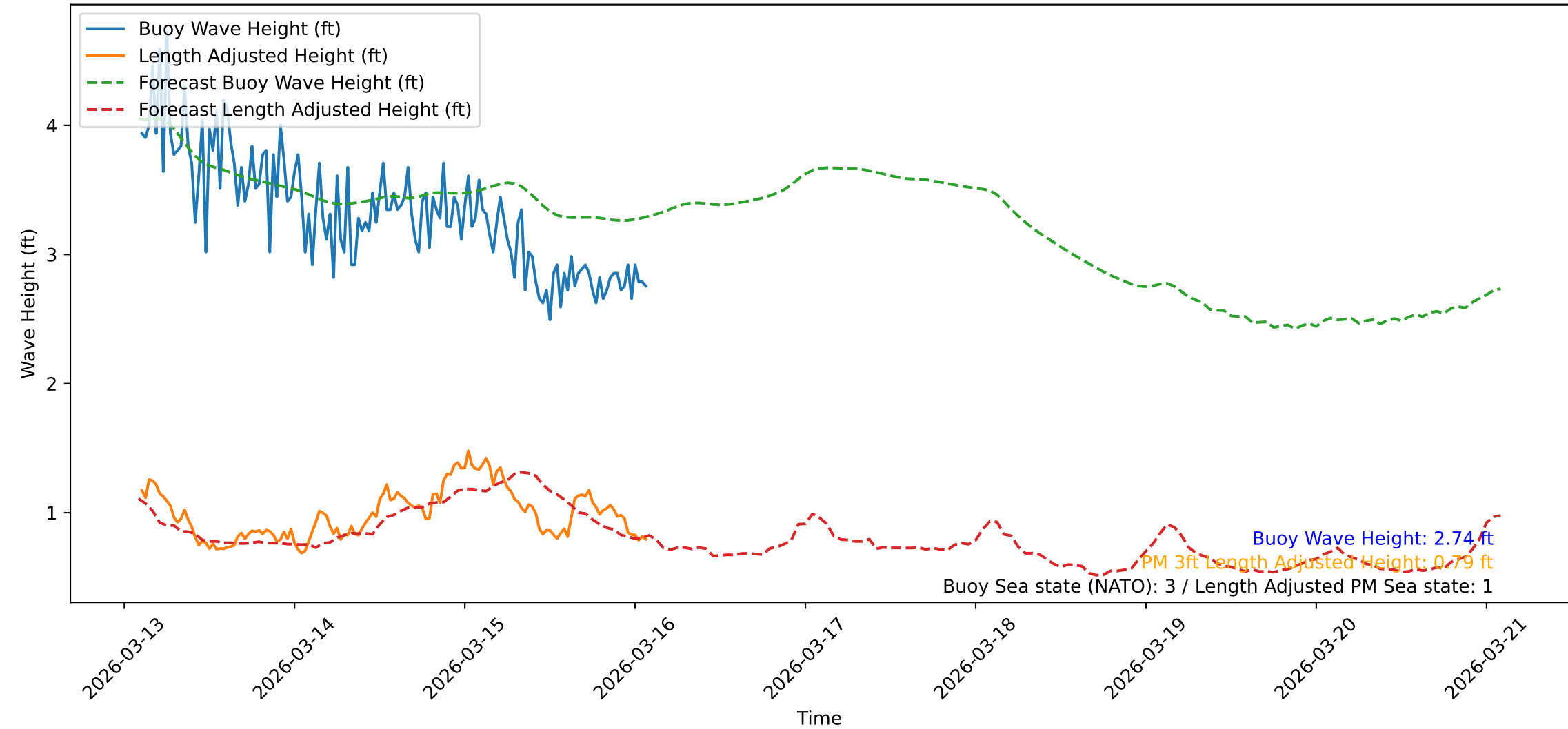
Wave Heights over Time for Oceanside Harbor at 2026-03-16 02:21:28
