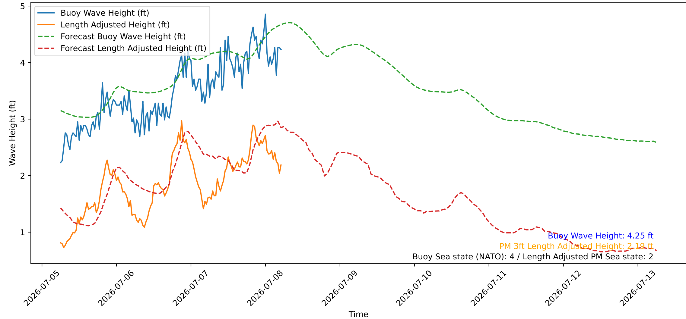
Wave Heights over Time for Red Beach at 2026-07-08 05:50:47
