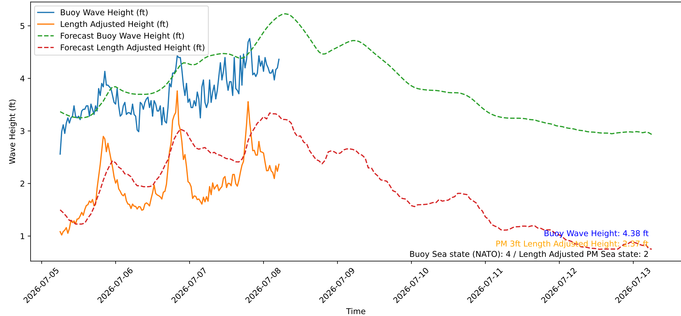
Wave Heights over Time for Green Beach at 2026-07-08 05:51:09
