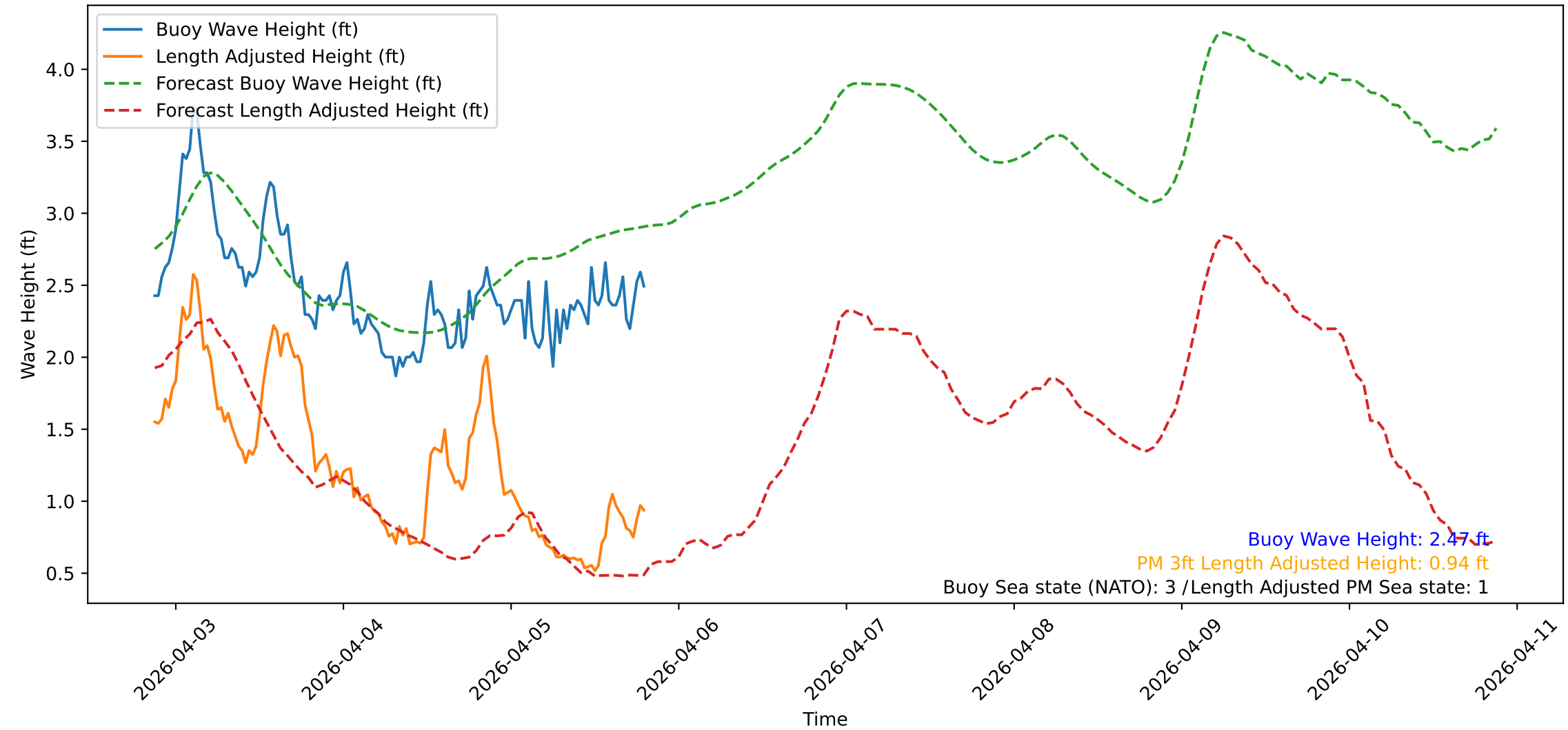
Wave Heights over Time for Red Beach at 2026-04-05 20:30:59
