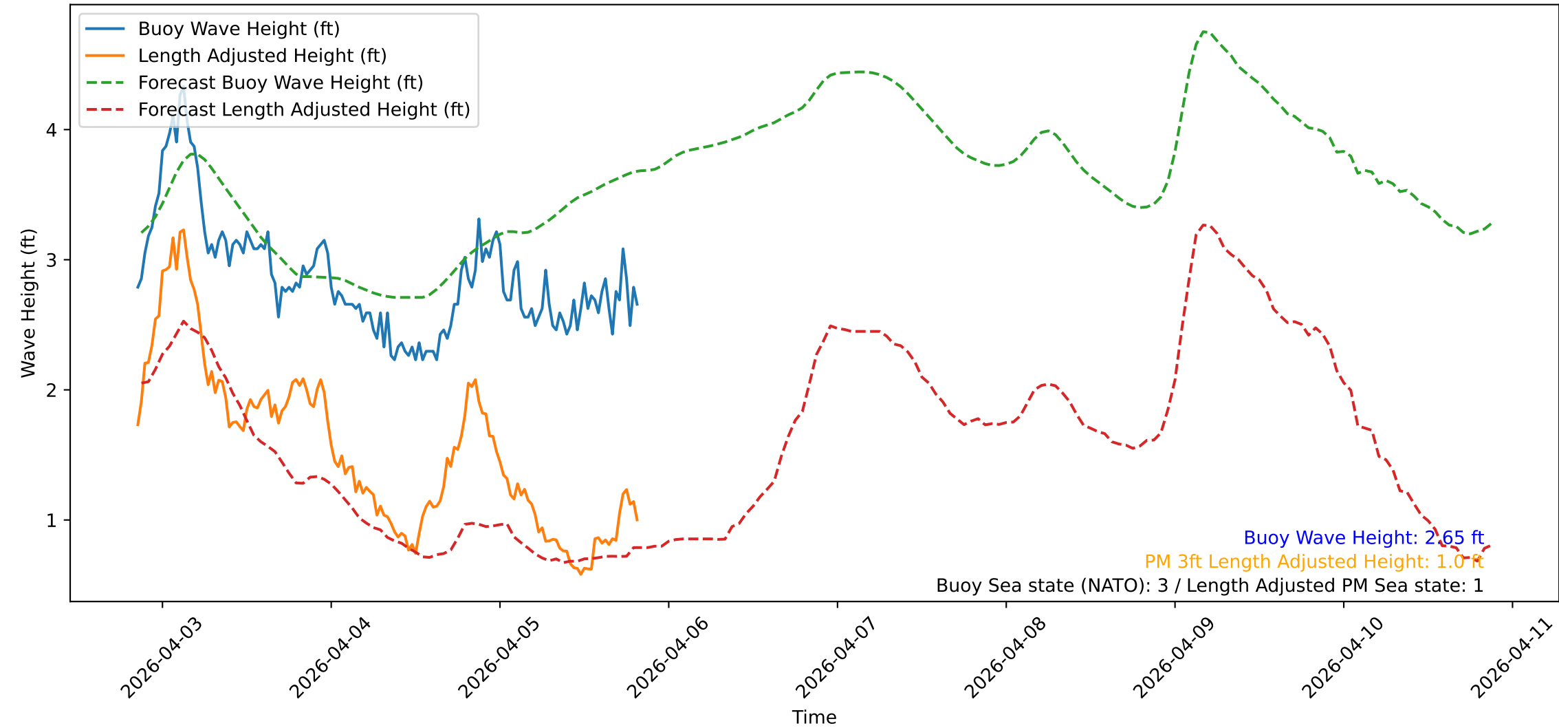
Wave Heights over Time for Green Beach at 2026-04-05 20:31:26
