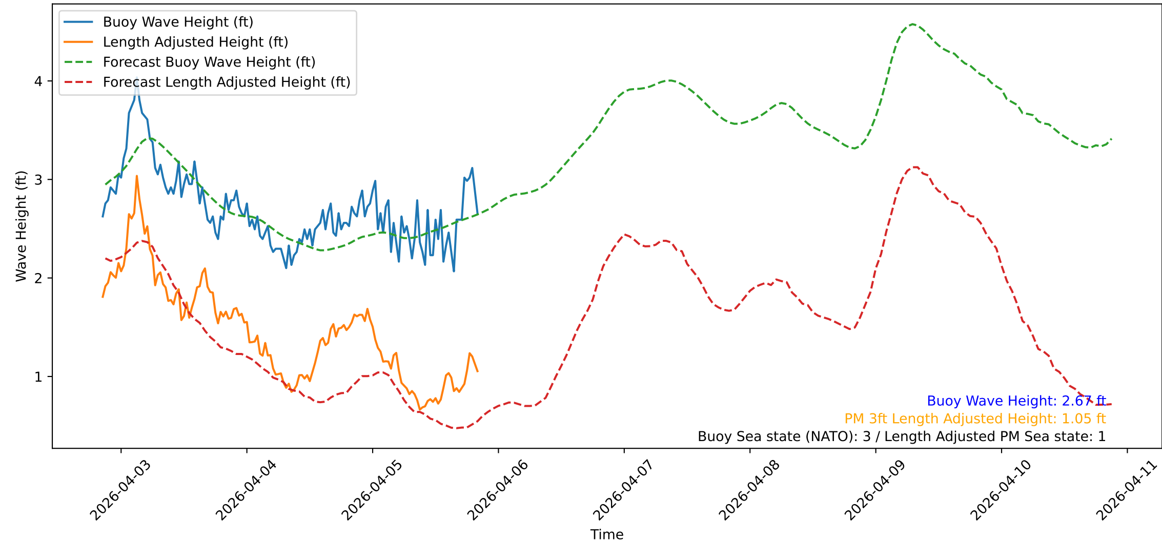
Wave Heights over Time for Oceanside Harbor at 2026-04-05 20:30:38
