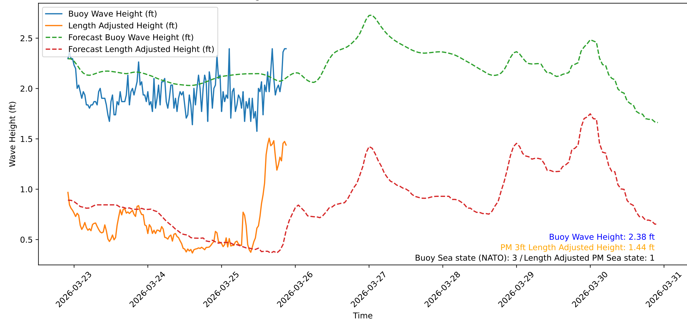
Wave Heights over Time for Red Beach at 2026-03-25 21:50:47
