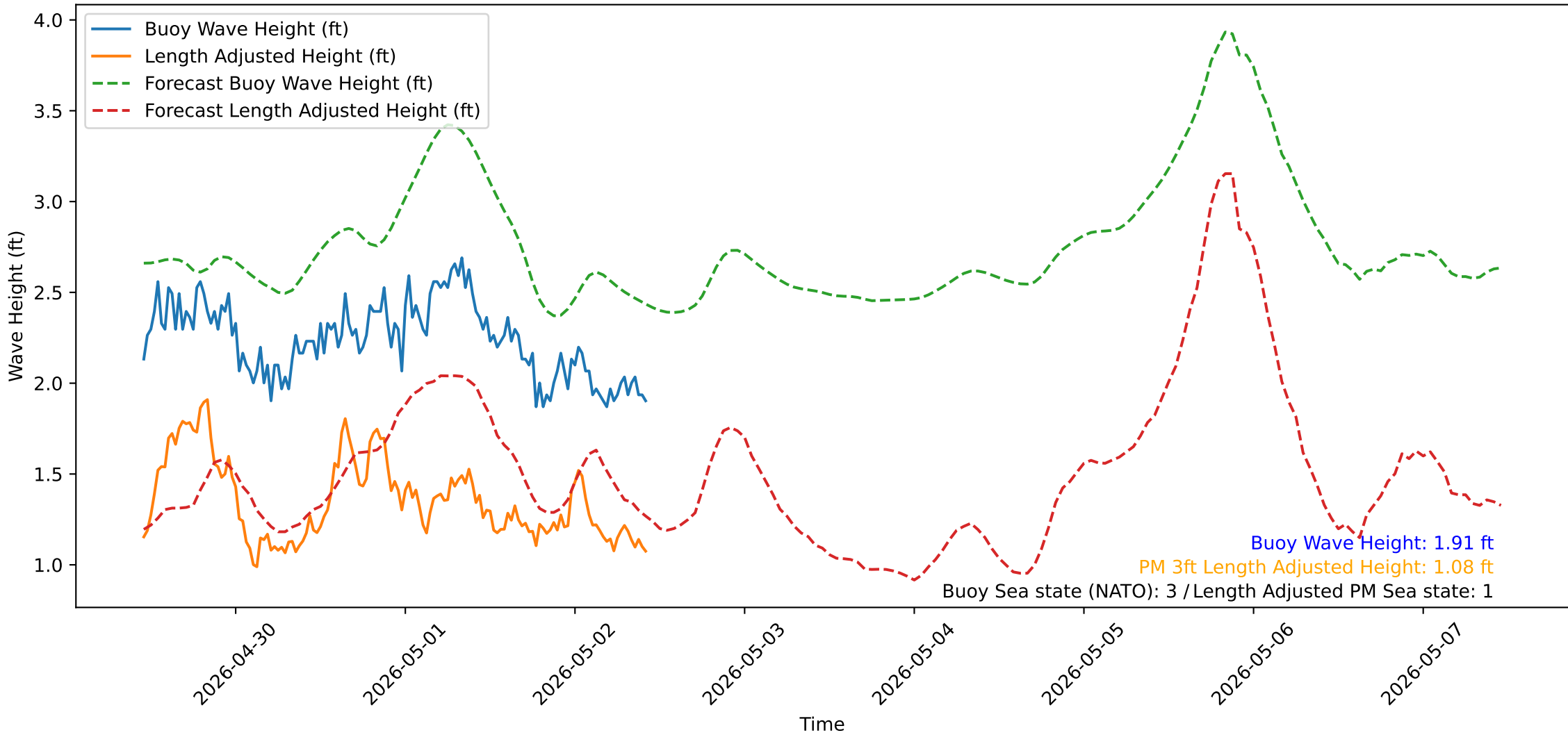
Wave Heights over Time for Oceanside Harbor at 2026-05-02 10:50:31
