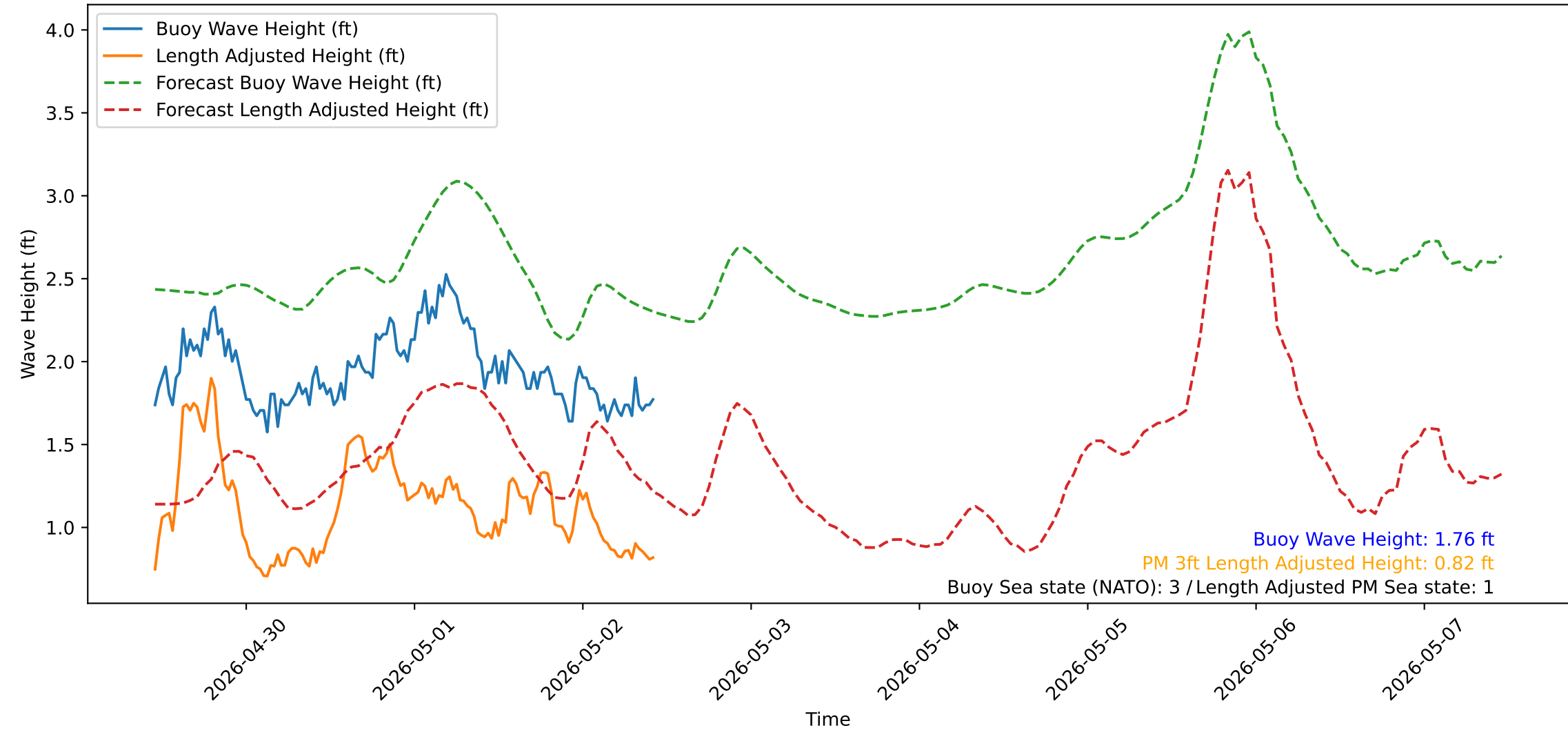
Wave Heights over Time for Red Beach at 2026-05-02 10:50:52
