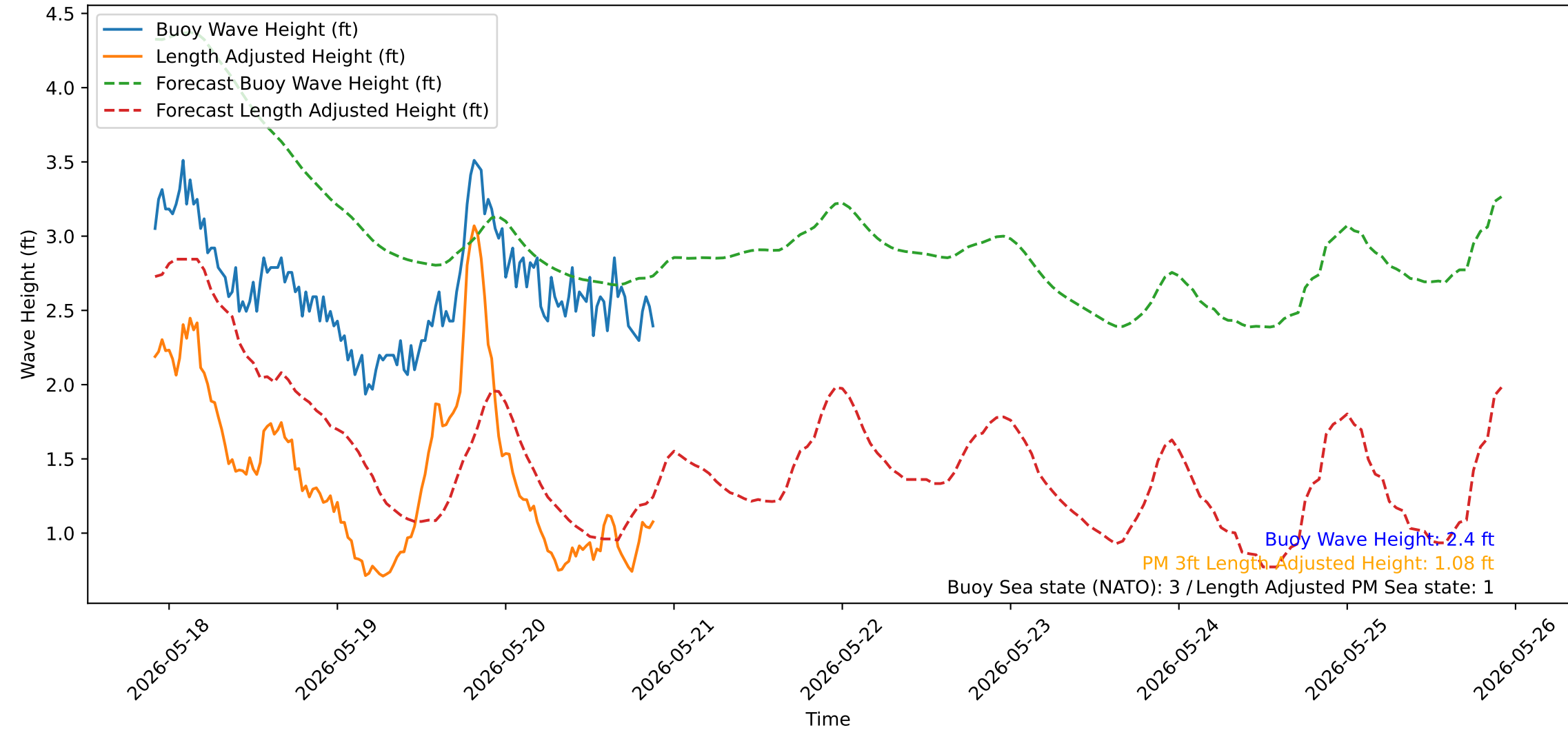
Wave Heights over Time for Red Beach at 2026-05-20 21:50:52
