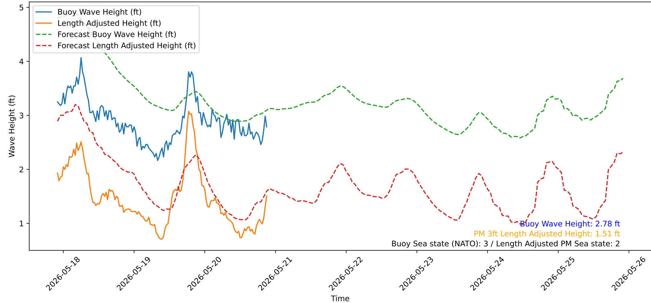
Wave Heights over Time for Green Beach at 2026-05-20 21:51:15
