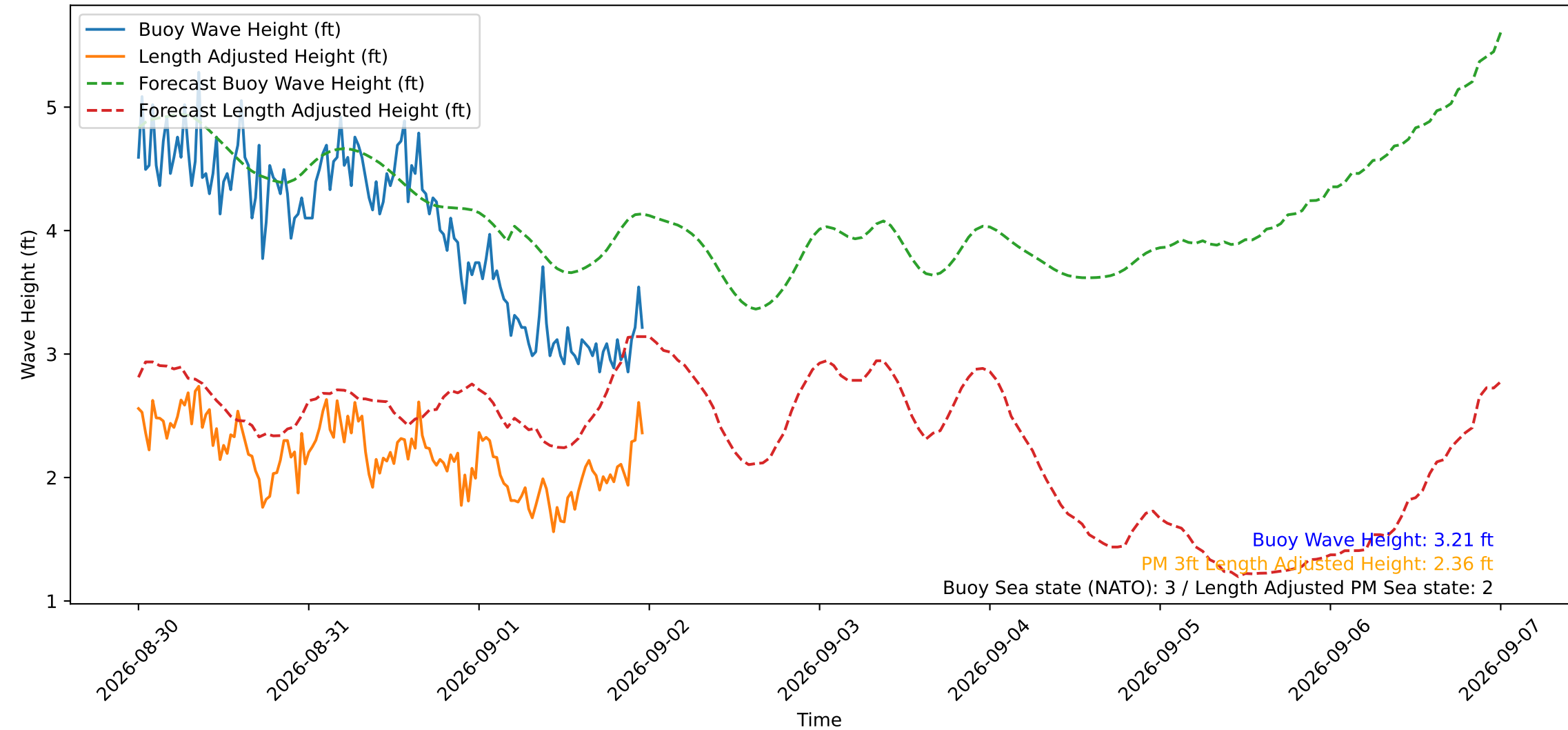
Wave Heights over Time for Oceanside Harbor at 2026-09-02 00:00:30
