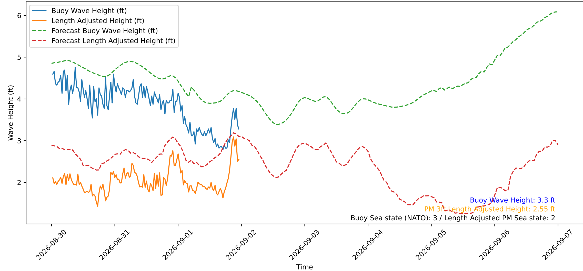
Wave Heights over Time for Green Beach at 2026-09-02 00:01:12
