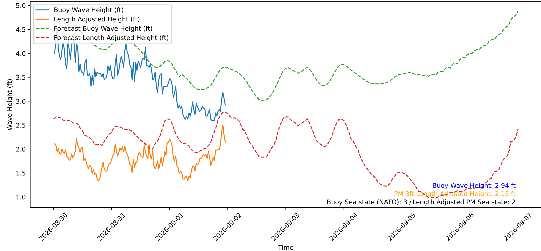
Wave Heights over Time for Red Beach at 2026-09-02 00:00:49
