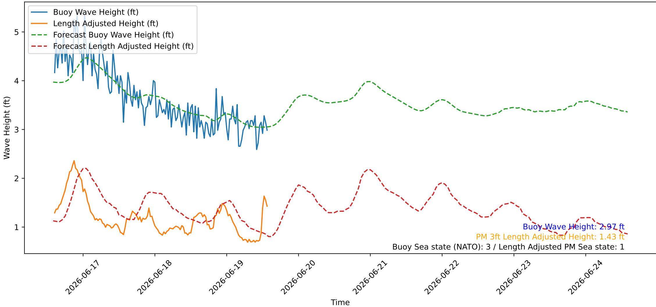
Wave Heights over Time for Red Beach at 2026-06-19 14:10:46
