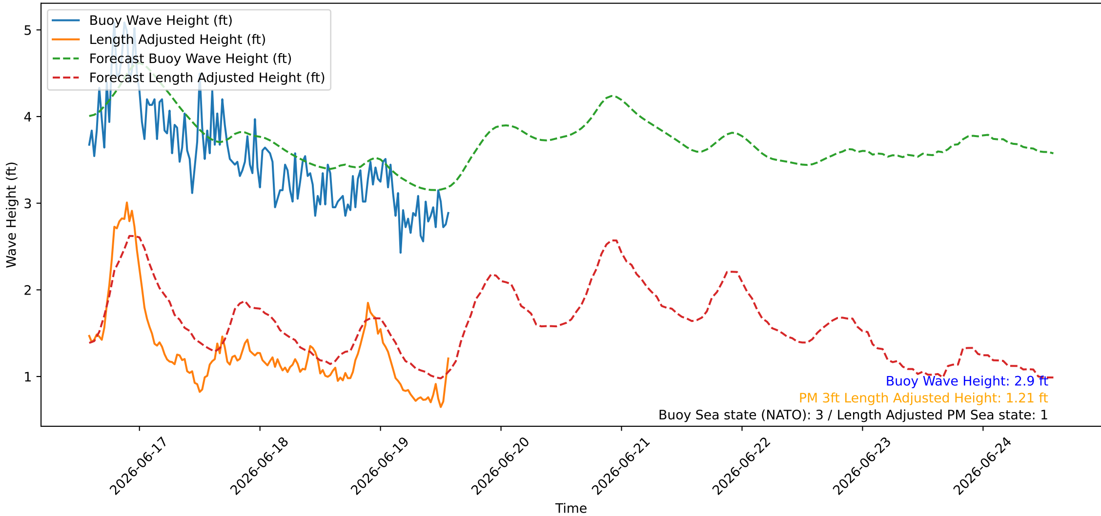
Wave Heights over Time for Green Beach at 2026-06-19 14:11:08
