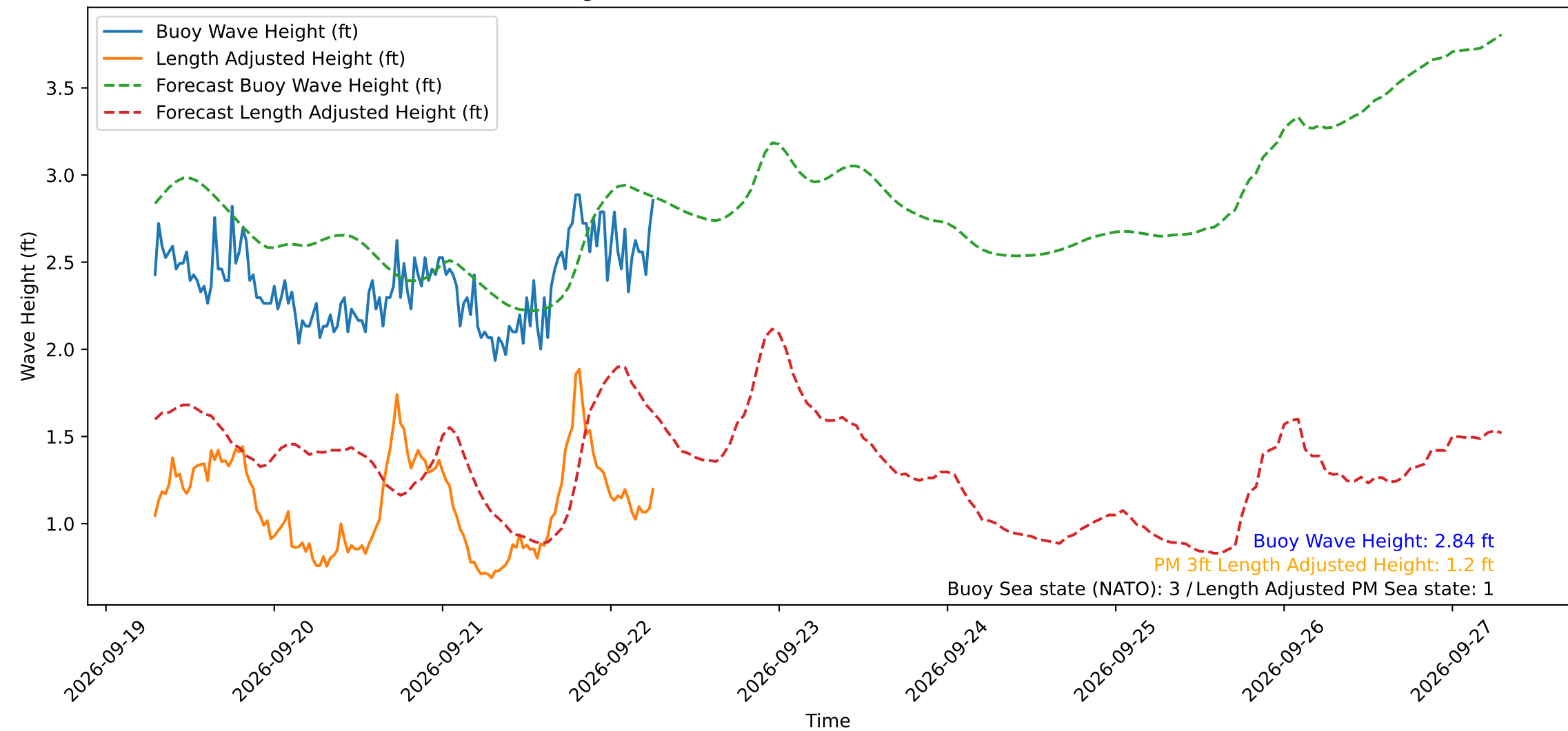
Wave Heights over Time for Red Beach at 2026-09-22 06:40:48
