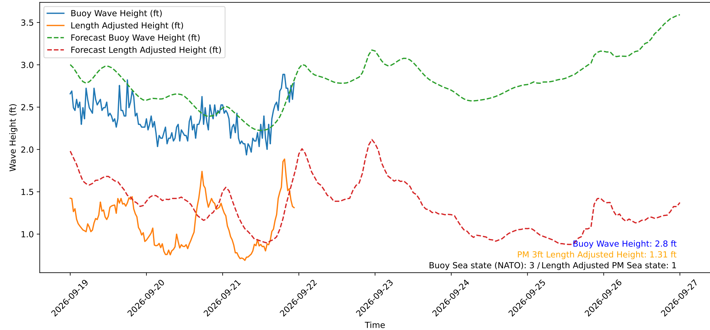
Wave Heights over Time for Red Beach at 2026-09-21 23:30:49
