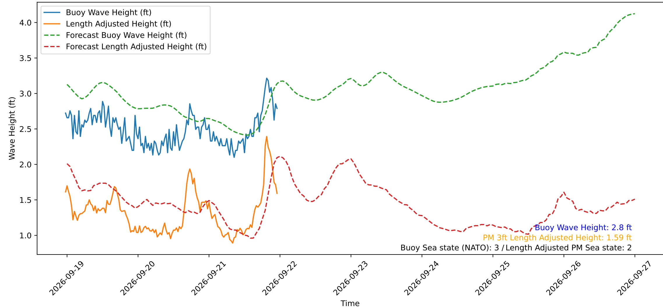
Wave Heights over Time for Oceanside Harbor at 2026-09-21 23:30:29
