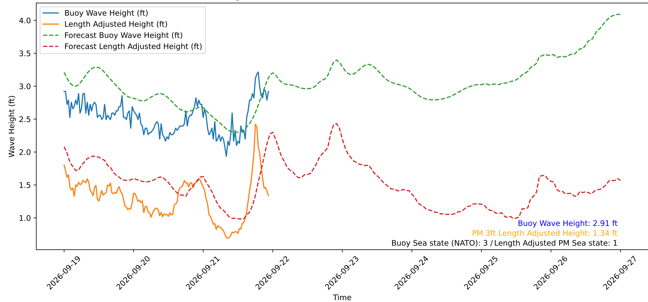
Wave Heights over Time for Green Beach at 2026-09-21 23:31:11
