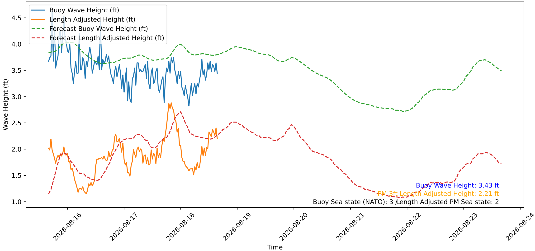
Wave Heights over Time for Oceanside Harbor at 2026-08-18 16:10:26
