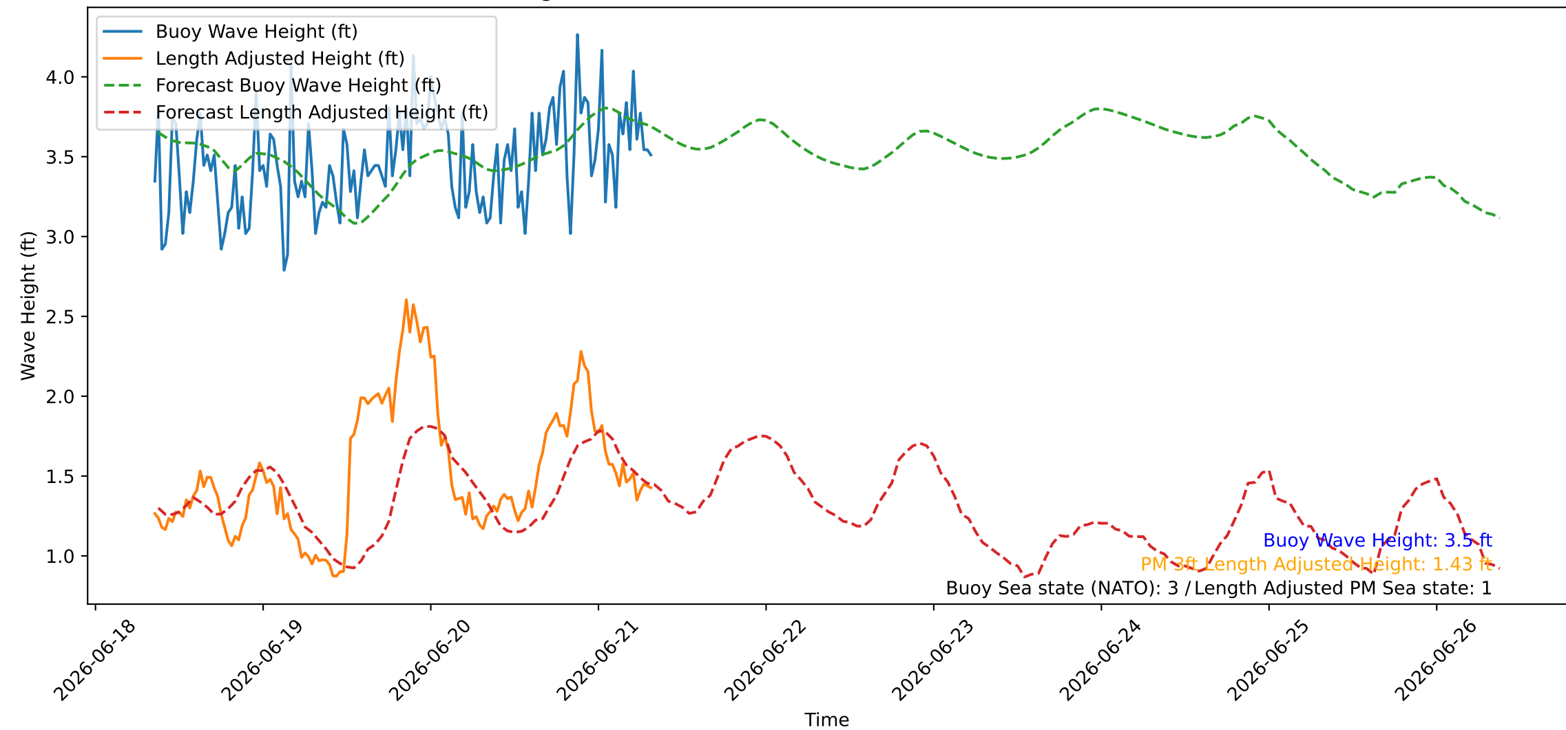
Wave Heights over Time for Oceanside Harbor at 2026-06-21 08:30:26
