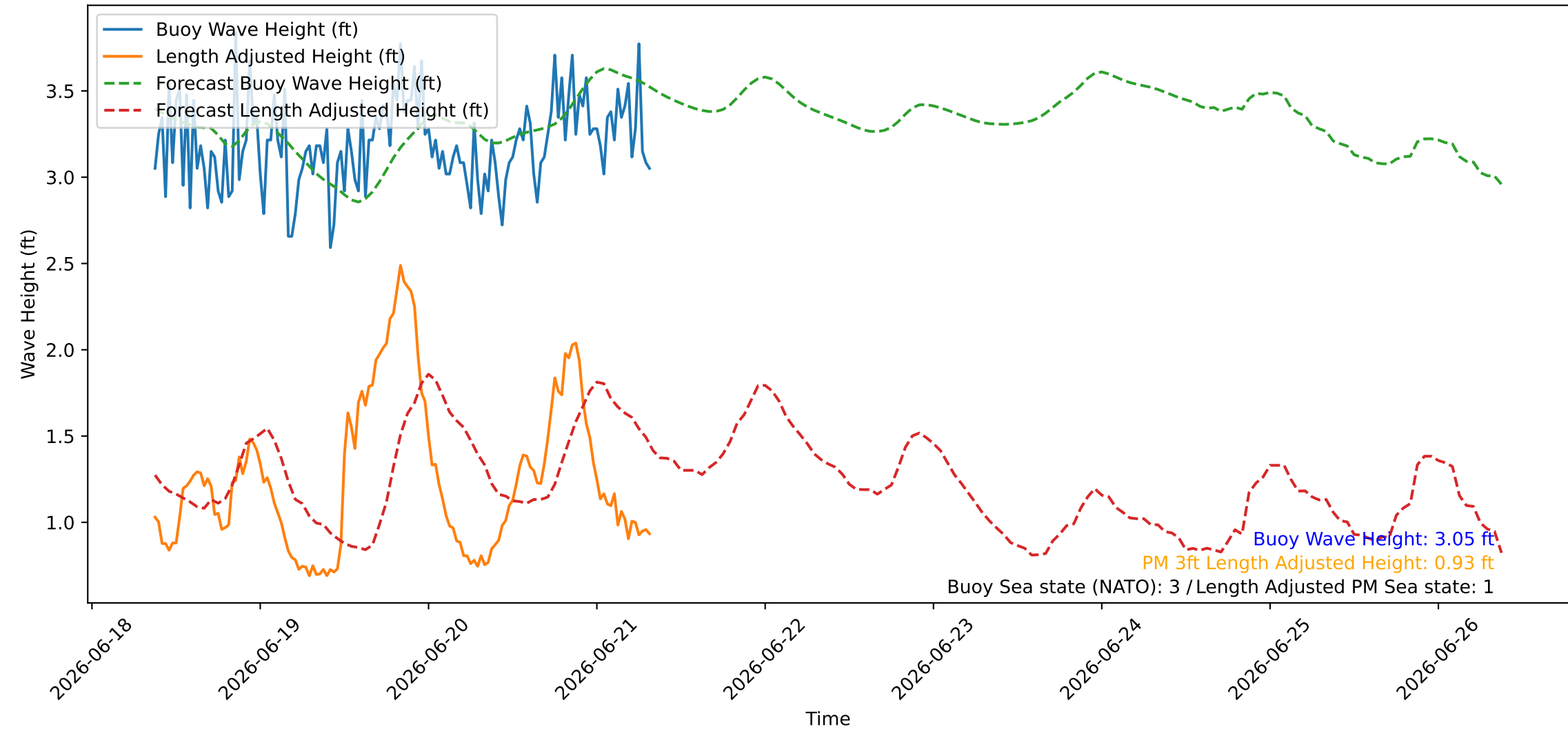
Wave Heights over Time for Red Beach at 2026-06-21 08:30:46
