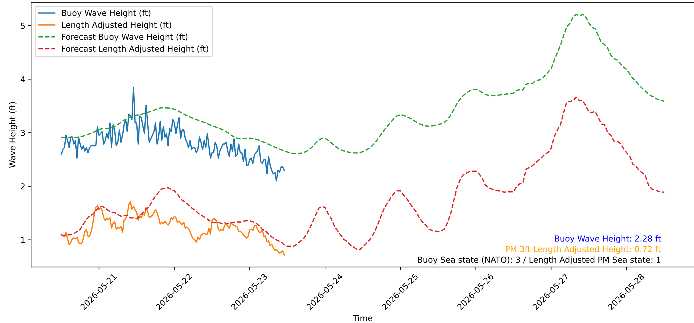
Wave Heights over Time for Oceanside Harbor at 2026-05-23 12:10:31
