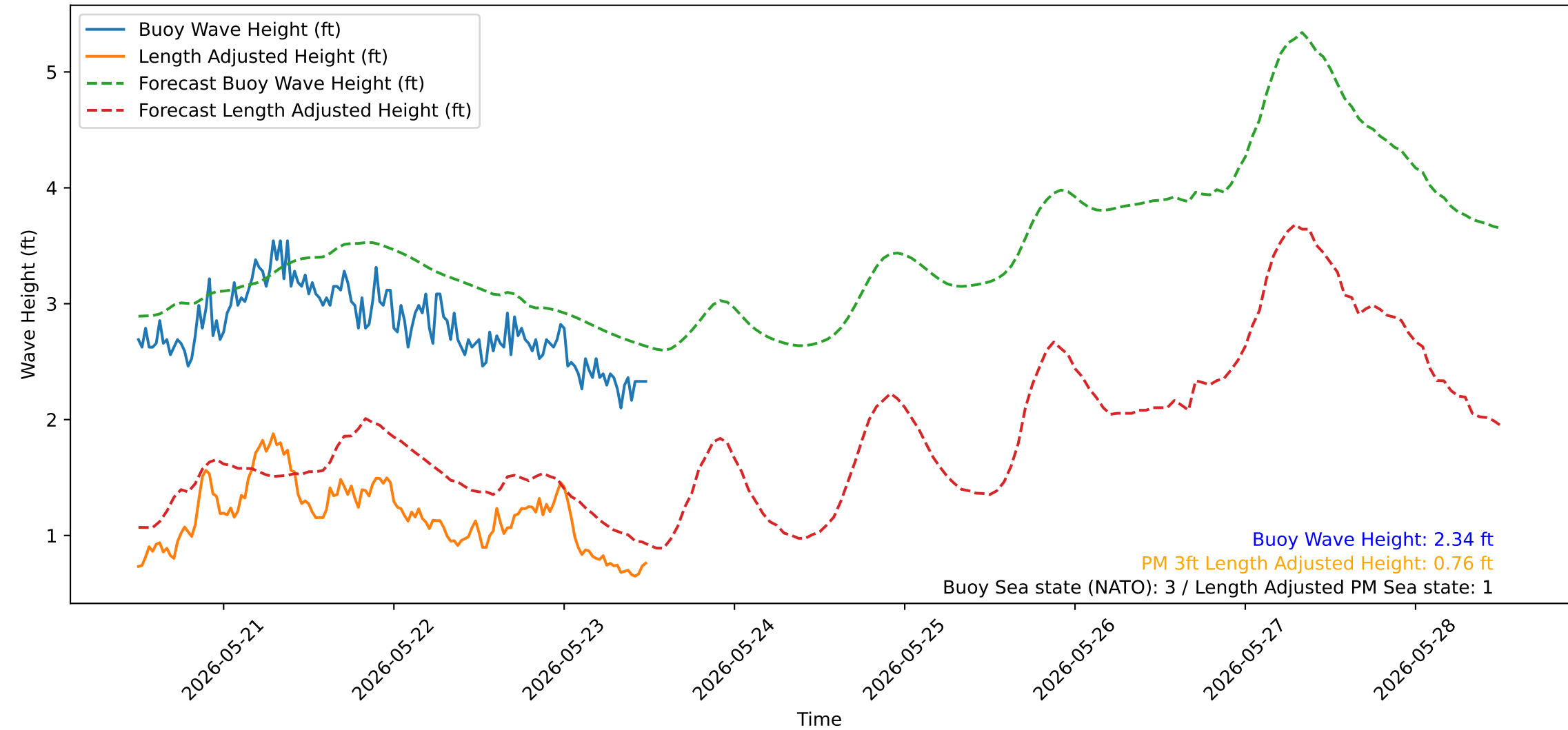
Wave Heights over Time for Green Beach at 2026-05-23 12:11:13
