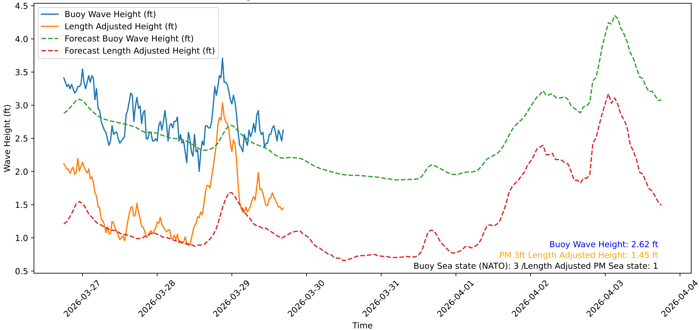
Wave Heights over Time for Green Beach at 2026-03-29 17:51:09
