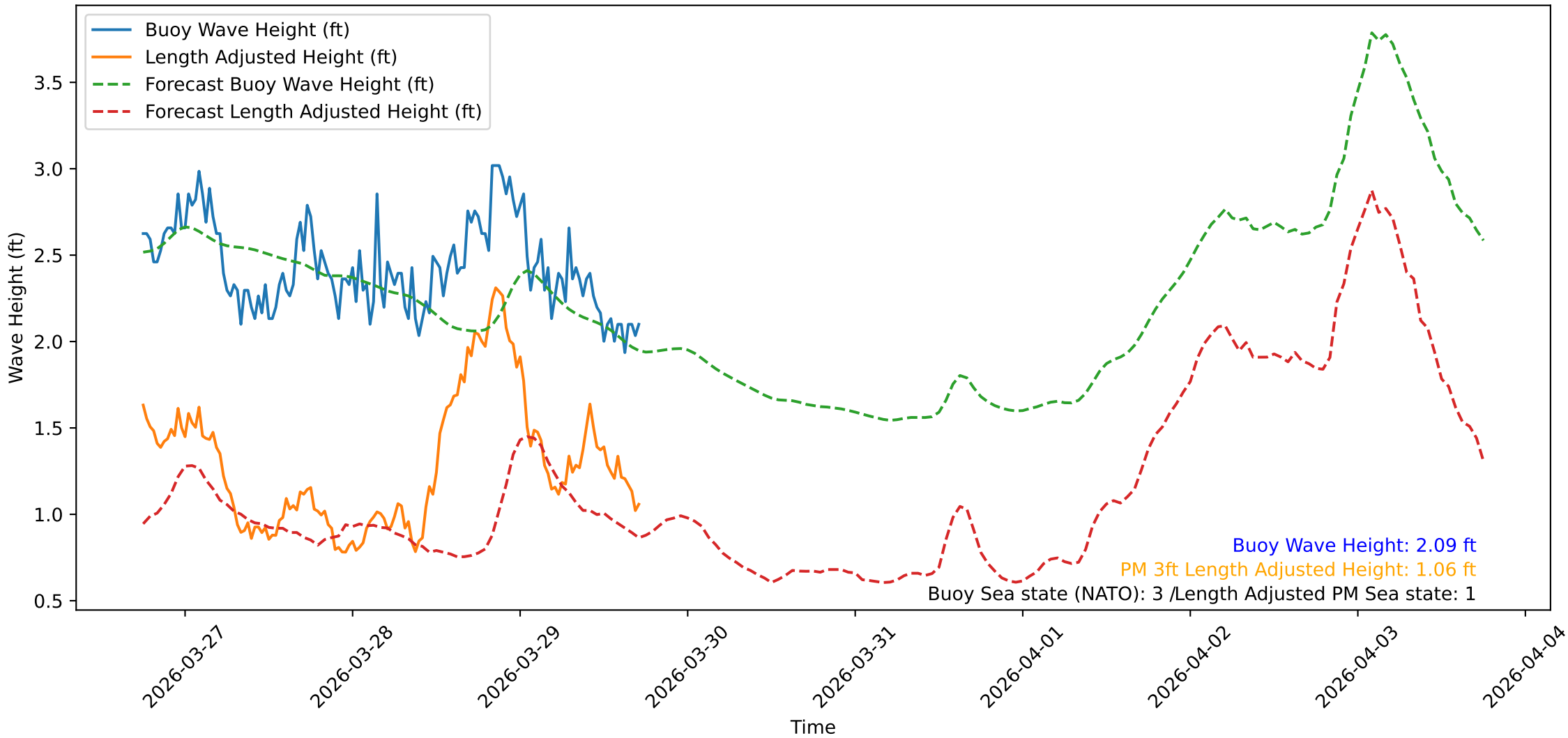
Wave Heights over Time for Red Beach at 2026-03-29 17:50:47
